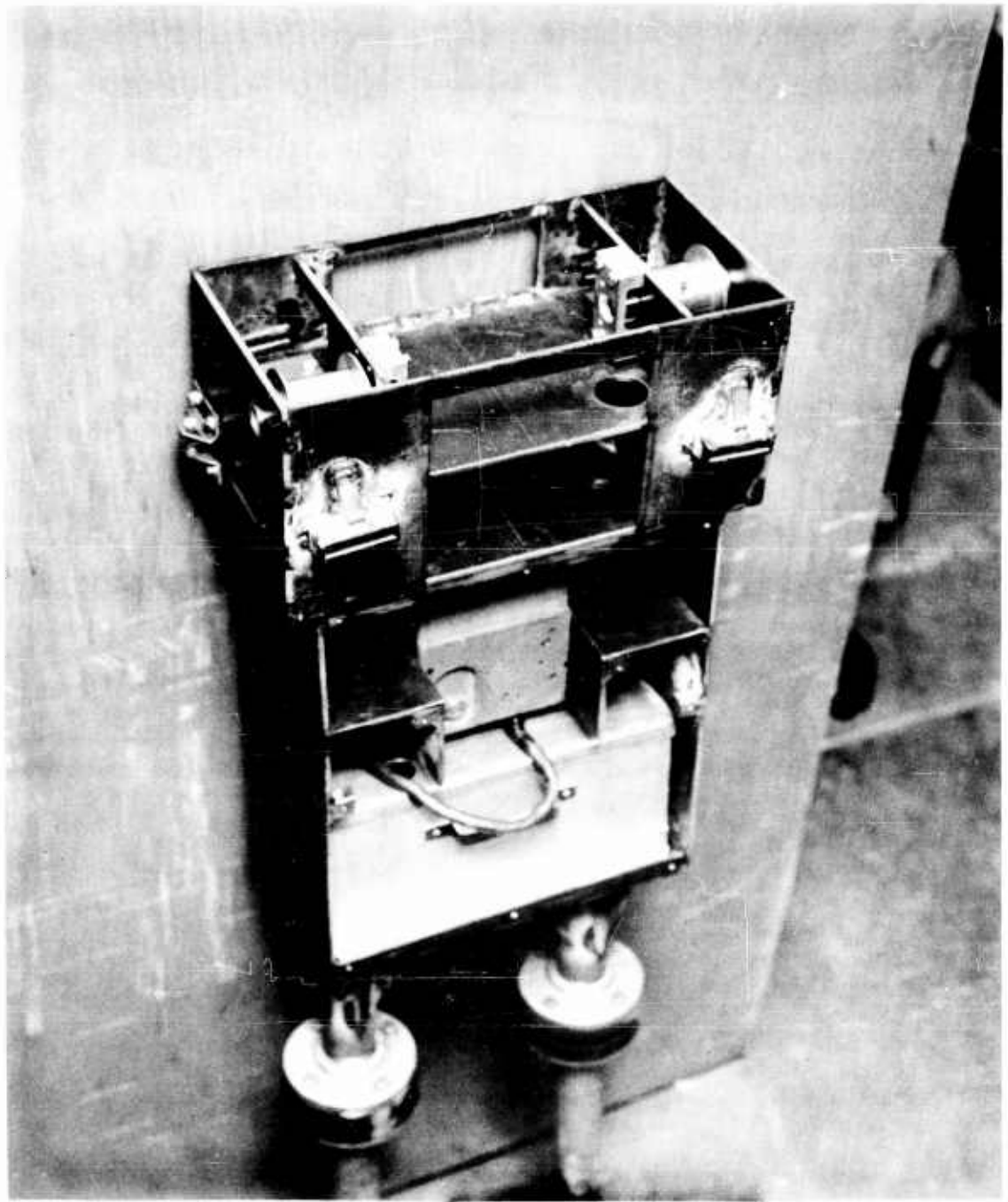
Figure 28 Installation of Upper to Lower Cavities
