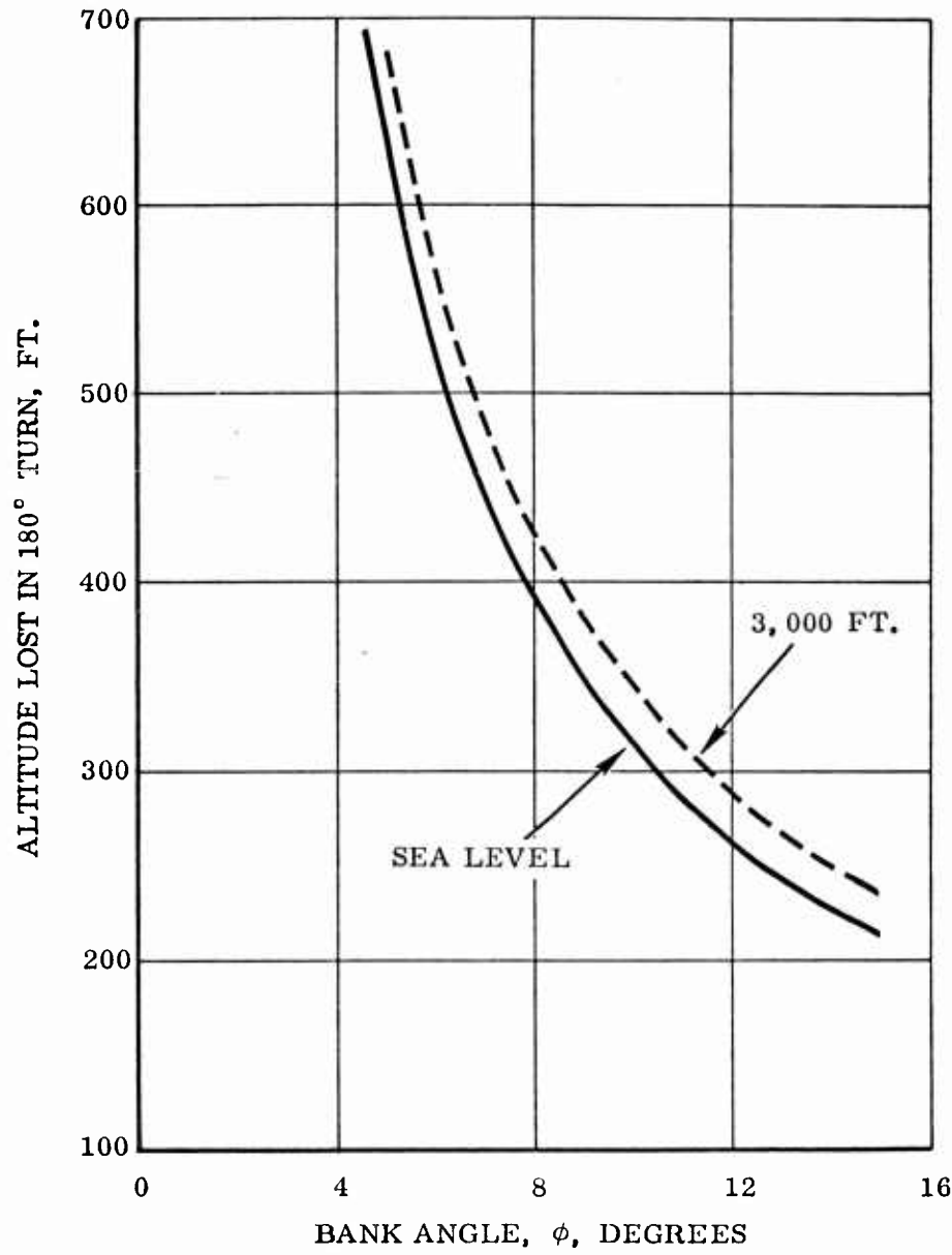
Figure 11 Theoretical Altitude Lost in 180^\circ Turn Versus Bank Angle
