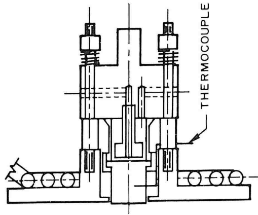
( SECTIONAL VIEW )
