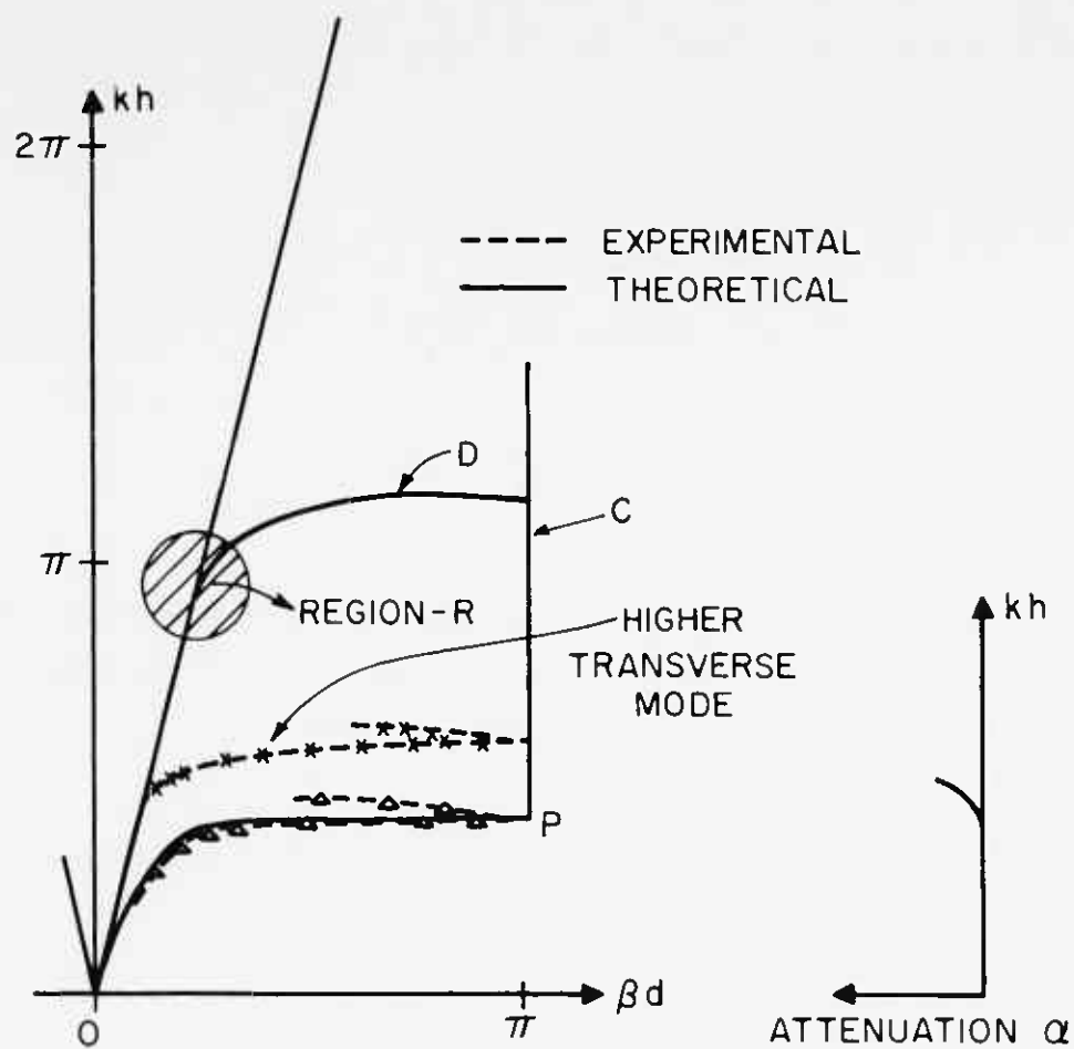
Figure 3a. Theoretical and Experimental k - \beta Diagram of Uniform Corrugated Surface
