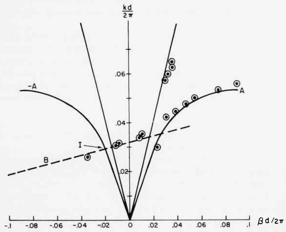
Figure 7. K - \beta Diagram of Uniform Corrugated Surface with Multiple Loop Feed
