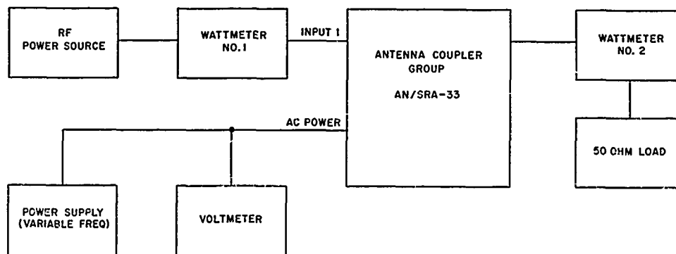
Figure 2-3. Test Circuit for Test No. 3
