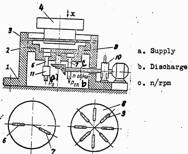
Figure 4 Basic diagram of vibration stand with diaphragm hydroservomotor.
