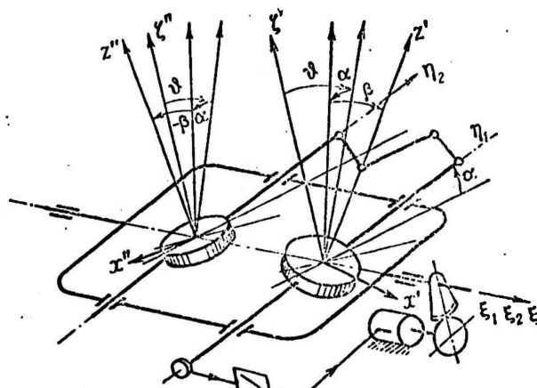
Figure 1 Schematic drawing of the gyro-frame
