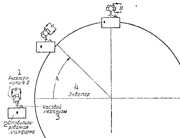
Fig. 103. Change in the mutual position of the accelerometer platform with respect to the gyrostabilized platform during missile flight along a meridian, as a result of the functioning of the system through the latitude channel. 1) Accelerometer N-S; 2) stabilized platform; 3) clockwork mechanism; 4) equator.
