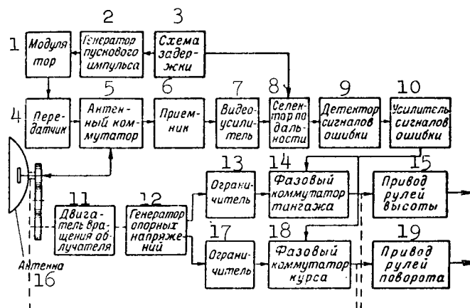
Fig. 58. Block diagram of active (radar) homing system. 1) Modulator; 2) trigger pulse generator; 3) delay circuit; 4) transmitter; 5) antenna switch; 6) receiver; 7) video-amplifier; 8) range selector; 9) error-signal detector; 10) error-signal amplifier; 11) motor by means of which the primary radiating element is set into motion; 12) reference voltage generator; 13) limiter; 14) pitch phase commutator; 15) elevator drive; 16) antenna; 17) limiter; 18) heading phase commutator; 19) rudder drive.
