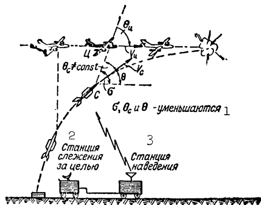
Fig. 46. Technique for proportional homing of guided missile. 1) \sigma , \theta and \theta diminishing; 2) target-tracking station; 3) guidance station.
