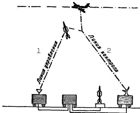
Fig. 39. Communications lines in remote-control systems (non-autonomous systems). 1) Control link; 2) telemetry link.
