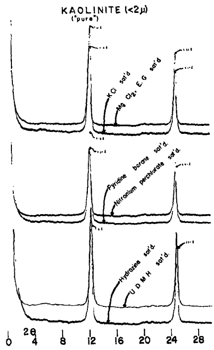
Figure 10. X-ray diffraction patterns for "pure" Kaolinite.
