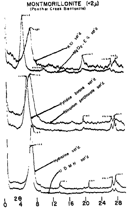
Figure 11. X-ray diffraction patterns for "pure" Montmorillonite.
