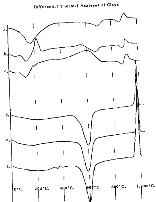
Figure 16. The differential thermal analyses of saturated montmorillonite and kaolinite clays.
