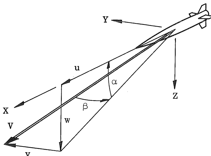
Fig. 5 Velocity Components and Aerodynamic Angles
