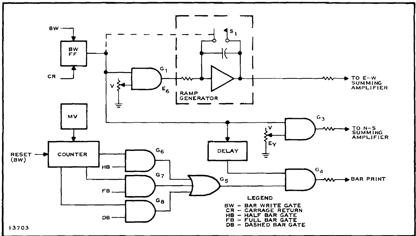
Figure 18. Bar Generator and Print Gate Block Diagram
