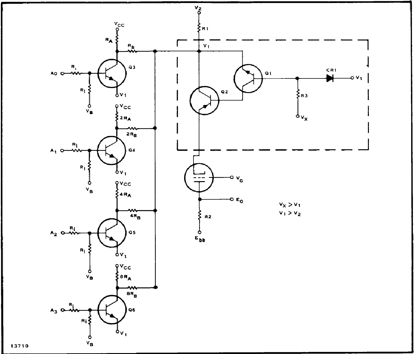
Figure 23. One Half of D/A Converter Partial Schematic Diagram
