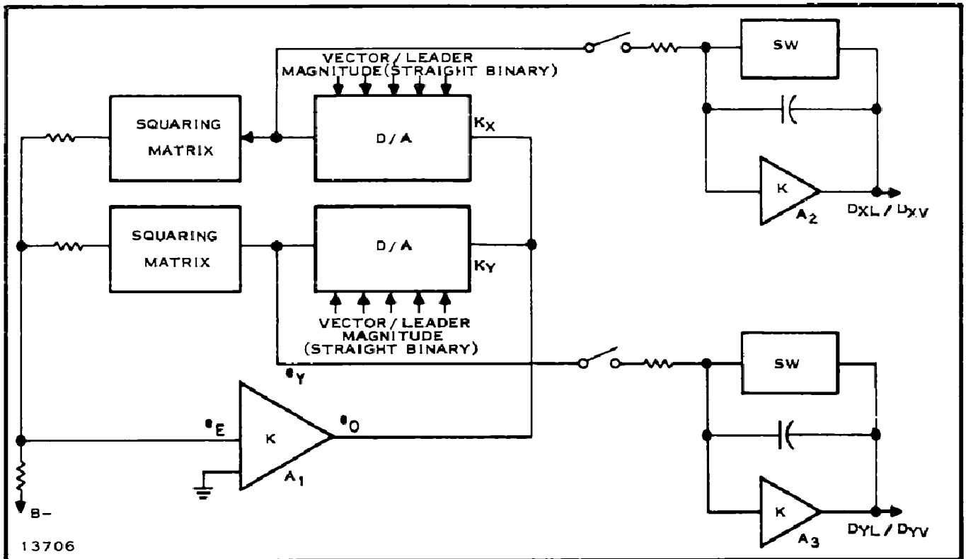
Figure 17. Vector/Leader Generator Functional Block Diagram
