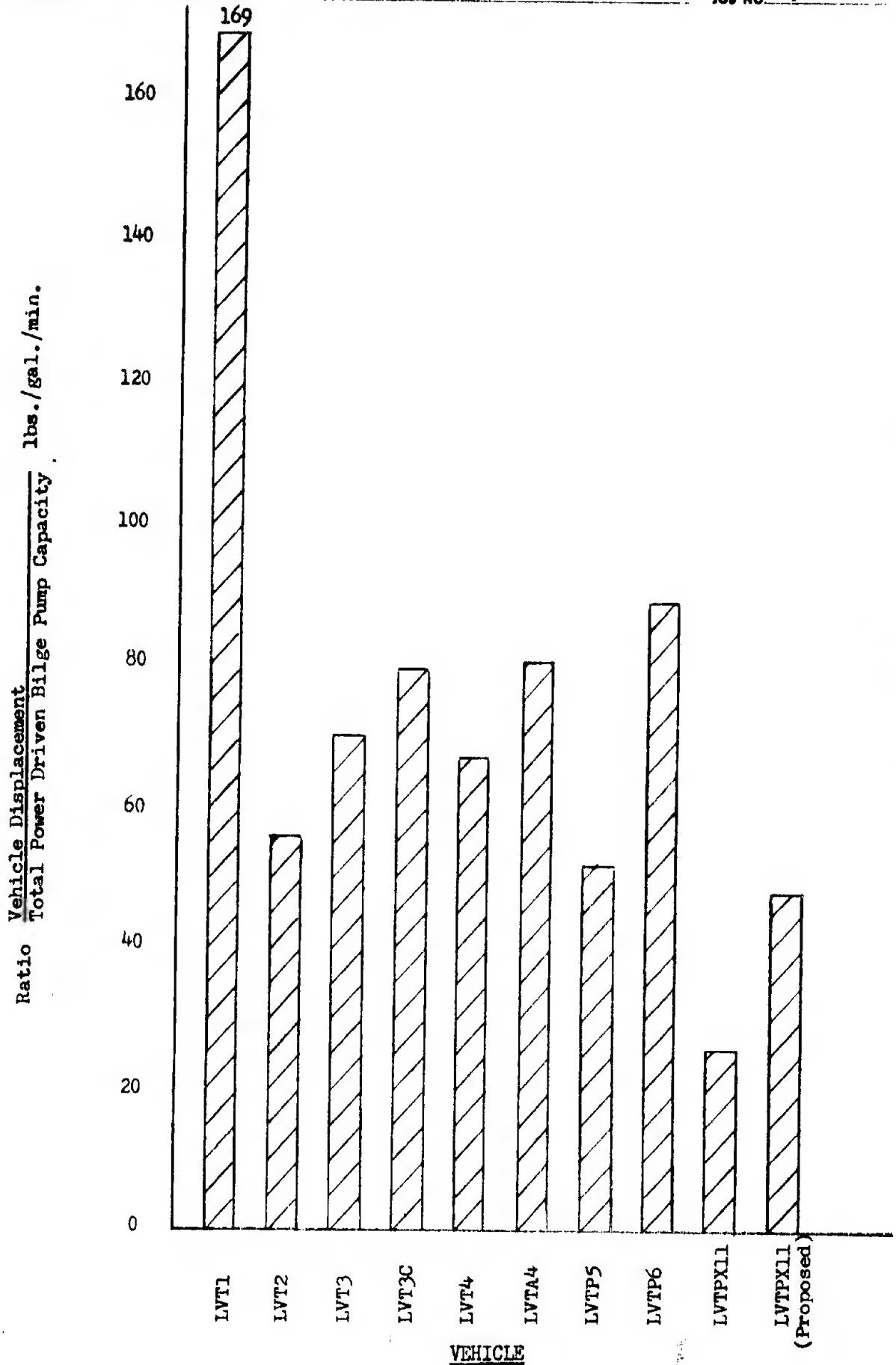
Figure 8-1 BILGE SYSTEM COMPARATIVE STUDY
