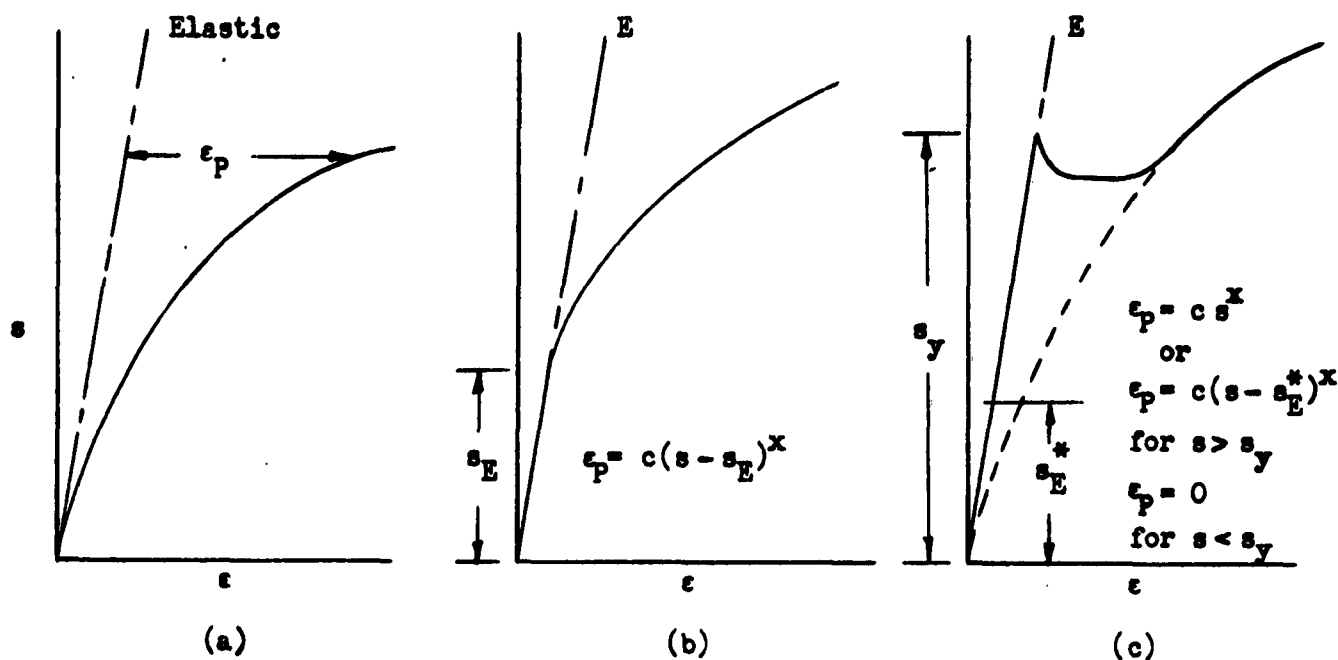
Fig. 9 Different Ways of Interpreting the Endurance Limit
