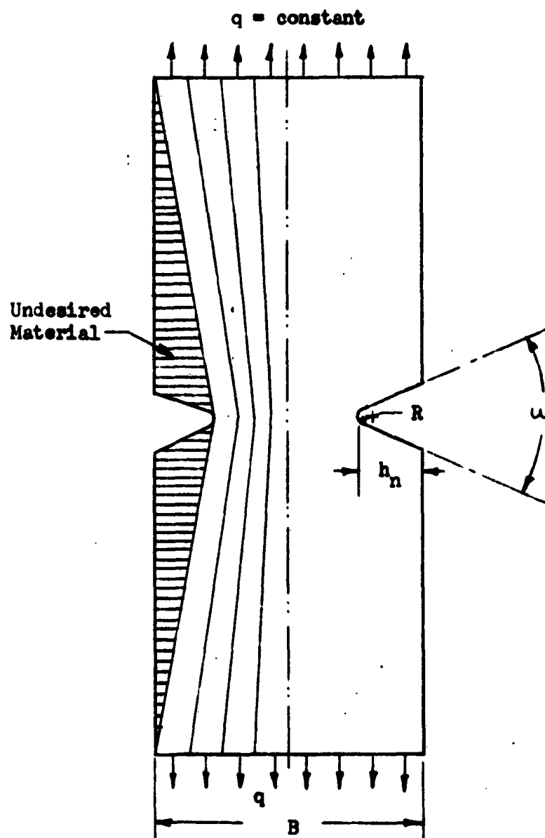
Fig. 22 Effect of a Notch
