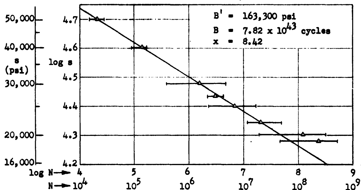
Fig. 7 Log-Log Plot of Fig. 6
