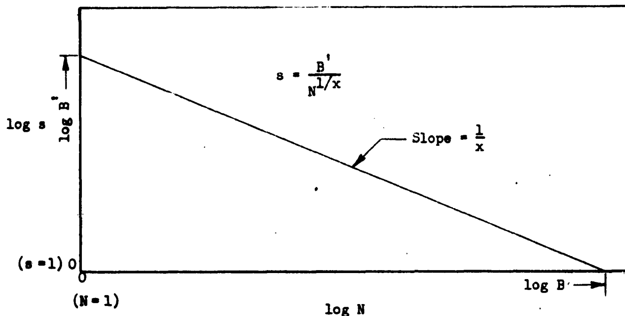
Fig. 5 Logarithmic Plot of s - N Equation
