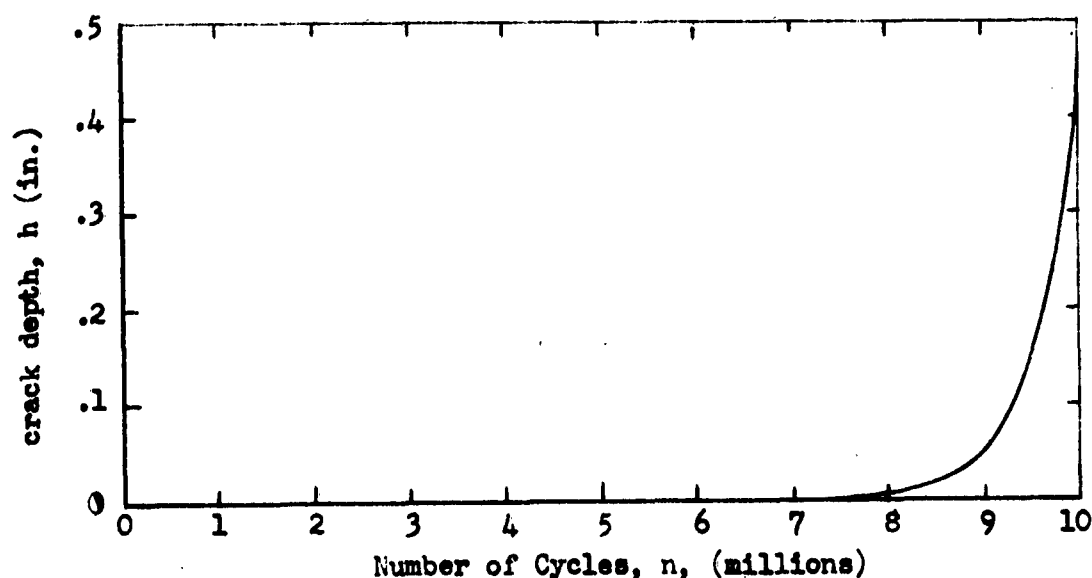
Fig. 3 Diagrammatic Representation of Crack Growth
