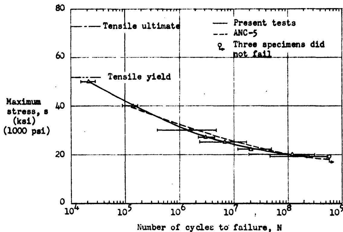
Fig. 6 s - N Curves for Tests of 24S-T4 Rotating-Beam Specimens (From NACA TN-2798)
