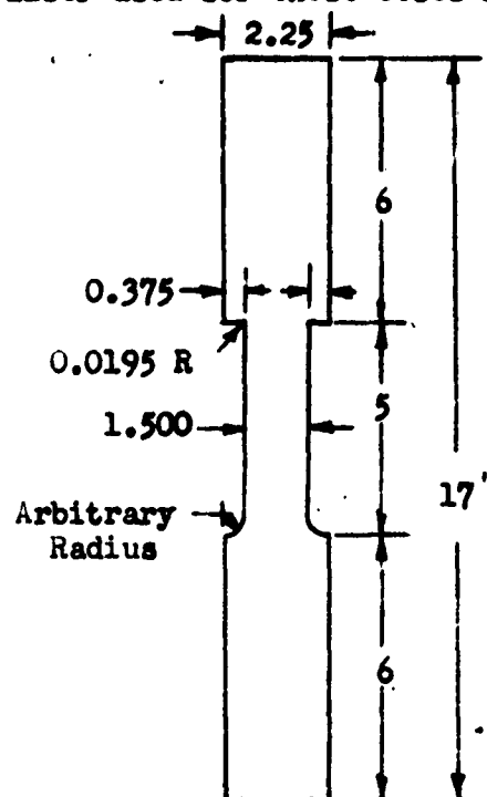
Fig. 24 Notched Fatigue Test Specimen with K_t = 4.0 (From NACA TN 2389, Fig. 2)
