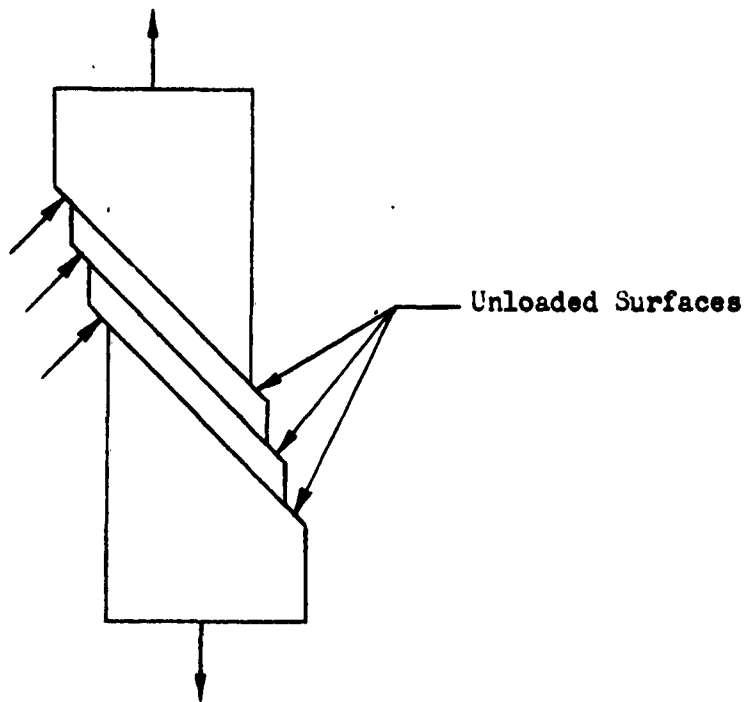
Fig. 1 - Separation Failures During Slip
