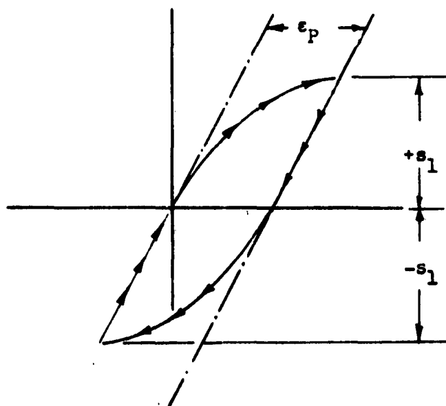
Fig. 15 Stress-Strain Loop for Balanced Cyclic Loading.
