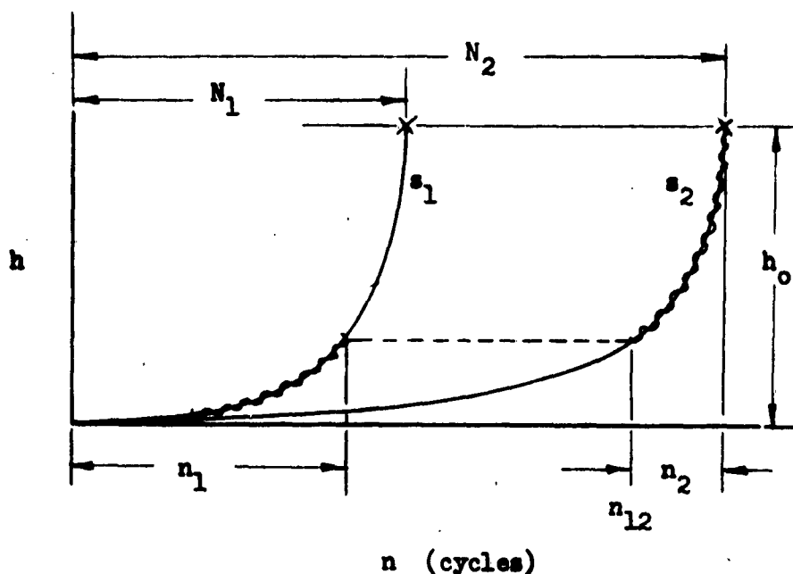
Fig. 13 "Overstressing", in Terms of Crack Growth
