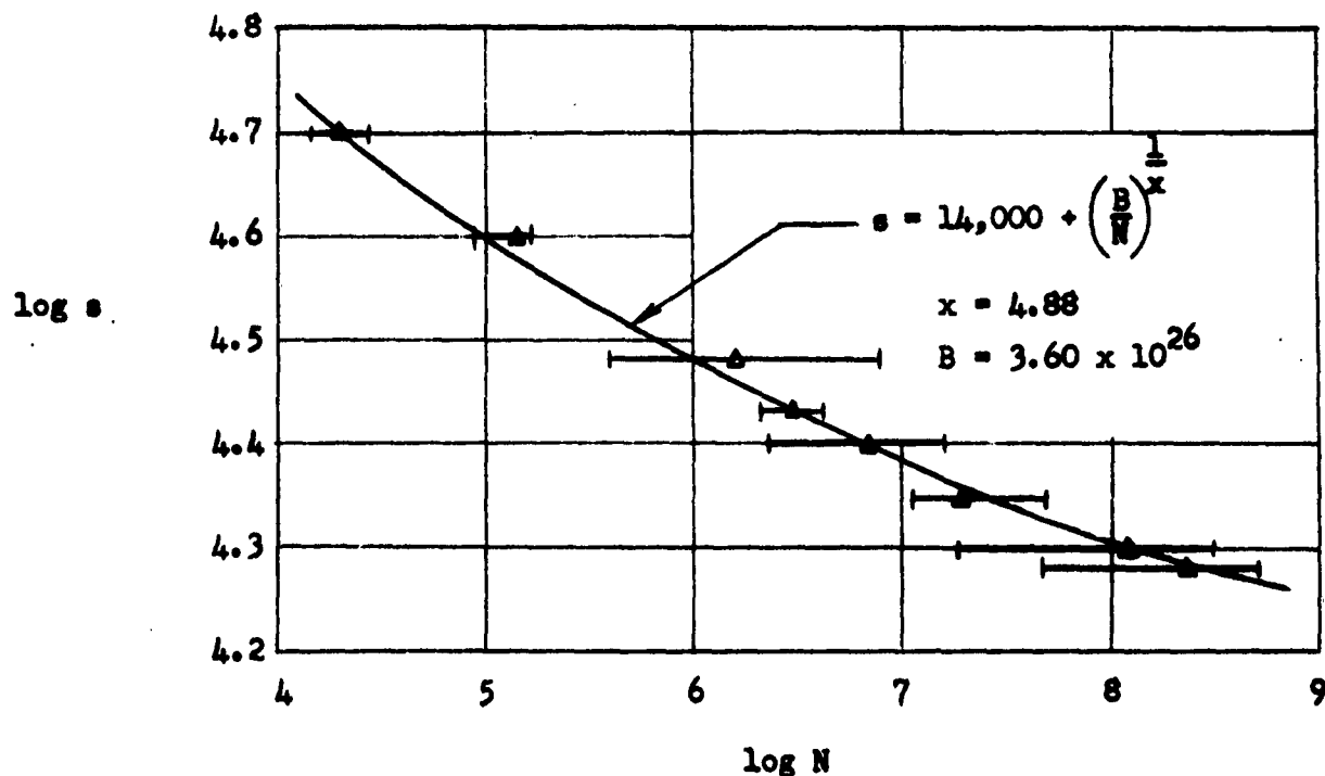
Fig. 10 - Effect of An Elastic Limit (Test Data from NACA TN-2798)
