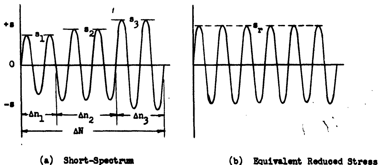
Fig. 11 Variable Stress Amplitudes Represented by a Spectrum
