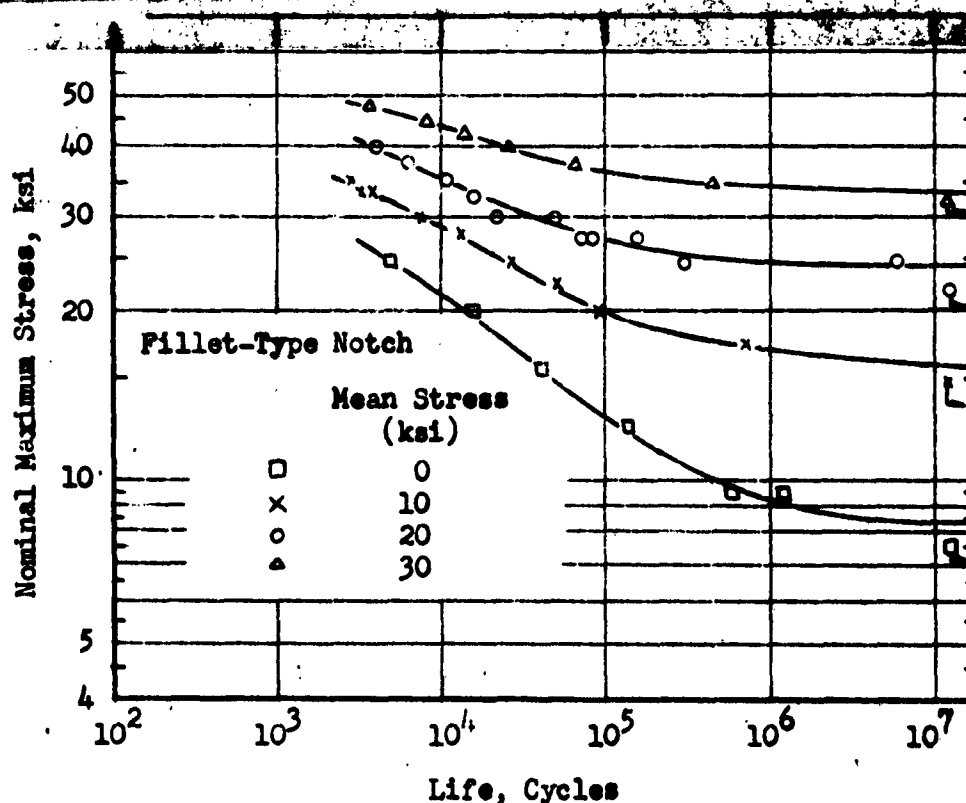
Fig. 23 Results of Axial-Load Fatigue Tests on Notched 24S-T3 Aluminum Sheet Specimens - K_t = 4.0 (From NACA TN 2389, Fig. 6)
