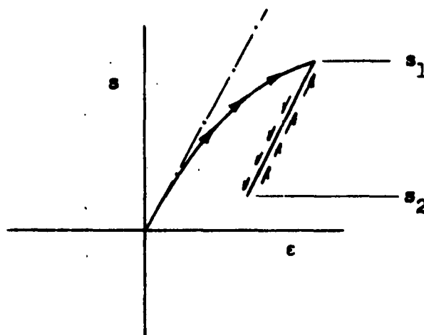
Fig. 16 Unbalanced Cyclic Loading
