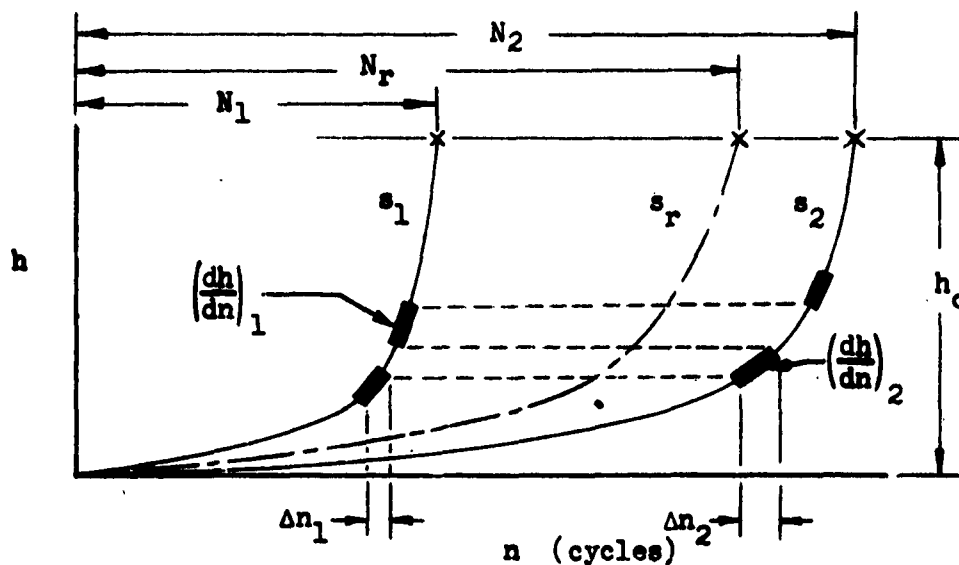
Fig. 12 Crack Growth for a Stress Spectrum Consisting of Two Different Amplitudes
