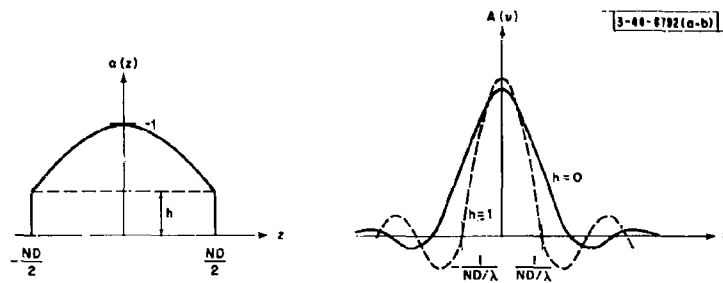
(a) Envelope of cosine-on-a-pedestal amplitude taper.
