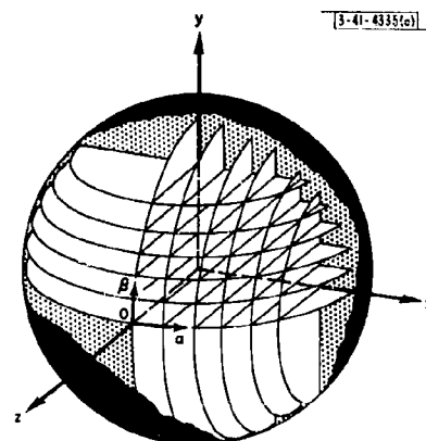
Fig. 31. Beam-steering contours for planar arrays lying in the x-y plane.
