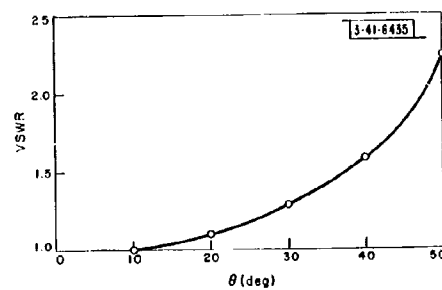
Fig. 61. Minimum VSWR obtainable with linearly polarized, lossless radiators when scanning to an angle \theta_{\max} in both principal planes of an array.
