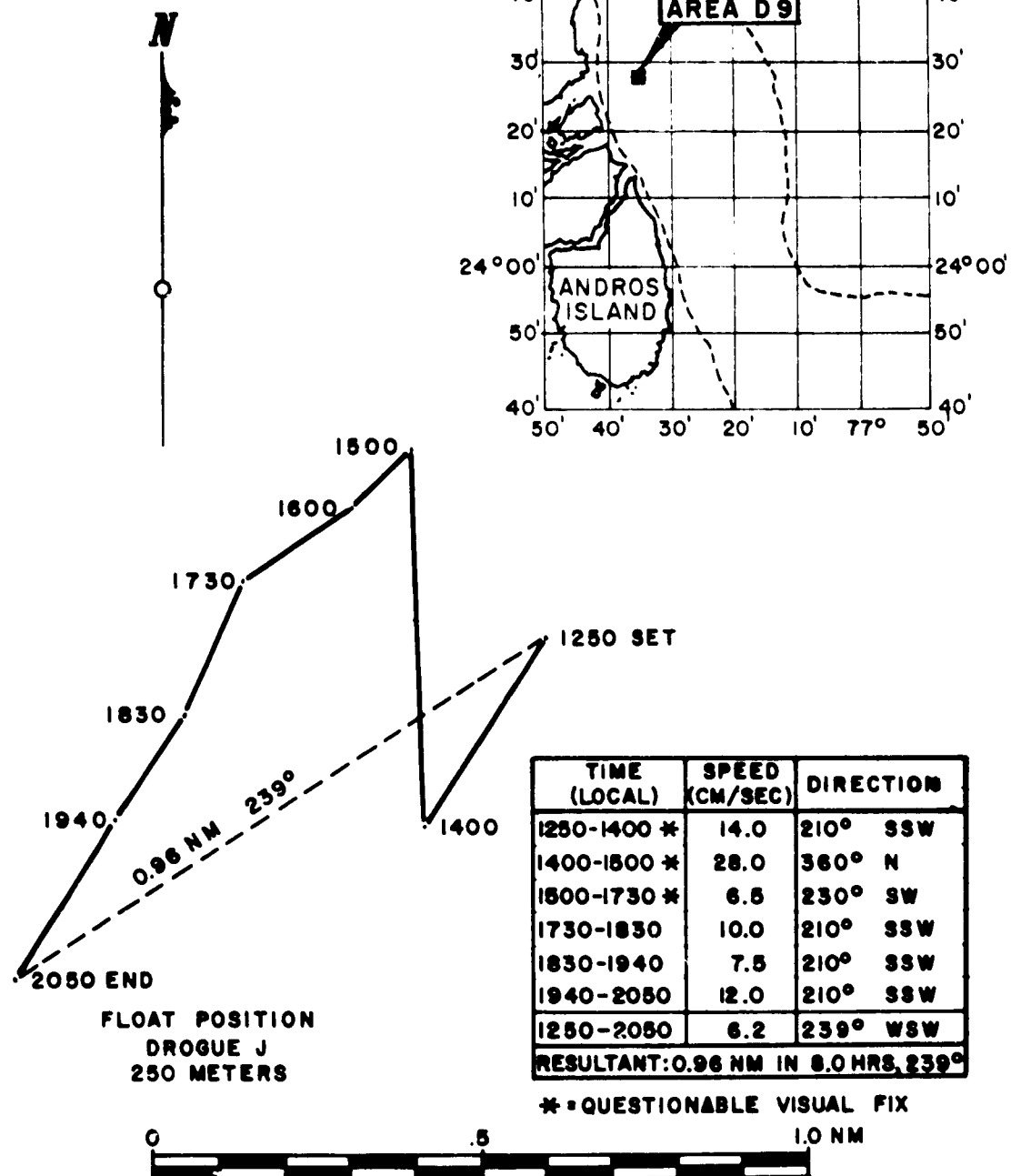
Drogue Current Observations - Area D9 - Depth 250 Meters - Drogue J
