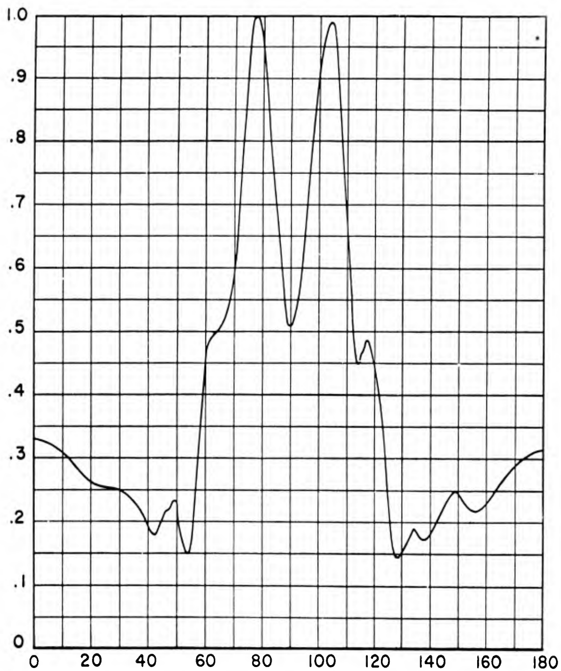
Fig. 10 Measured Vertical Pattern One Wavelength per Turn Scale Model
