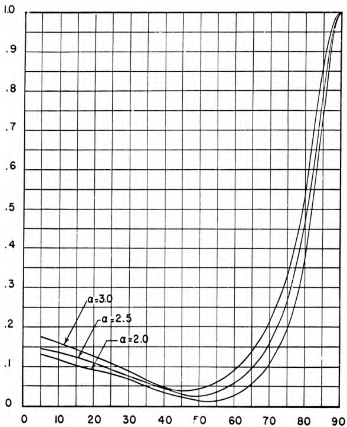
Fig. II Vertical Patterns (Computed) F = 750 Mc. \phi = 0^\circ
