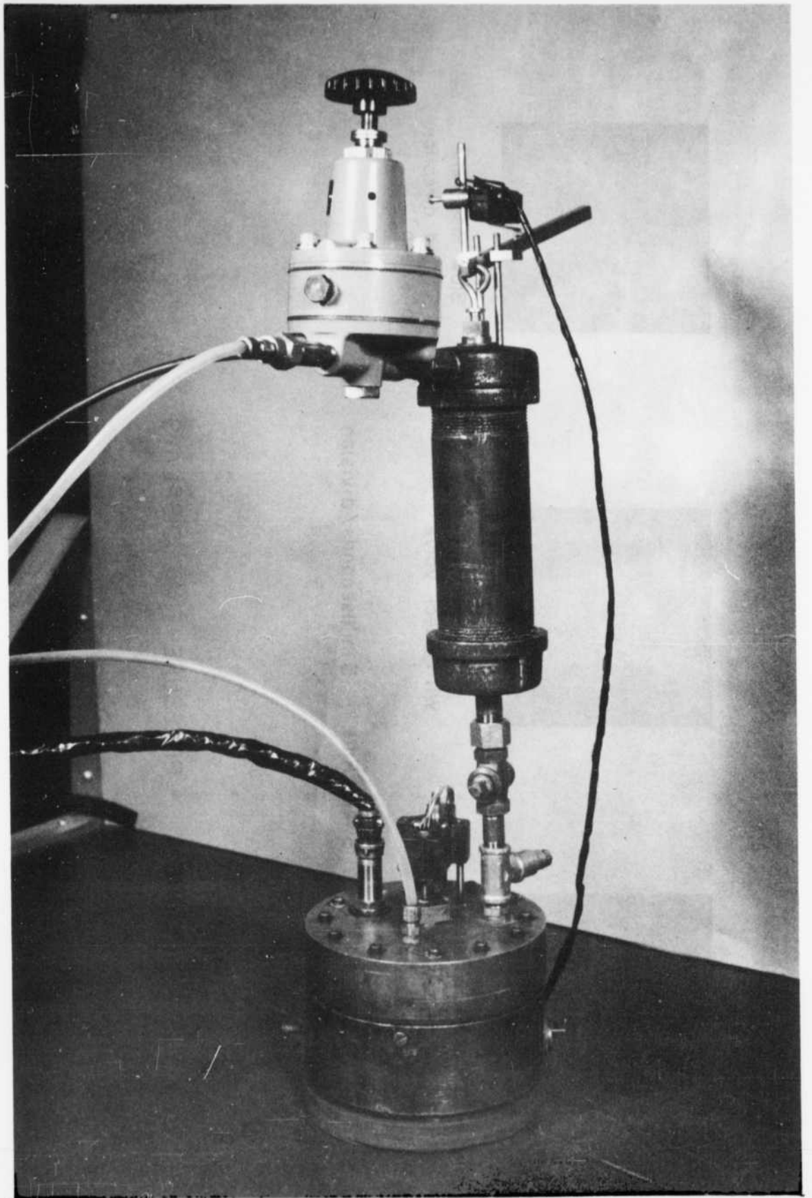
FIGURE 3 OEDOMETER II
