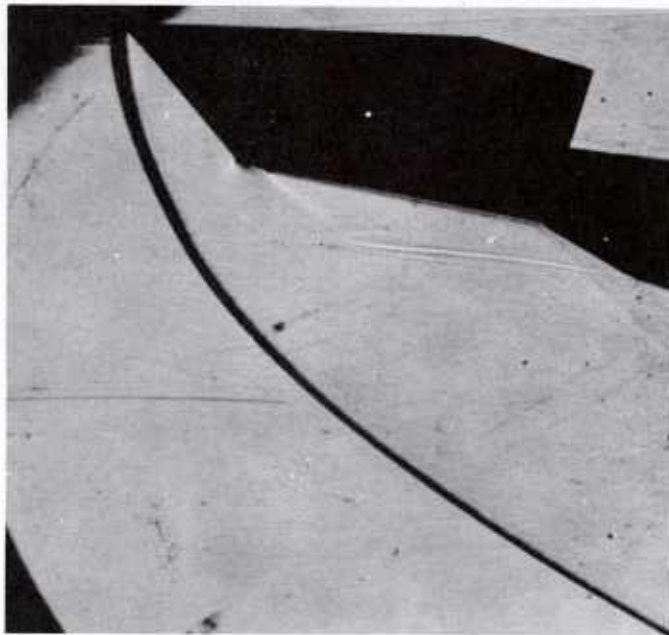
Fig. 12 Schlieren Flow Photographs; M_\infty = 5 , \alpha = +15^\circ and Re_\infty / ft = 3,300,000
