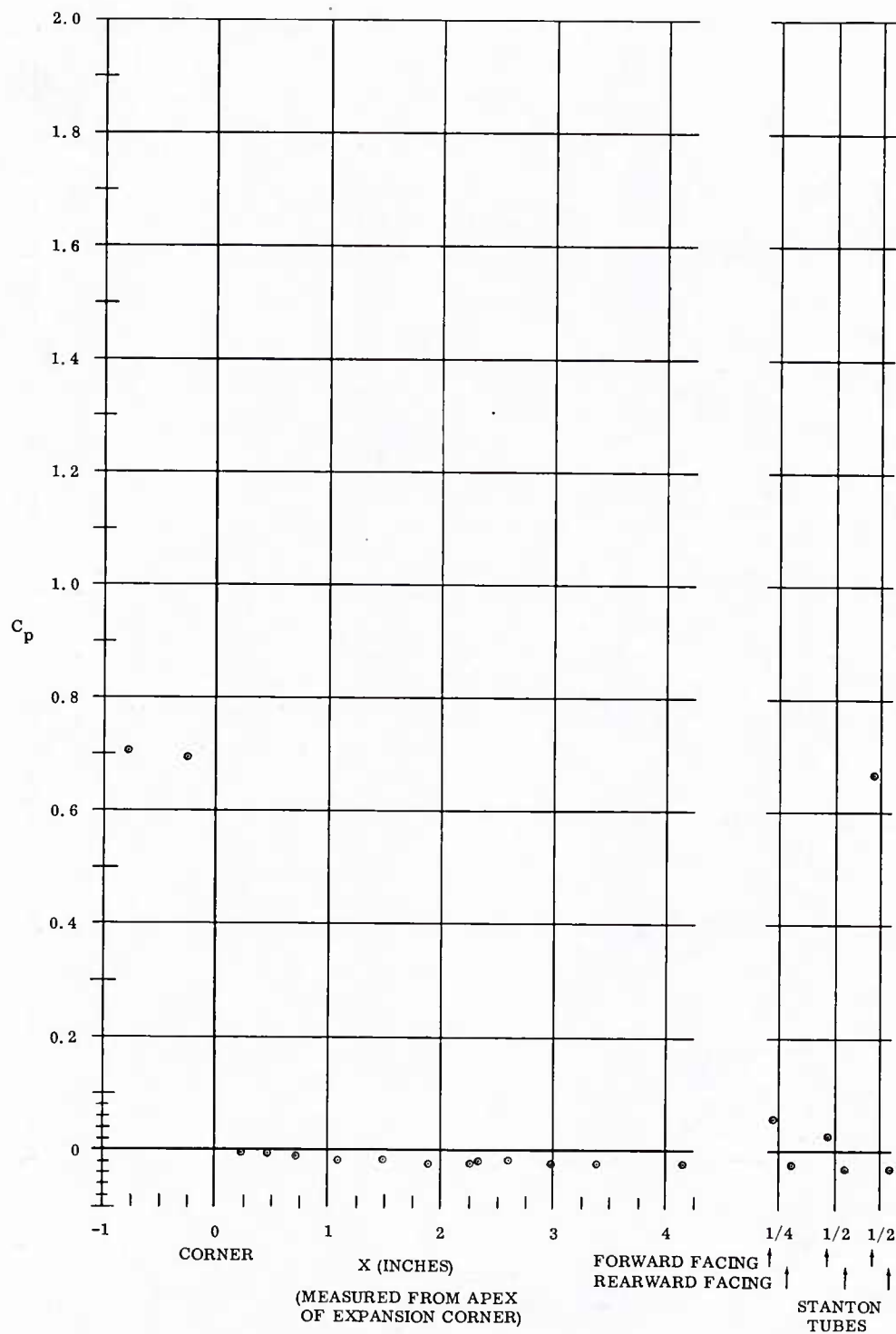
Fig. 21 Pressure Coefficient Distribution over Sharp Expansion Corner M_\infty = 5 ; Re_\infty / ft = 3,300,000 ; \alpha = -5^\circ
