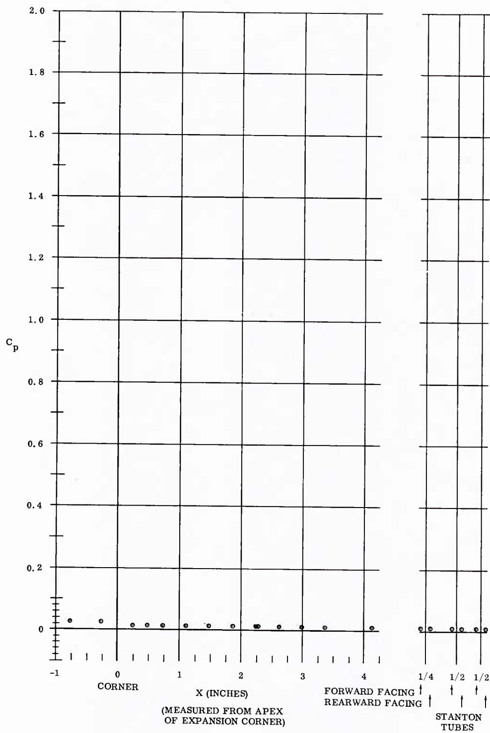
Fig. 42 Pressure Coefficient Distribution over Sharp Expansion Corner M_\infty = 8 ; Re_\infty/\text{ft} = 3,300,000 ; \alpha = -30^\circ
