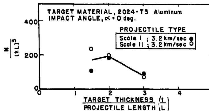
FIGURE 13.- Effect of Projectile Size Upon the Number of Projectile Remnants.
