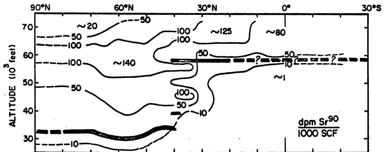
FIGURE 11 MEAN DISTRIBUTION OF STRONTIUM-90 FROM PRE-1961 TESTS STILL PRESENT IN THE STAR DUST SAMPLING CORRIDOR DURING JANUARY-APRIL 1962, CALCULATED FROM Sr^{89}/Sr^{90}
