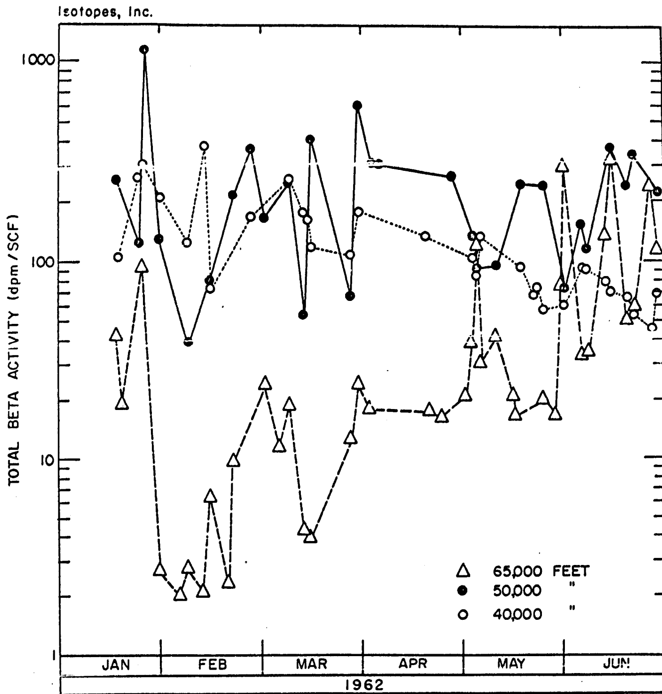
FIGURE 14 THE CHANGE WITH TIME OF THE TOTAL BETA ACTIVITY AT THREE ALTITUDES AT 65°N DURING 1962
