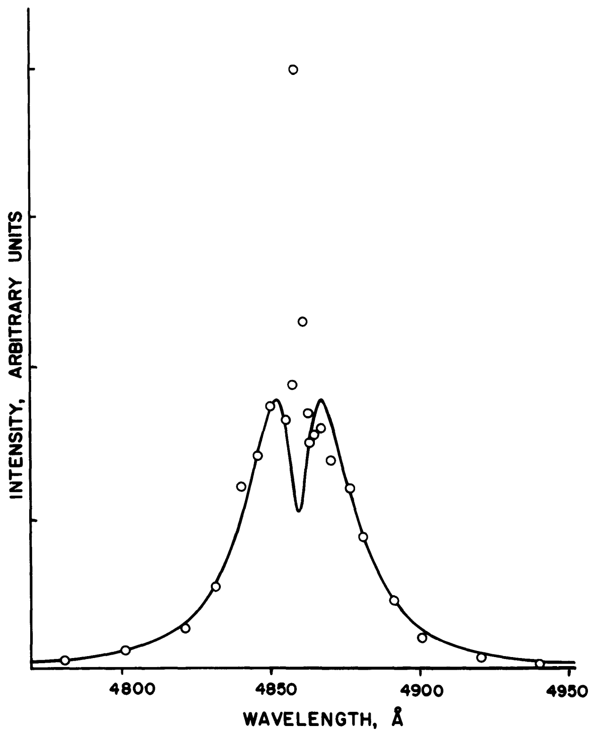
Fig. 11. Spectrum of D_{\beta} Balmer Line at Peak Compression
