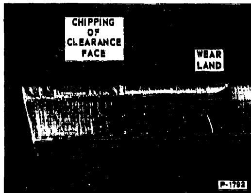
Figure 2-27 - Tool Tip Showing Chipped Clearance Face
