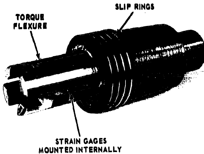
Figure 2-13 - Torque Flexure with Slip Rings
