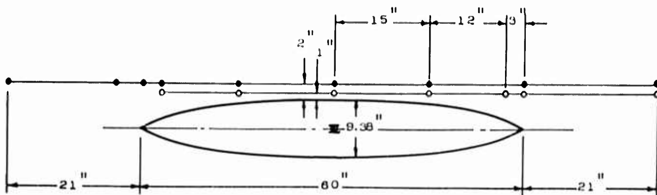
FIG. 4a. Positions of Wave Probes
