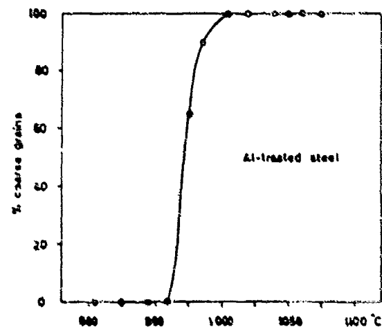
FIG. 13. DIAGRAM SHOWING SPONTANEOUS GRAIN GROWTH IN AN ALUMINUM-TREATED CARBON-MANGANESE STEEL WITH C 0.15%, Si 0.25%, Mn 1.05%.
