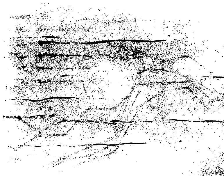
FIG. 26. LONG TINY SULPHIDE INCLUSIONS IN A MICRO-ALLOY COLUMBIUM STEEL AS A RESULT OF A CRITICAL ALUMINUM ADDITION. 200 x
