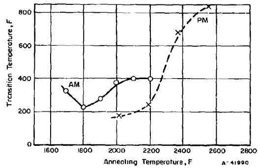
FIGURE A-28. COMPARISON OF BEND-TRANSITION TEMPERATURE OF ARC-MELTED AND POWDER-METALLURGY TUNGSTEN SHEET (11)
