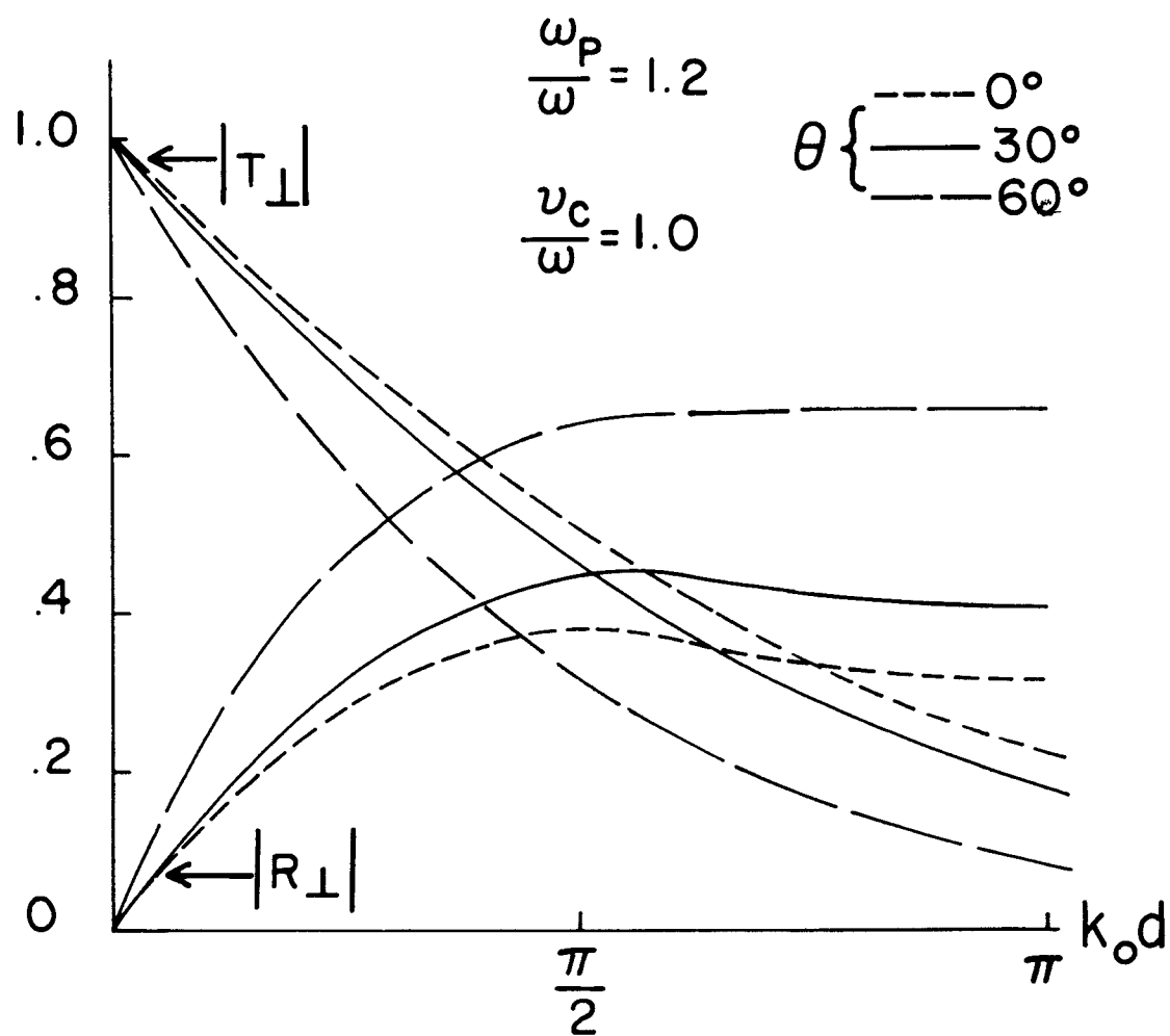
Fig. 5a. Exact Solution, below Cutoff, Lossy (TE Mode)
