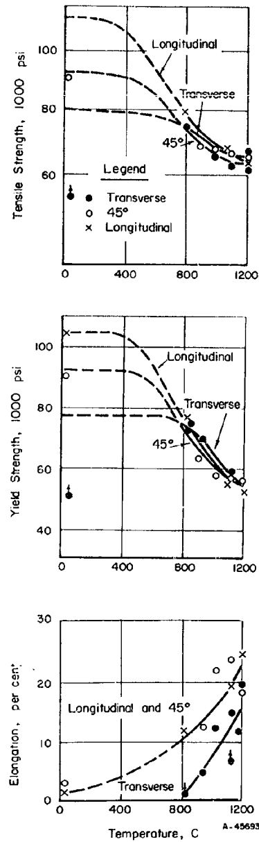
FIGURE A-9. TENSILE-PROPERTY DIRECTIONALITY OF COLUMBIUM SHEET (0.030 INCH) (20)
