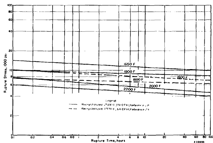
FIGURE A-28. RUPTURE CURVES FOR COMMERCIAL PURE RECRYSTALLIZED COLUMBIUM
