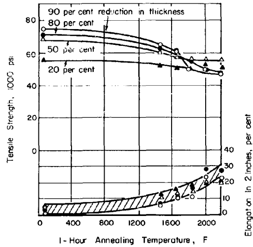
FIGURE A-7. ROOM-TEMPERATURE TENSILE PROPERTIES OF COMMERCIALY PURE ARC-CAST COLUMBIUM AS A FUNCTION OF DEFORMATION AND ANNEALING TEMPERATURE (19)
