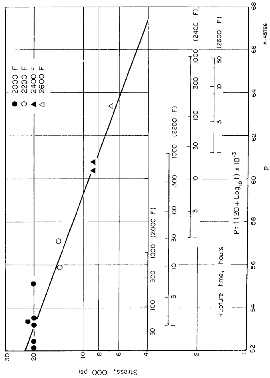
FIGURE A-67. RUPTURE CHARACTERISTICS OF D-43 AT 2000 TO 2600 F (4)
