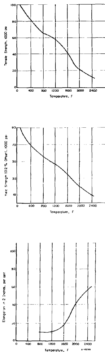
FIGURE A-58. EFFECT OF TEMPERATURE ON THE TENSILE PROPERTIES OF ARC-MELTED RECRYSTALLIZED D-31 SHEET (0.040 INCH)(2)
