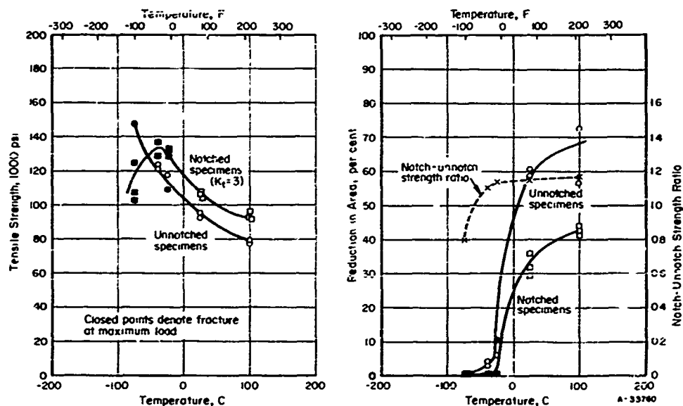
FIGURE A-29. TENSILE PROPERTIES FOR WROUGHT, STRESS-RELIEVED ARC-MELTED MOLYBDENUM SHEET (1/4 HR AT 1000 C; HARDNESS 222 VHN) (22)
