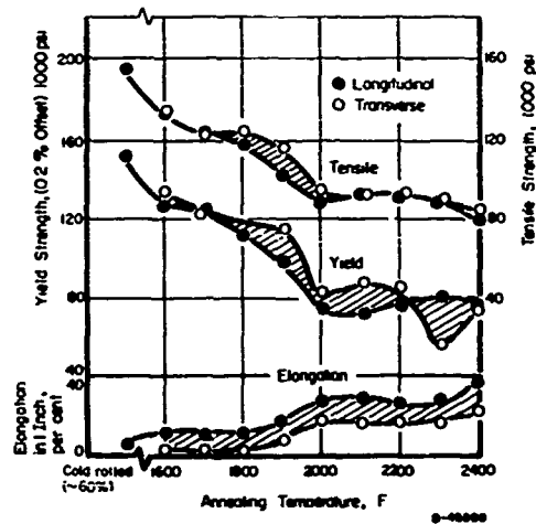
FIGURE A-7. EFFECT OF ANNEALING TEMPERATURE ON THE ROOM-TEMPERATURE TENSILE PROPERTIES OF COMMERCIAL-PURITY ARC-CAST MOLYBDENUM SHEET (0.020 INCH)(28)
