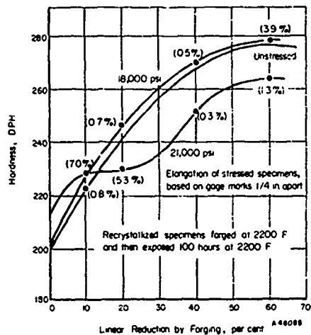
FIGURE A-132. EFFECT OF LINEAR FORGING REDUCTION AND HEATING UNDER IMPOSED STRESSES ON THE ROOM-TEMPERATURE HARDNESS OF TZM (5)
