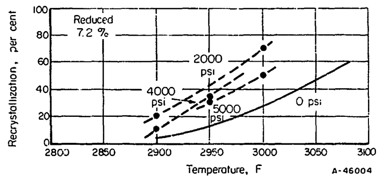
FIGURE A-141. RECRYSTALLIZATION BEHAVIOR AS A FUNCTION OF TEMPERATURE AND EXTERNALLY APPLIED STRESS FOR T2M BARS (24)
