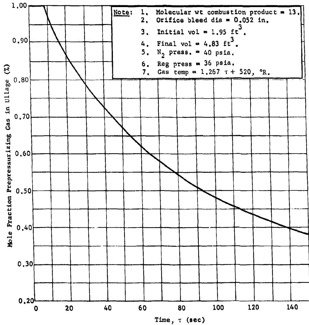
Fig. II-114 Ullage Gas Dilution for the Small Scale Single Tank System
