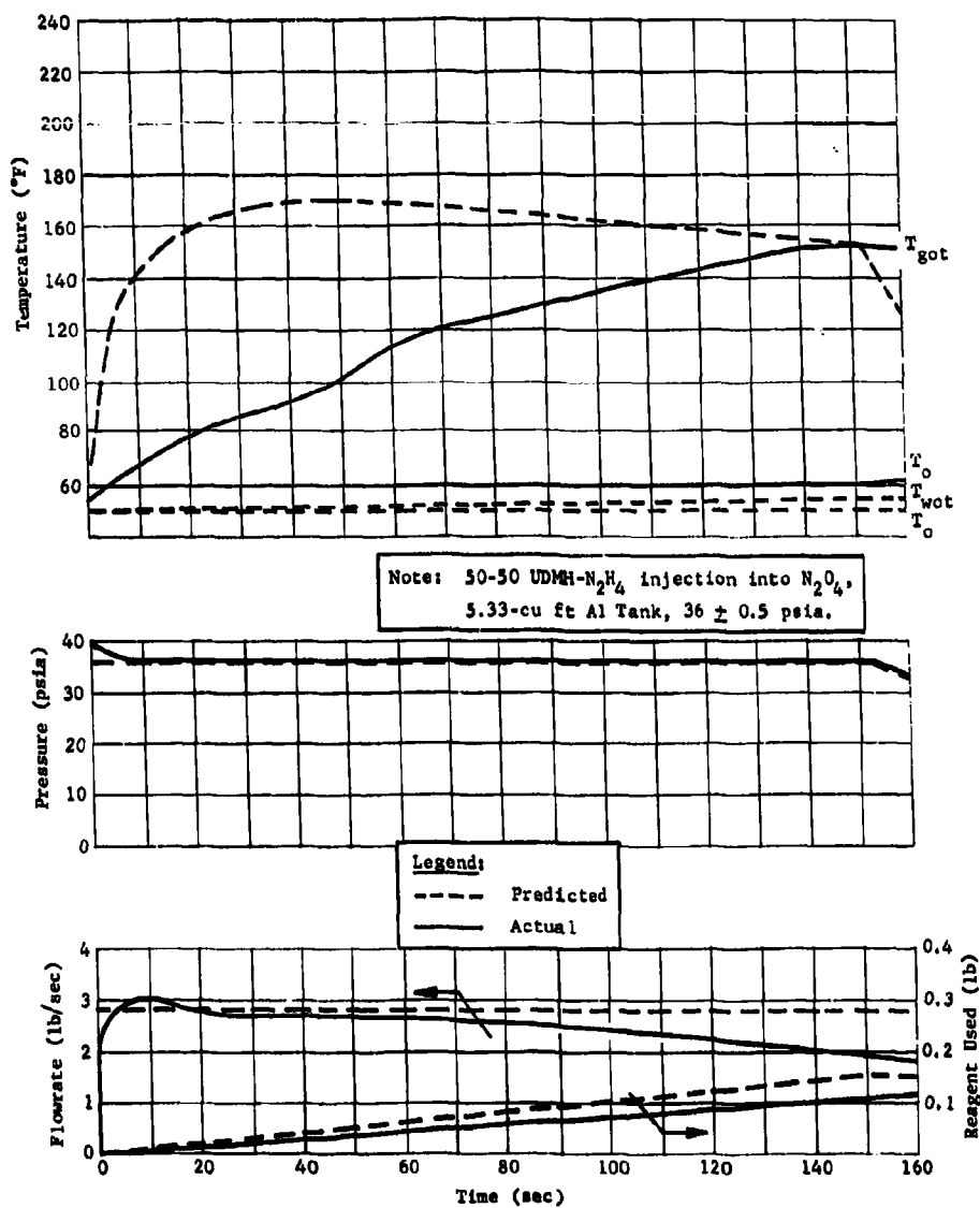
Fig. III-11 MTI Phase I Oxidizer Tank Performance
