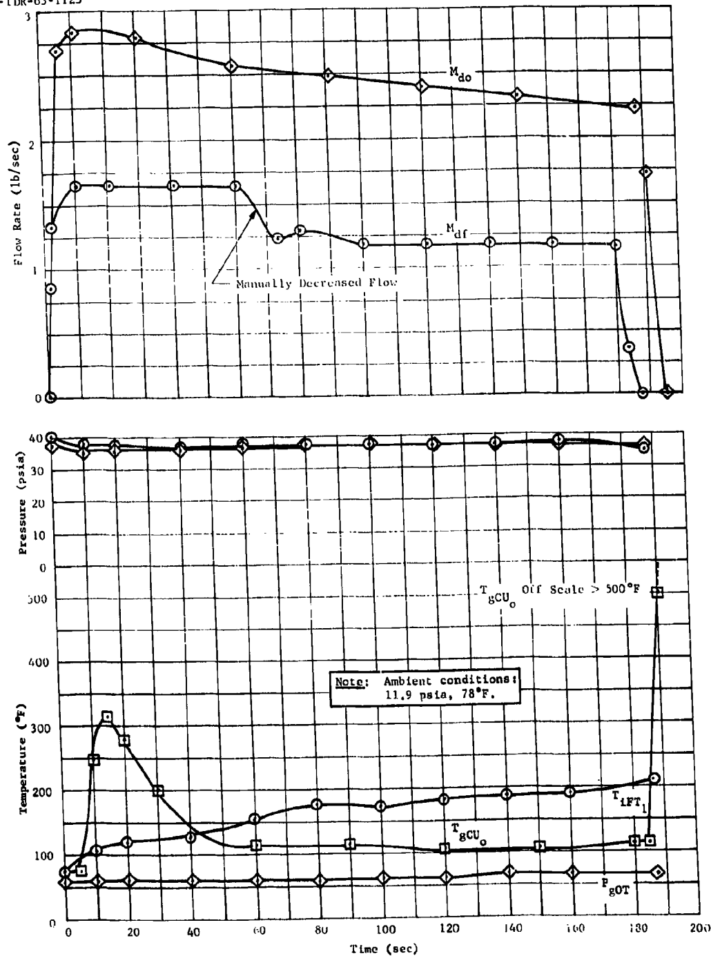
Fig. II-102 Parametric Test Common Ullage System Performance at 36 psia
