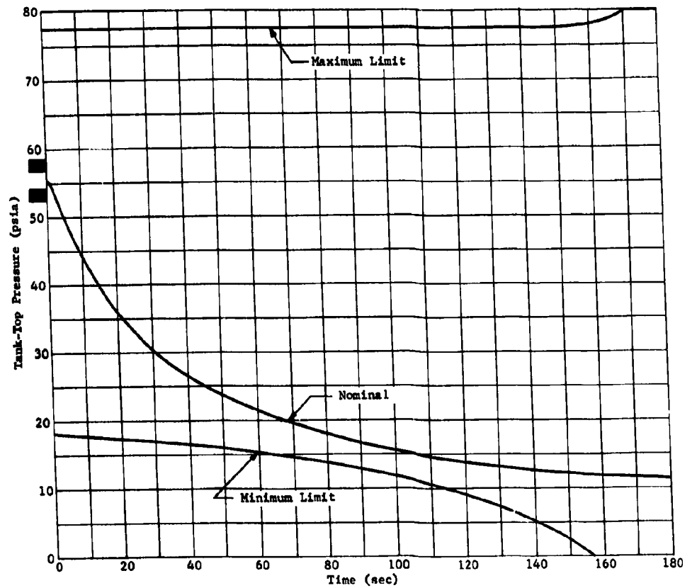
Fig. V-22 Flight Tank Pressure, Stage II Oxidizer Tank
