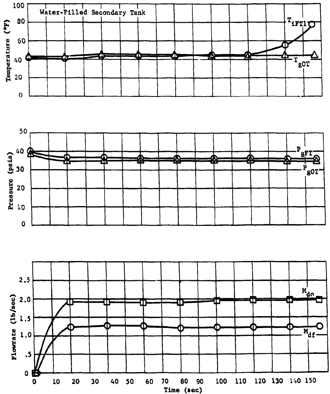
Fig. II-75 Pressurization System Performance Curves with 15-deg Fan Spray Subsurface Injection in Primary Tank
