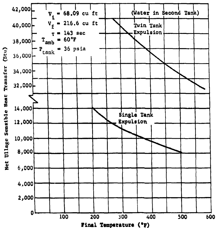
Fig. III-4 Phase III Fuel Tank Ullage Heat Transfer vs Final Pressurant Temperature
