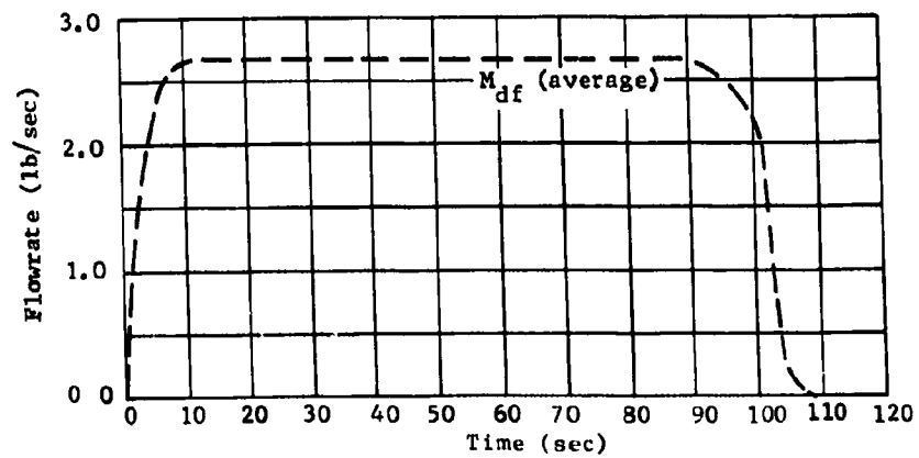
Fig. II-107 Parametric Test Fuel Tank System Performance at 200 psia
