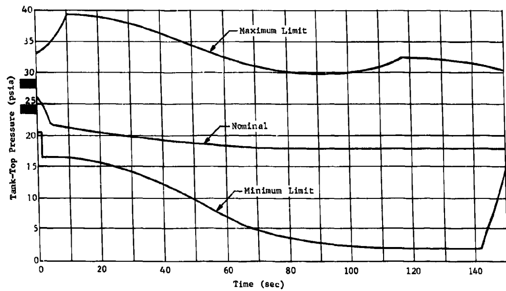
Fig. V-20 Flight Tank Pressure, Stage I Oxidizer Tank
