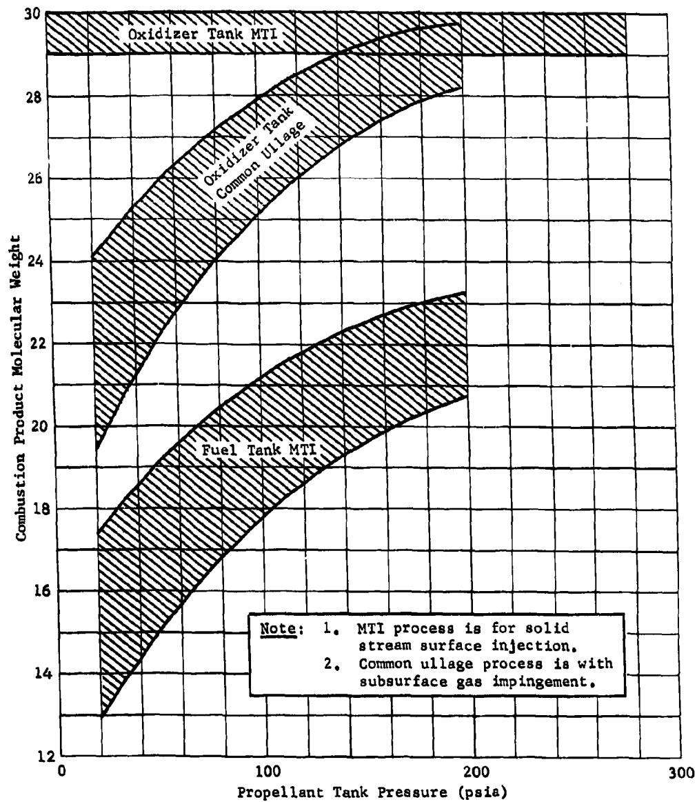
Fig. V-11 Combustion Product Molecular Weight for MTI Pressurization Systems
