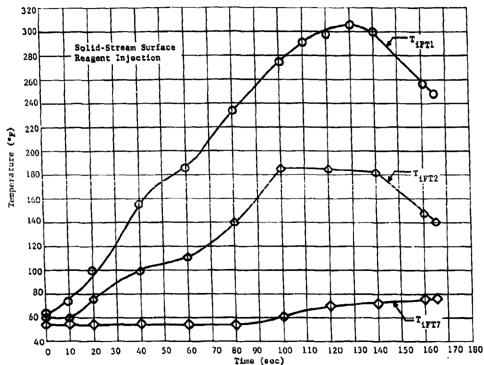
Fig. II-86 Primary Tank Internal Temperatures with Subsurface Gas Impingement in Oxidizer Tank
