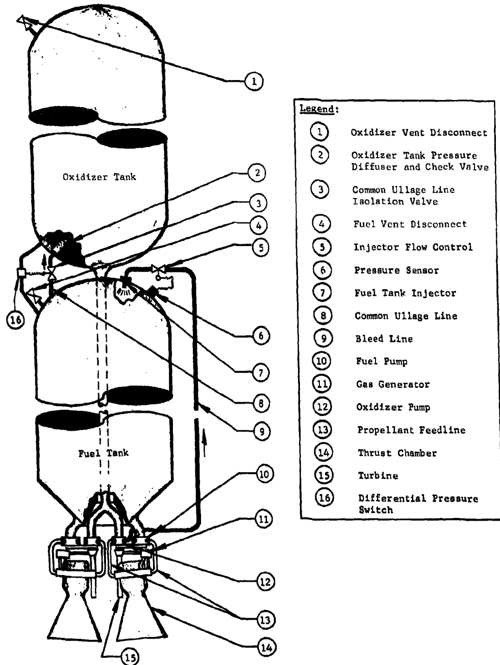
Fig. V-26 Pulse-Type MTI with Turbopump Bleed, Common Ullage System
