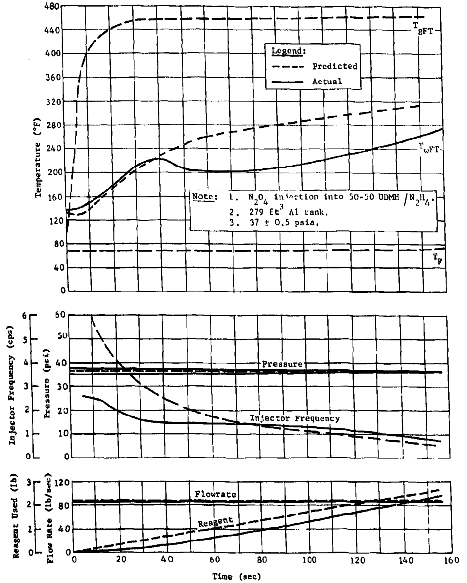
Fig. V-9 Phase III MTI Fuel Tank Performance
