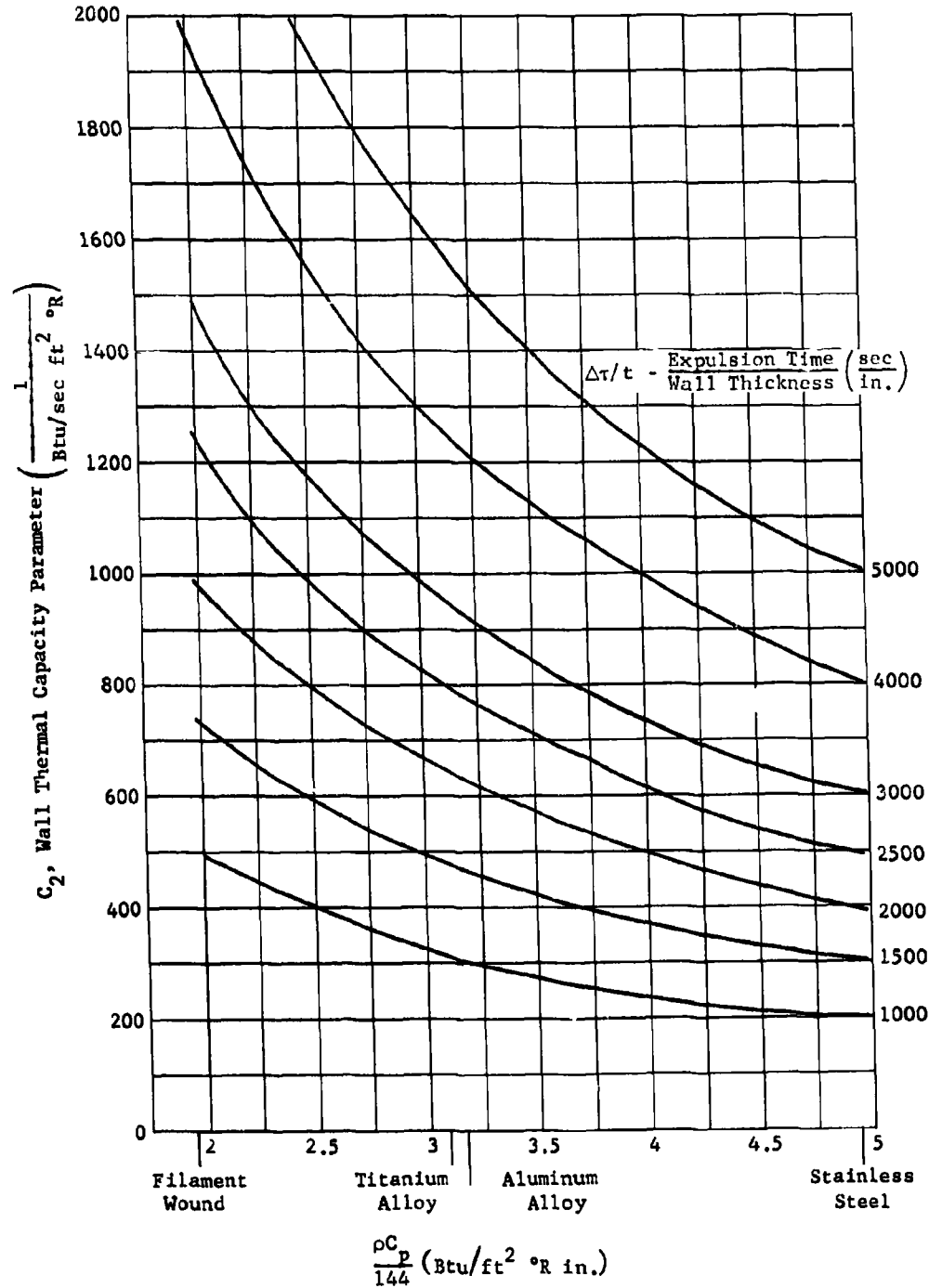
Fig. V-14 Tank Wall Thermal Capacity
