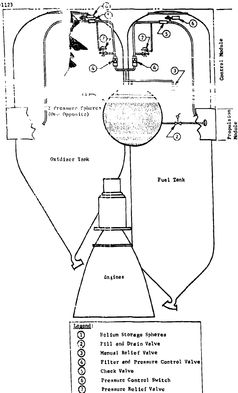
Fig. V-31 Titan III Transtage Helium Pressurization System (Configuration 1)
