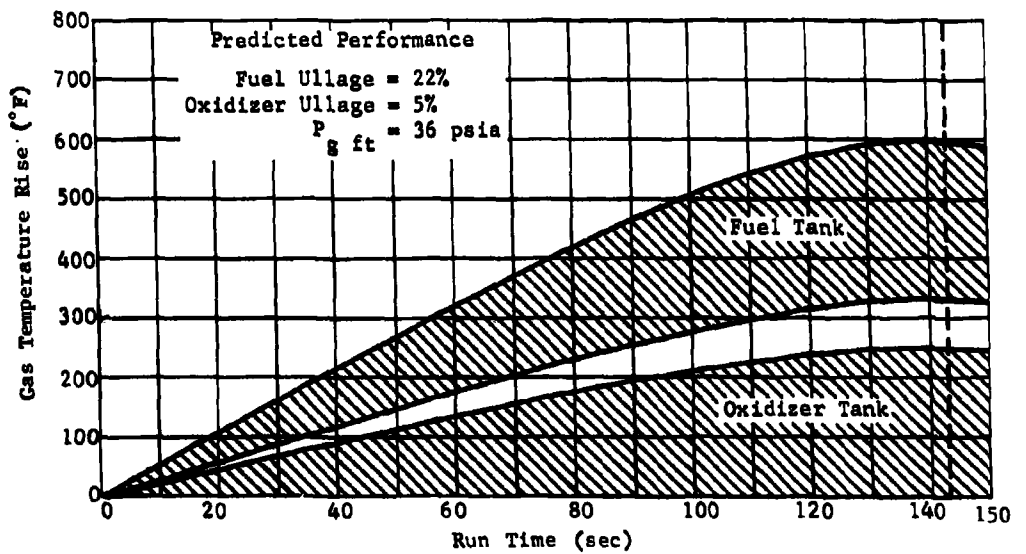
Fig. III-7 Phase III Predicted Performance Range
