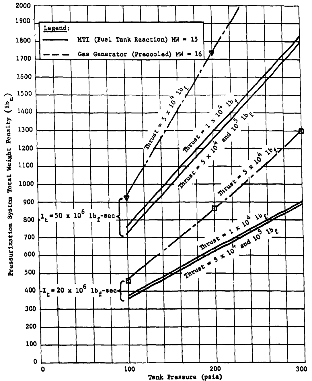
Fig. II-34 MTI vs Gas Generator Pressurization Systems, Case III, Upper Stage Vehicle
