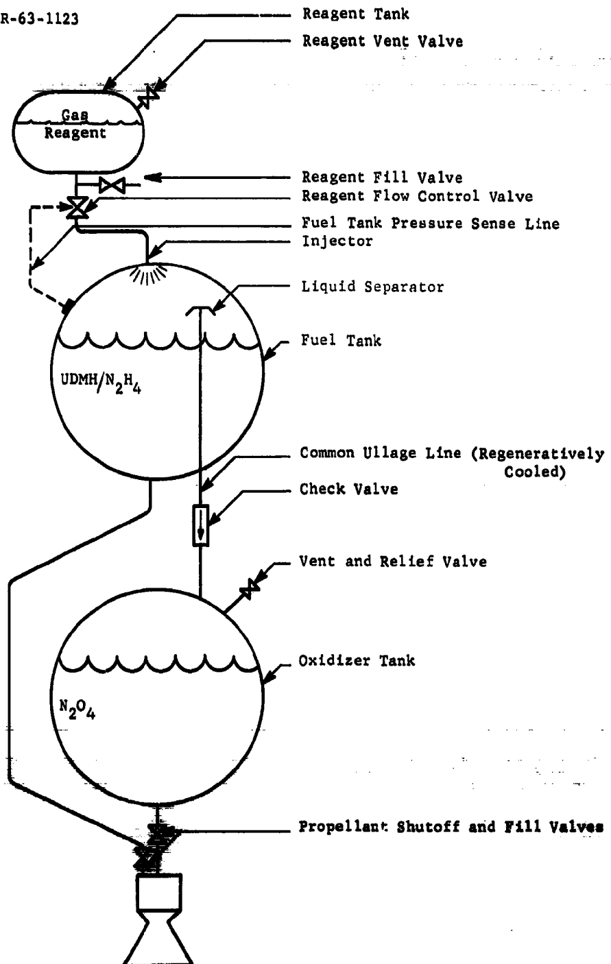
Fig. II-5 Common Ullage MTI Pressurization System with Pneumatically Pressurized Remote Reagent Storage, Pressure-Fed Engine
