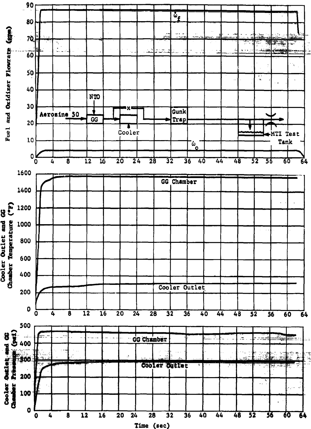
Fig. II-11 MTI Common Ullage Feasibility "Open Container" Test, Surface Impingement
