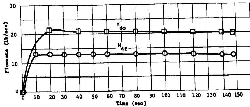
Fig. II-69 Pressurization System Performance Curves with 15-deg Fan Spray Surface Injection in Primary Tank
