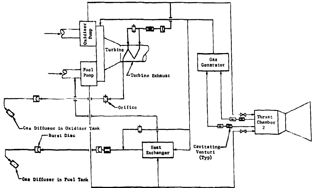
Fig. V-17 Existing Titan II Pressurization System, Stage I
