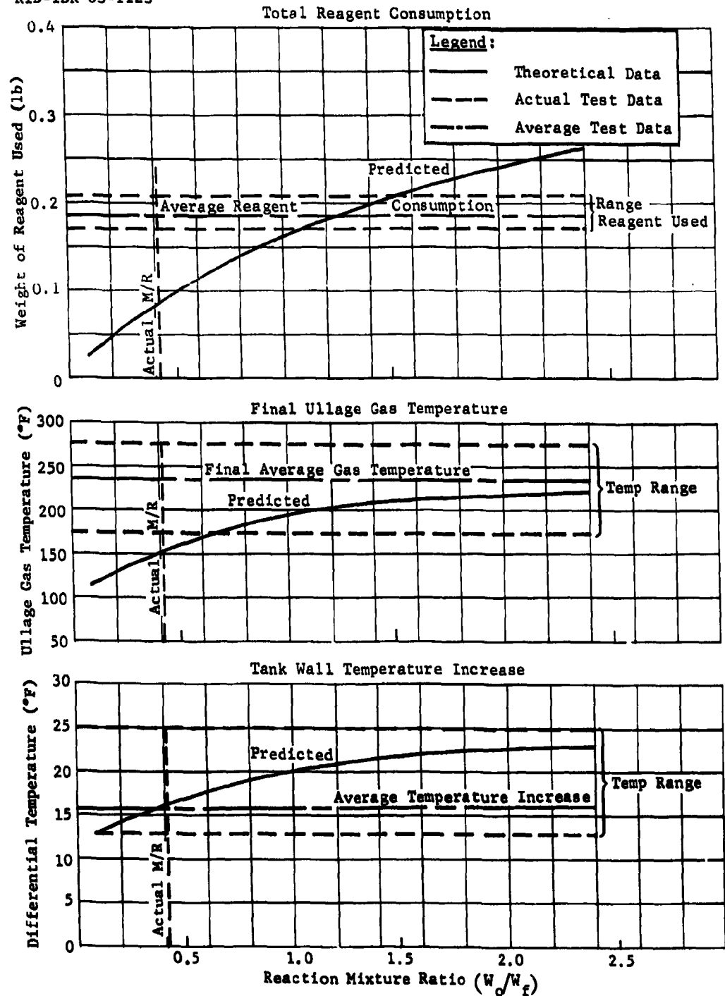
Fig. II-57 Phase I Fuel Tank Pressurization System Performance Evaluation ( N_2O_4 Solid-Stream Surface Injection, Single Tank Test)
