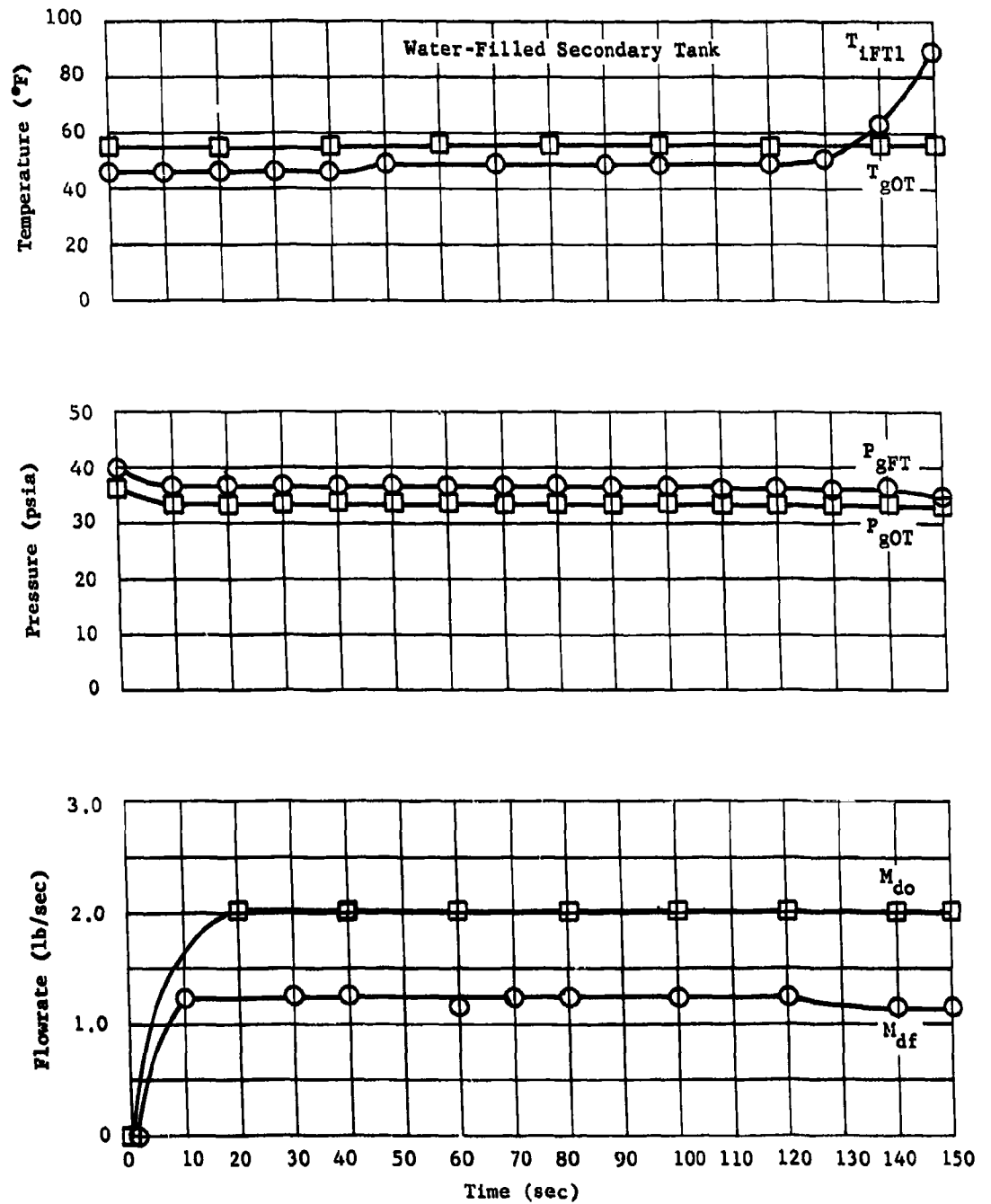
Fig. II-72 Pressurization System Performance Curves with Solid-Stream Subsurface Injection in Primary Tank
