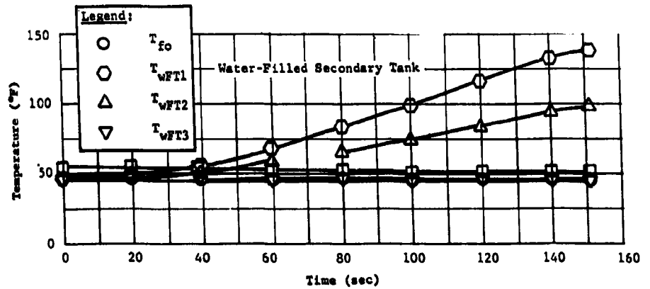
Fig. II-71 Primary Tank External Temperatures for 15-deg Fan Spray Surface Reagent Injection
