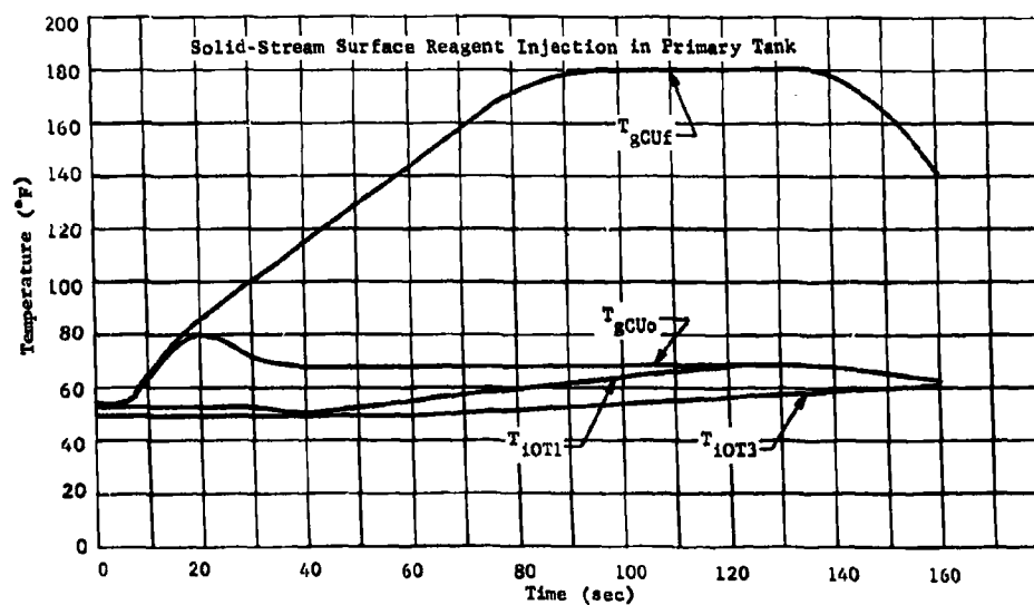
Fig. II-87 Oxidizer Tank Temperatures with Subsurface Gas Impingement
