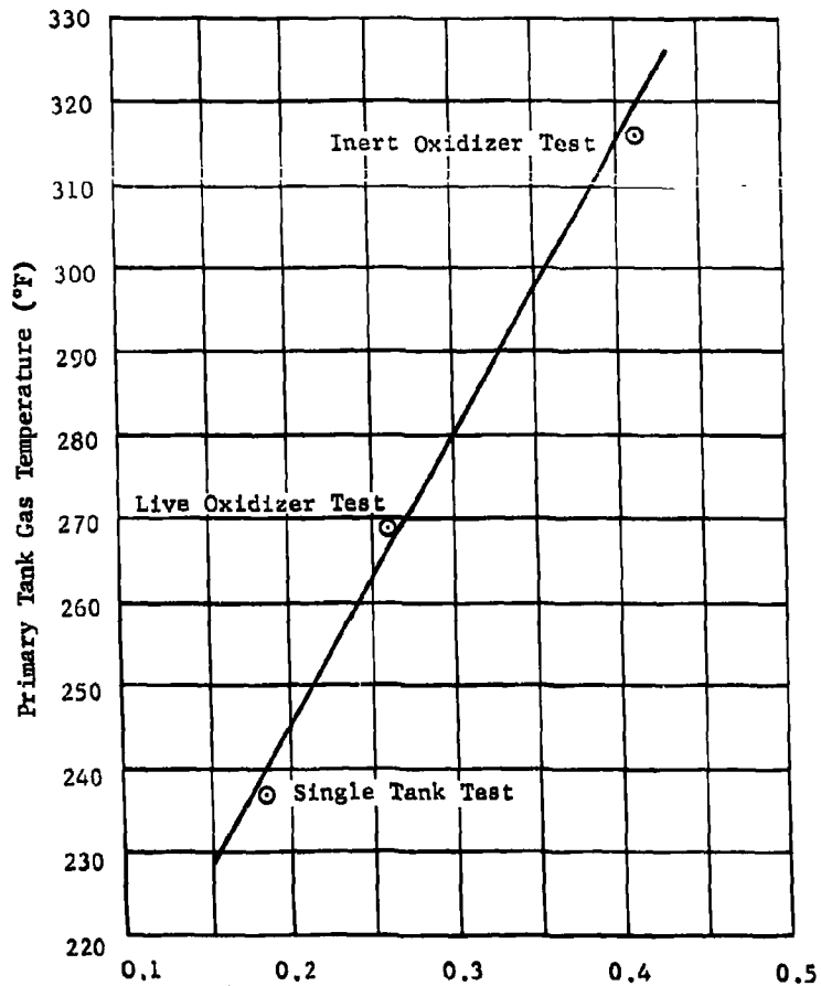
Fig. II-100 Phase I Fuel Tank Gas Temperature vs Reagent Consumption
