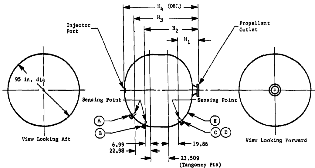
Fig. III-34 Phase III Tankage
