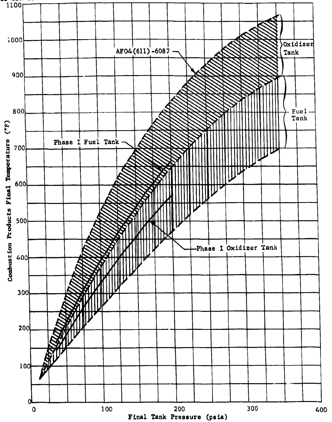
Fig. V-5 MTI Final Gas Temperature Comparisons, Small-Scale Systems
