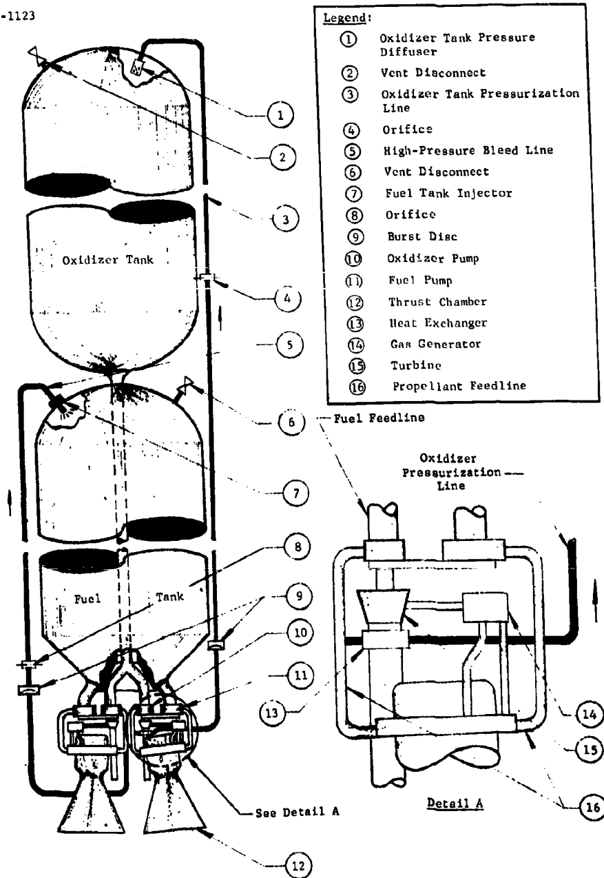
Fig. V-25 Constant Flow-Type MTI, Turbopump, Bleed Fuel Tank Pressurization, Evaporated Propellant Oxidizer Pressurization
