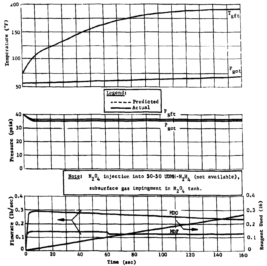
Fig. III-12 MTI Phase I Common Ullage System Performance
