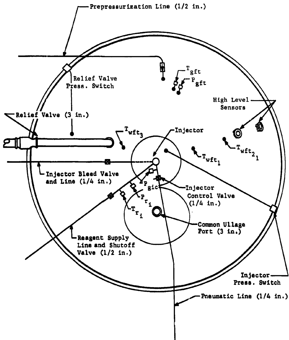
Fig. IV-2 Instrumentation Location Phase III Tank Plan (Top) View
