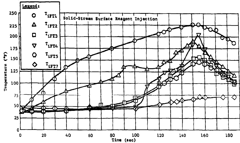
Fig. II-82 Primary Tank Internal Temperature Profile with Surface Gas Impingement in Oxidizer Tank
