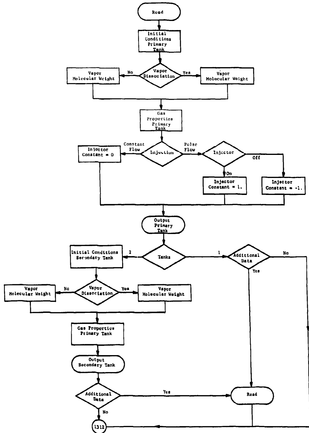
Fig. F-3 Detailed Logic Sequence
