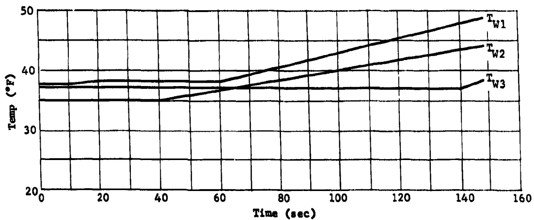
Fig. II-56 Fuel Tank Wall Temperature Profile
