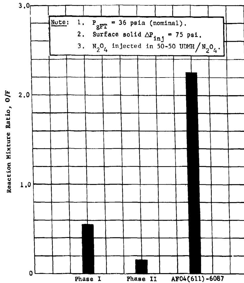
Fig. V-4 Reaction Mixture Ratio - MTI Fuel Tank
