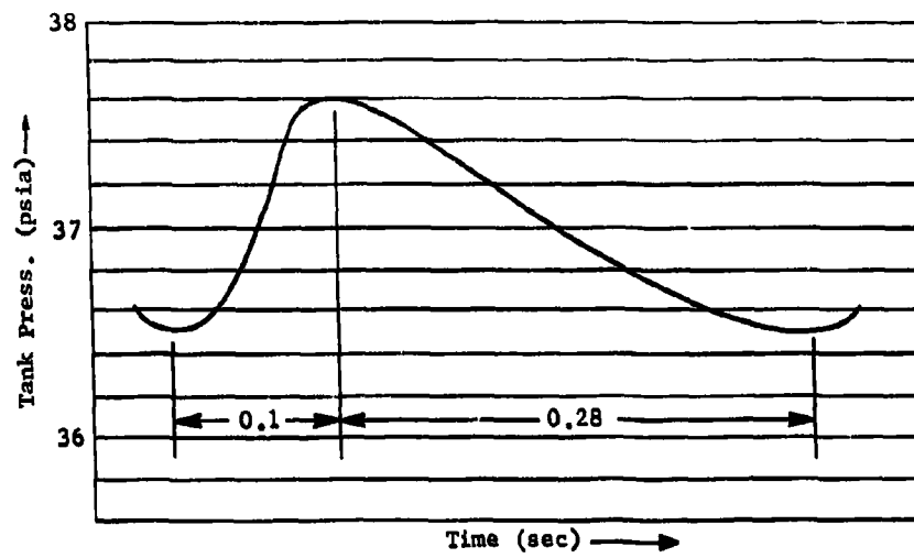
Fig. IV-13 Typical Pressure Cycle at 5% Ullage
