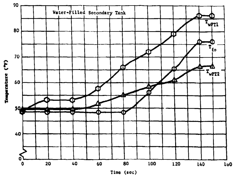
Fig. II-68 Primary Tank External Temperatures for Solid-Stream Surface Reagent Injection
