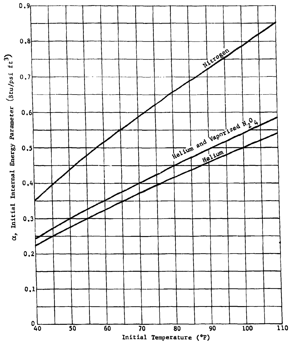
Fig. V-15 Initial Internal Energy of Prepressurants
