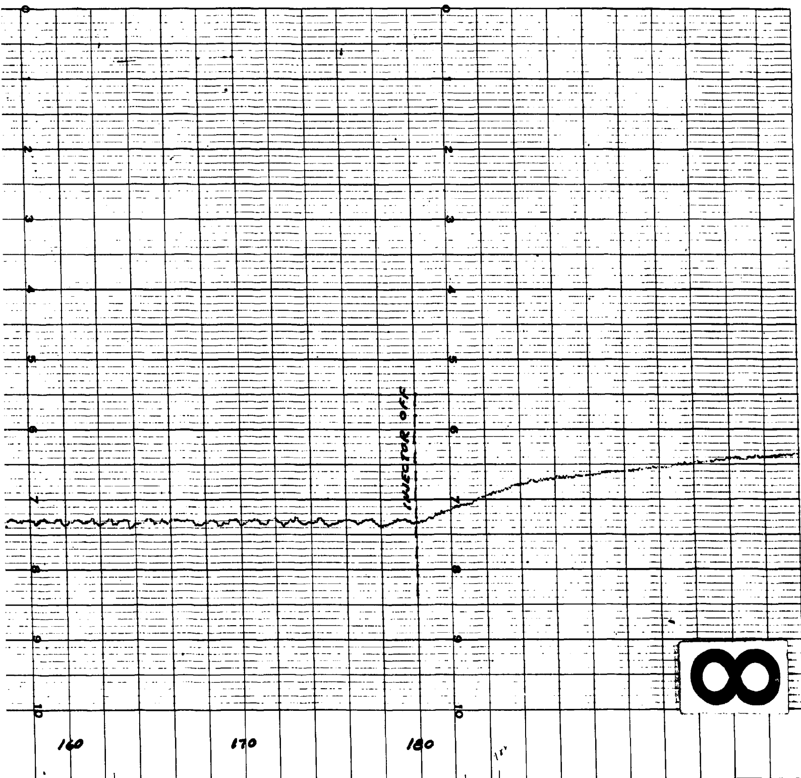
Fig. IV-17 Run 5 Actual Phase III Fuel Tank Pressure Trace, Restart Test IV-33 and IV-34
