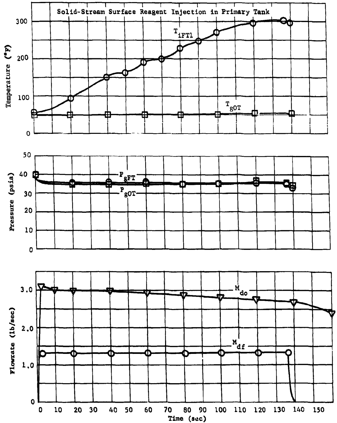
Fig. II-85 Pressurization System Performance Curves with Subsurface Gas Impingement in Oxidizer Tank
