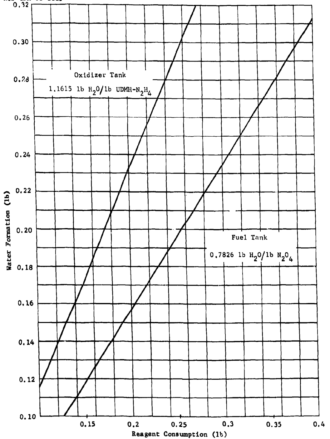
Fig. II-123 Theoretical Maximum Water Concentration in the Fuel vs Reagent Consumption
