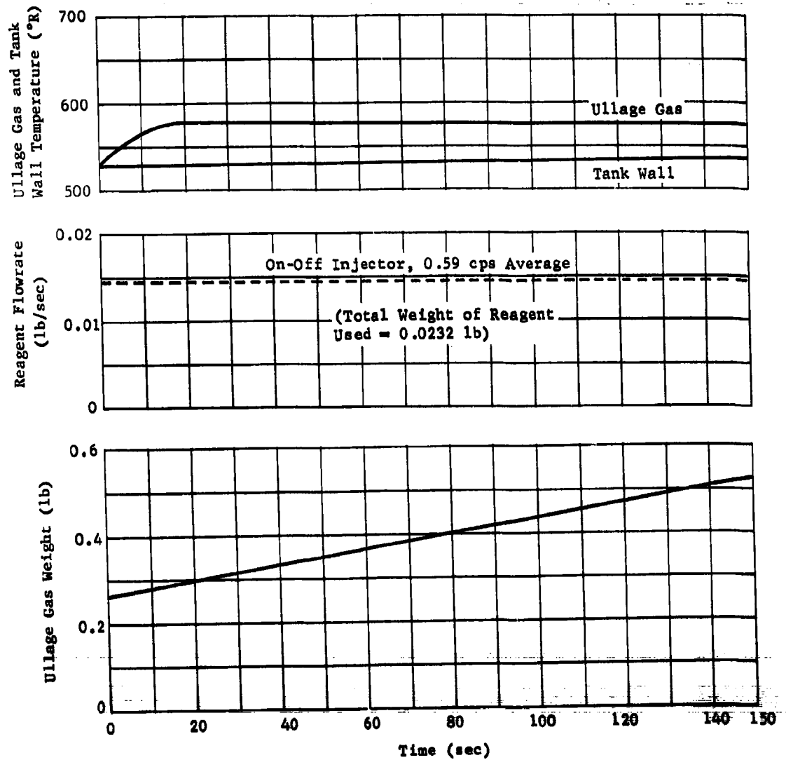
Fig. II-27 Phase I Fuel Tank Predicted Performance for a Mixture Ratio of 0.1 and Pressure of 36 psia
