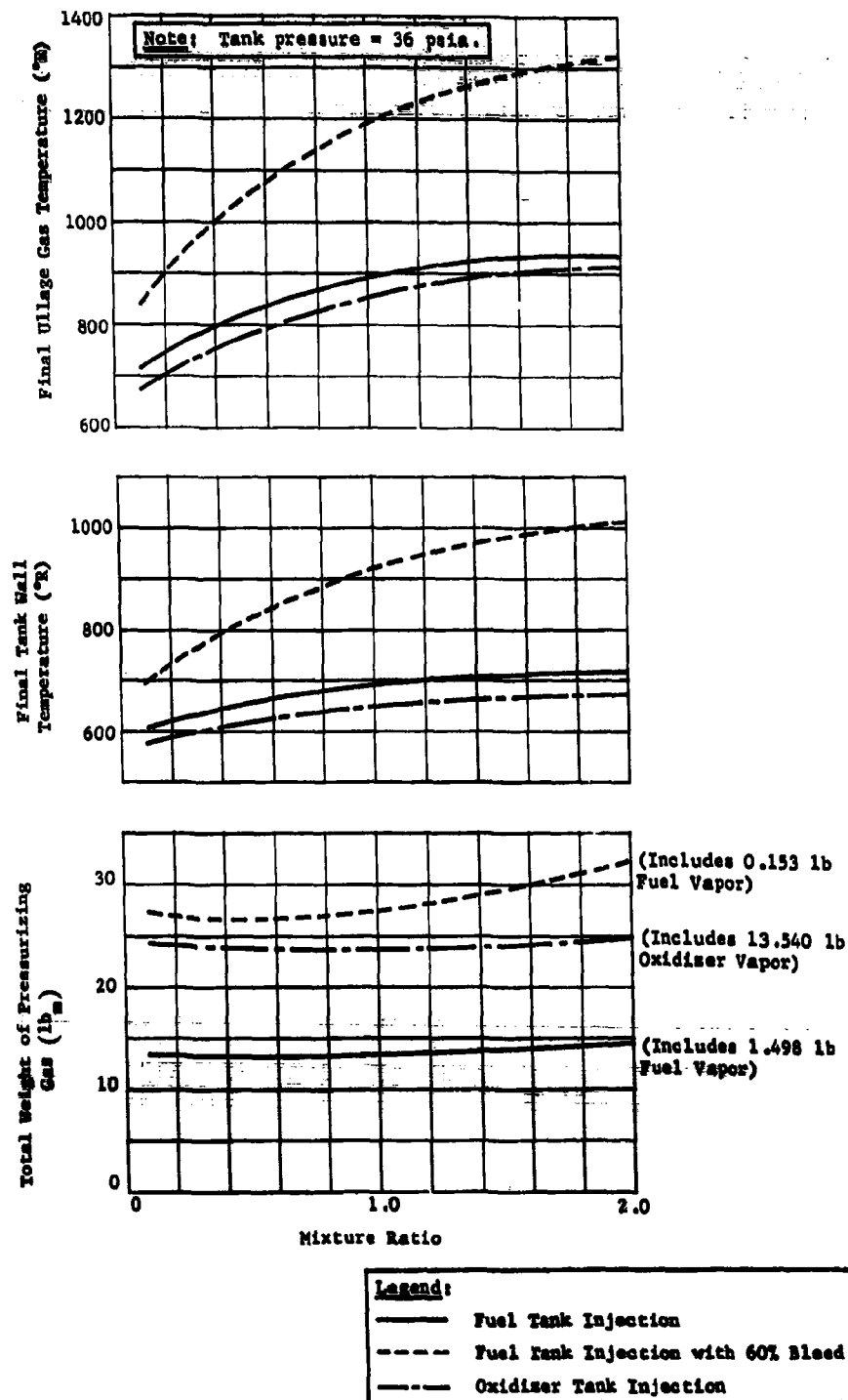
Fig. II-28 Theoretical Phase III System Performance for the Fuel and Oxidiser Tank
