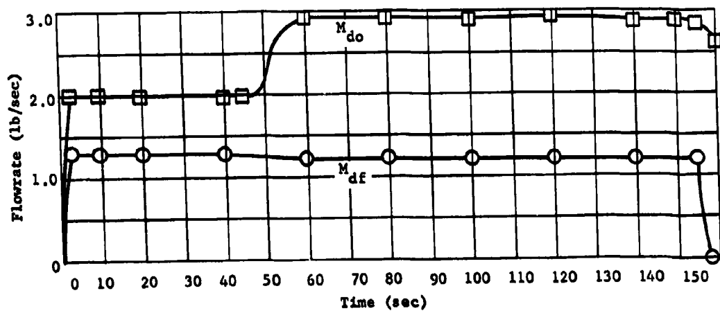
Fig. II-79 Pressurization System Performance Curves with Surface Gas Impingement in Oxidizer Tank
