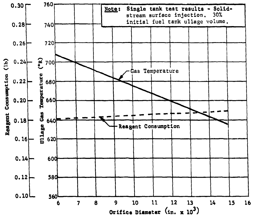
Fig. II-61 Orifice Size Effect on Ullage Gas Temperature and Reagent Consumption
