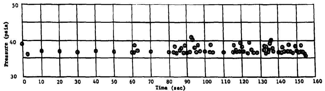
Fig. II-81 Secondary Tank Pressure Profile with Surface Gas Impingement on Oxidizer
