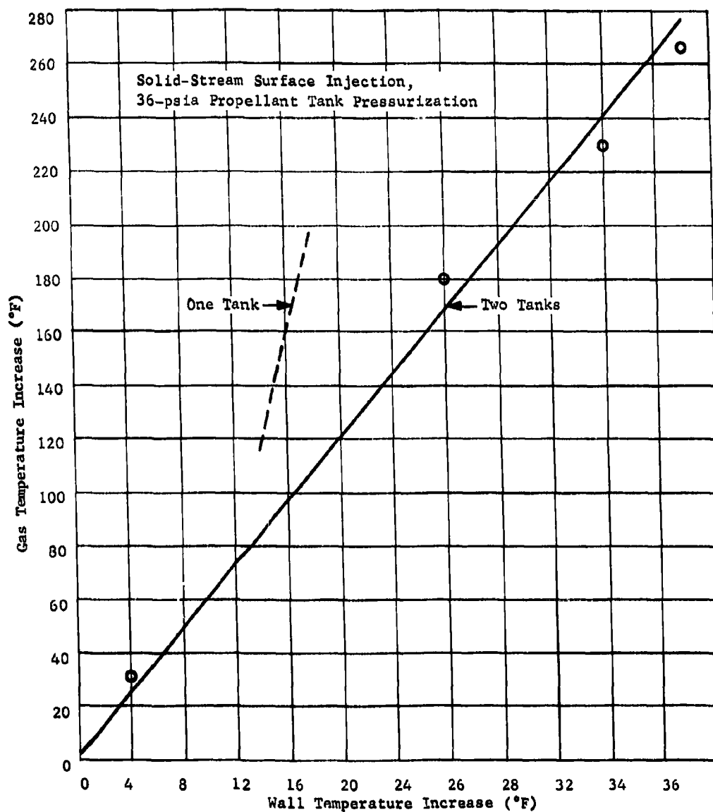
Fig. II-101 Phase I Fuel Tank Wall Temperature Increase vs Gas Temperature Increase
