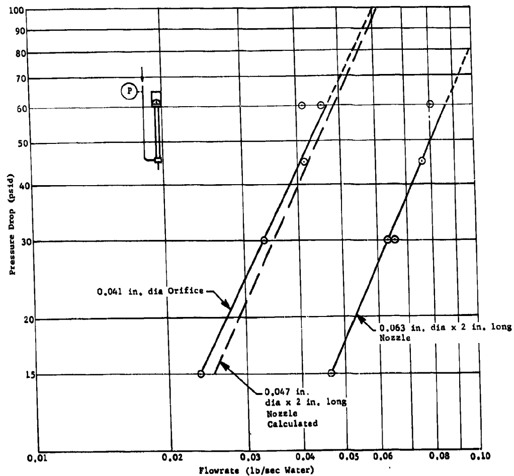
Fig. III-27 Phase III Injector Flow Capacity
