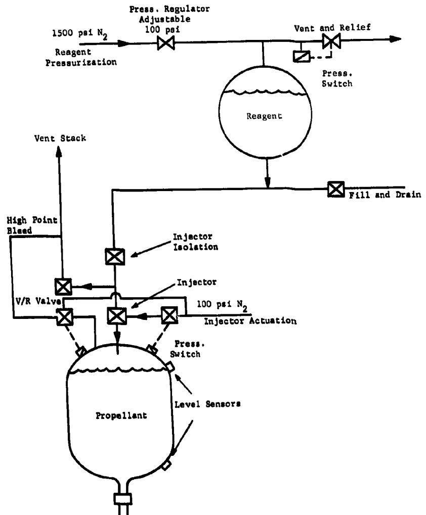
Fig. III-22 Main Tank Injection Phase III Separate Reagent Injection System
