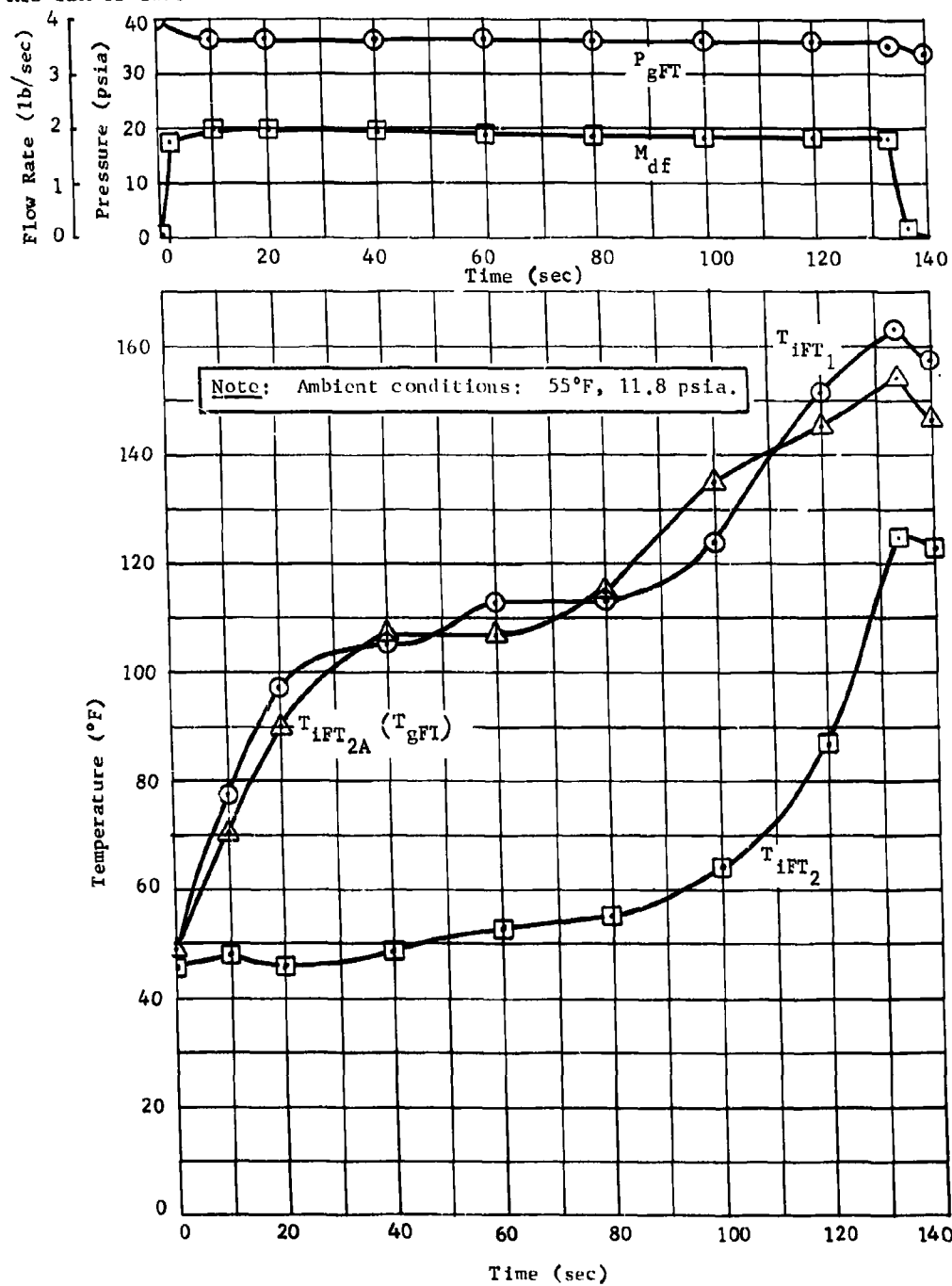
Fig. II-105 Parametric Test Fuel Tank System Performance at 36 psia
