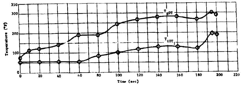
Fig. II-111 Parametric Test Oxidizer Tank System Performance at 100 psia
