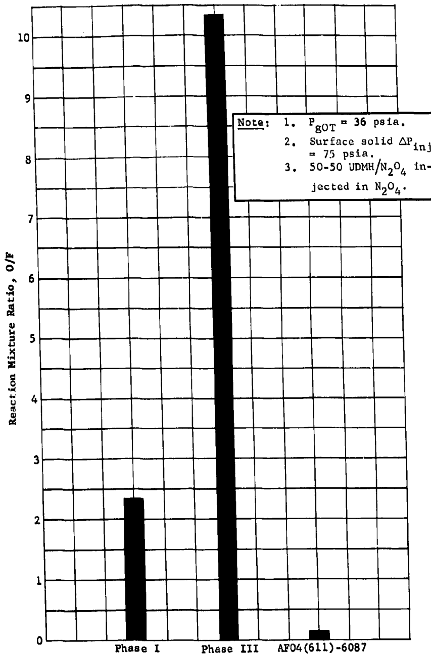
Fig. V-3 Reaction Mixture Ratio - MTI Oxidizer Tank
