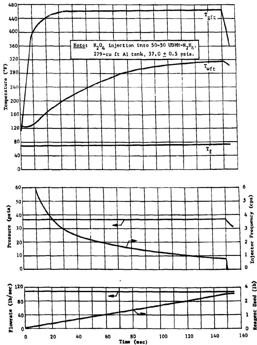
Fig. III-13 Phase III MTI Fuel Tank Performance, Predicted
