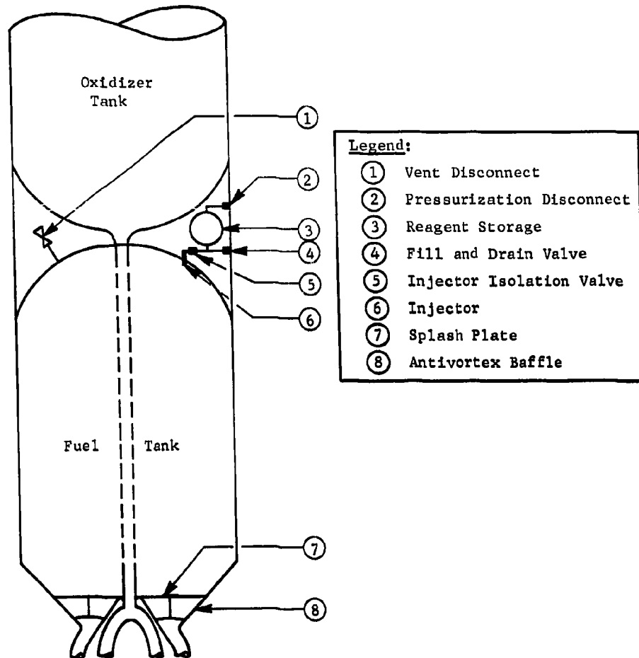
Fig. V-29 Titan II, Stage I Fuel Tank, MTI Pressurization System
