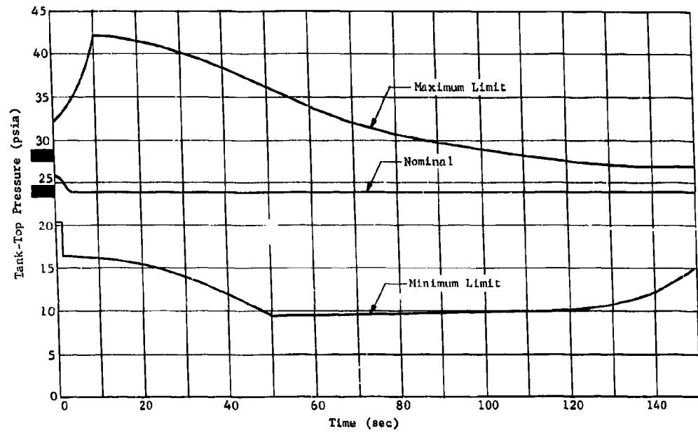
Fig. V-19 Flight Tank Pressure, Stage I Fuel Tank
