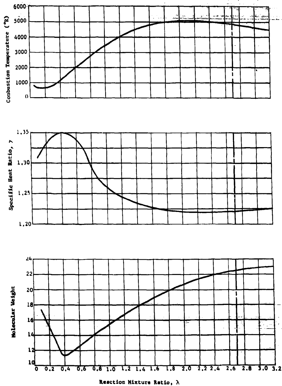
Fig. II-23 Thermodynamic Properties of \text{N}_2\text{O}_4\text{-NH}_3 Combustion Products at 36 psia
