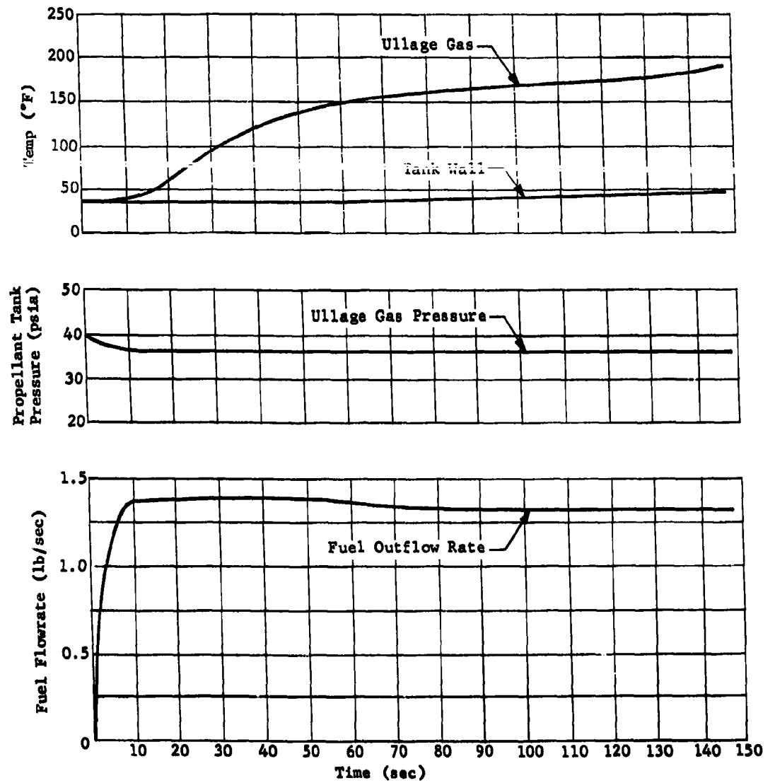
Fig. II-54 Typical Single Tank Pressurization System Performance with Solid-Stream Surface Injection
