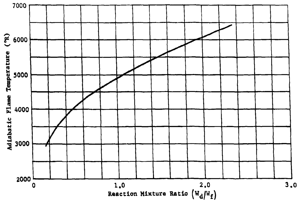
Fig. III-16 Theoretical Reaction Temperature Based on Actual Combustion Products at 36 psia
