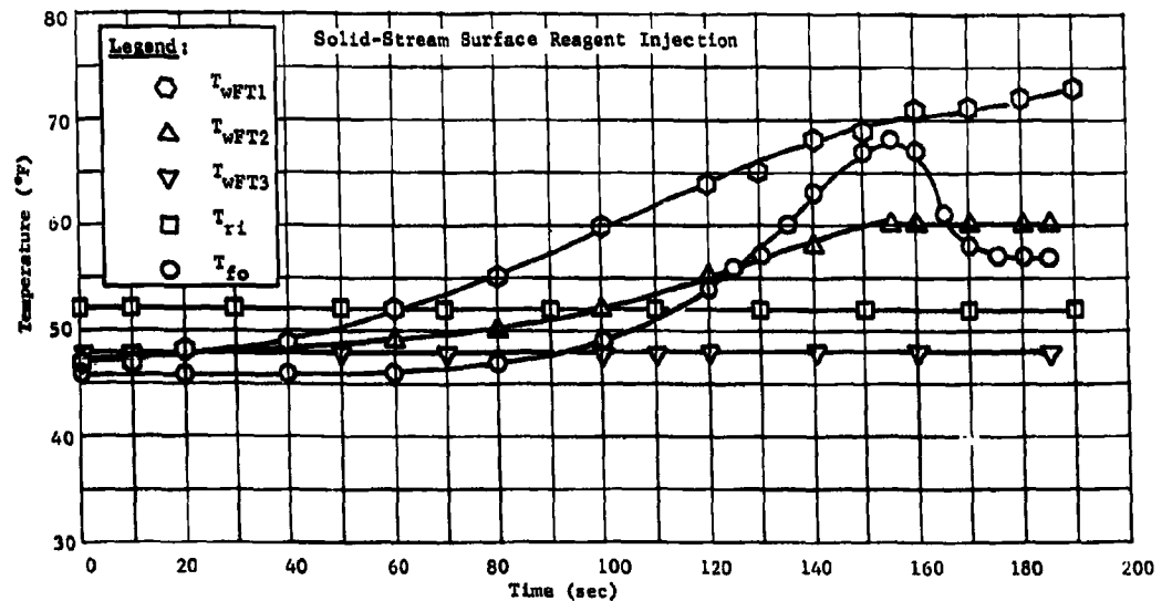
Fig. II-83 Primary Tank External Temperature Profile with Surface Gas Impingement in Oxidiser-Filled Secondary Tank
