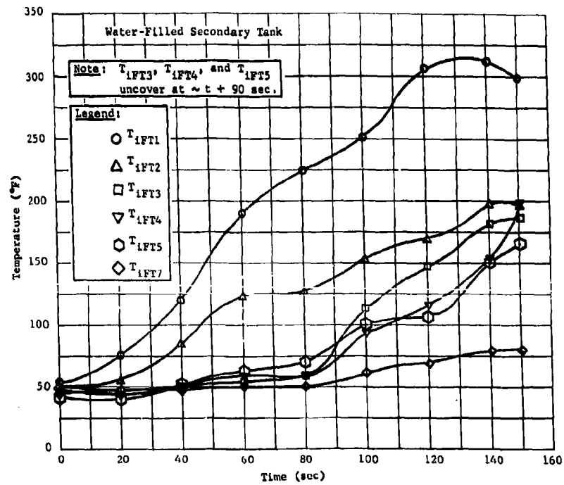
Fig. II-67 Primary Tank Internal Temperature Profiles with Solid-Stream Surface Reagent Injection
