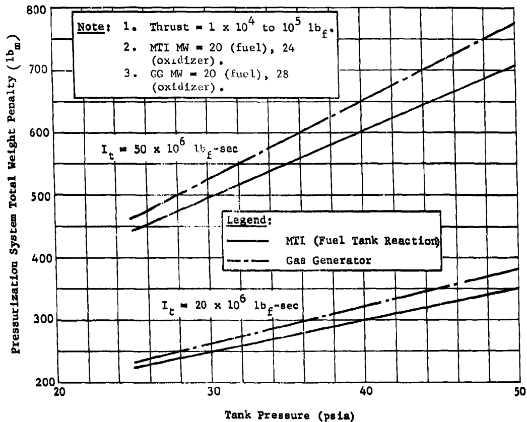
Fig. II-35 MTI vs Gas Generator Pressurization Systems, Case IV, Limited Space Vehicle, 1 Month Storage
