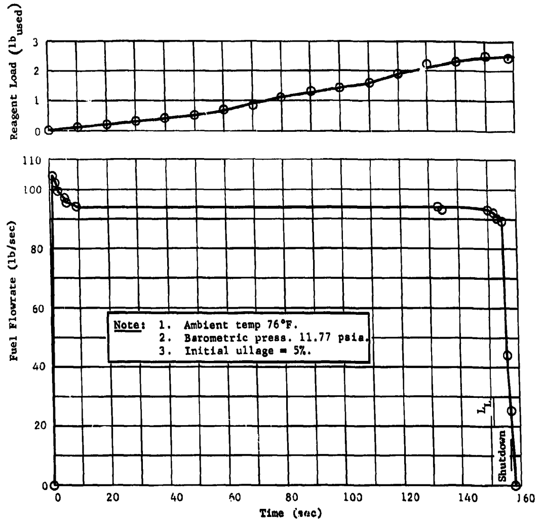
Fig. IV-12 Run 4 Phase III Fuel Tank Pressurization and Propellant Flowrates
