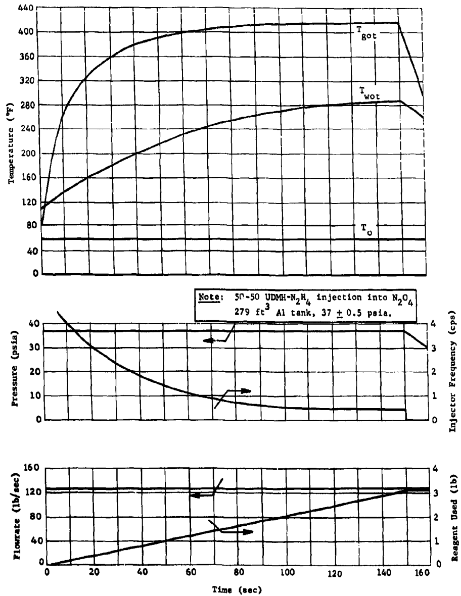
Fig. III-14 Phase III MTI Oxidizer Tank Performance, Predicted
