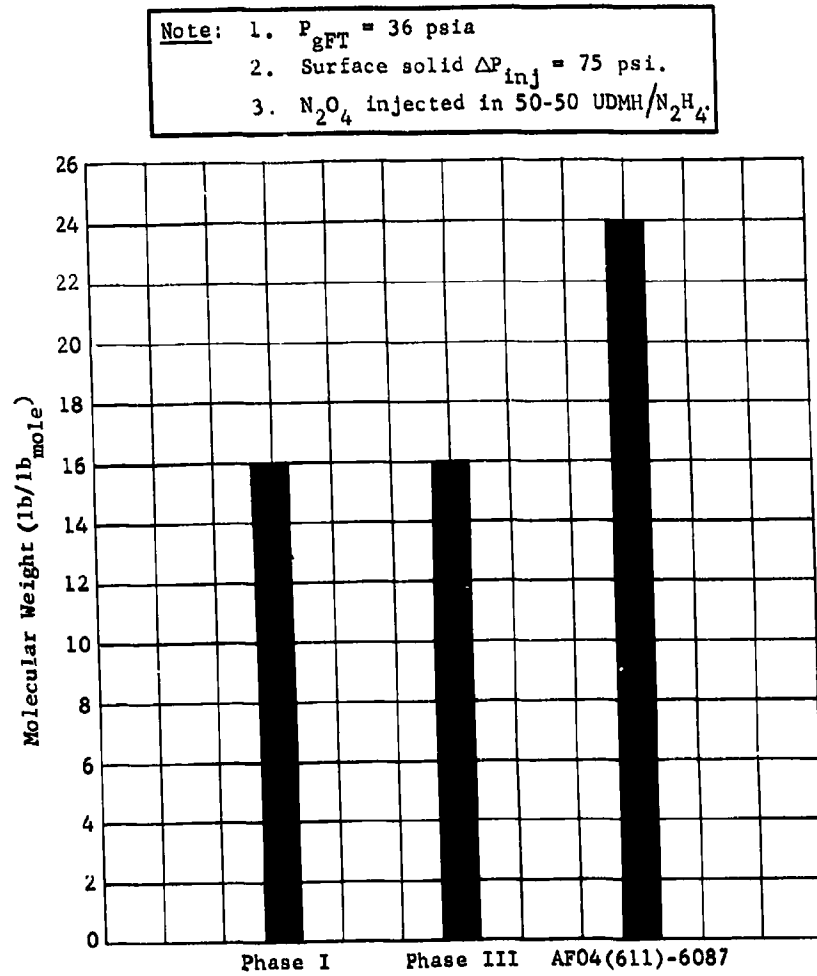
Fig. V-2 Molecular Weight Correlation - MTI in Fuel Tank
