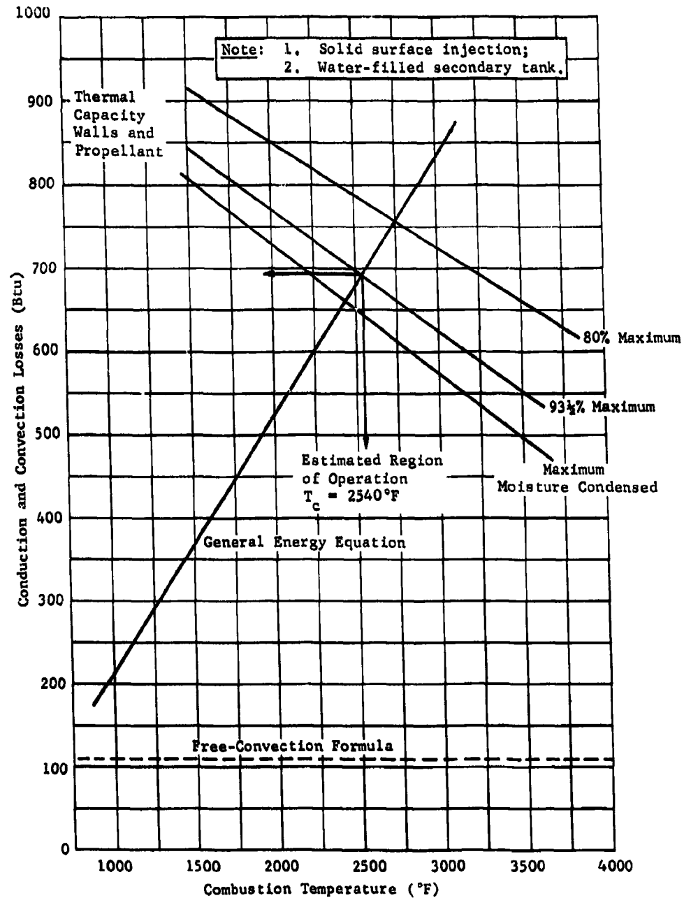
Fig. III-1 Research Test Tank Correlation of Fuel Tank Ullage Gas Thermodynamics
