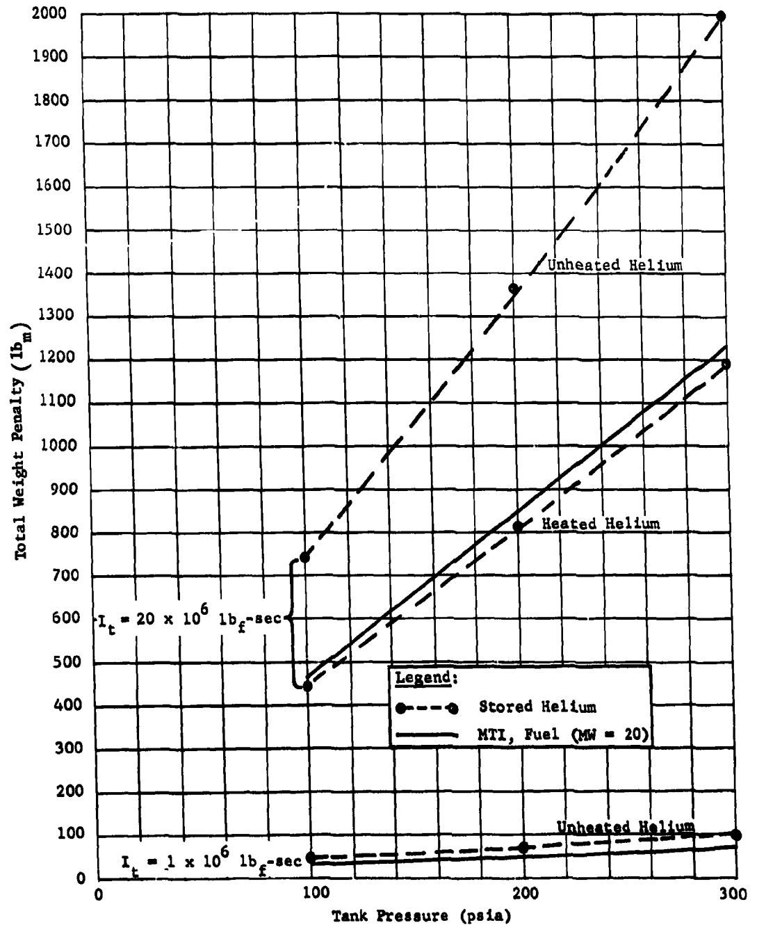
Fig. II-40 Comparison of MTI and Stored Helium Pressurization System Weights, Case VI, Space Vehicles, 1- to 30-day Space Storage
