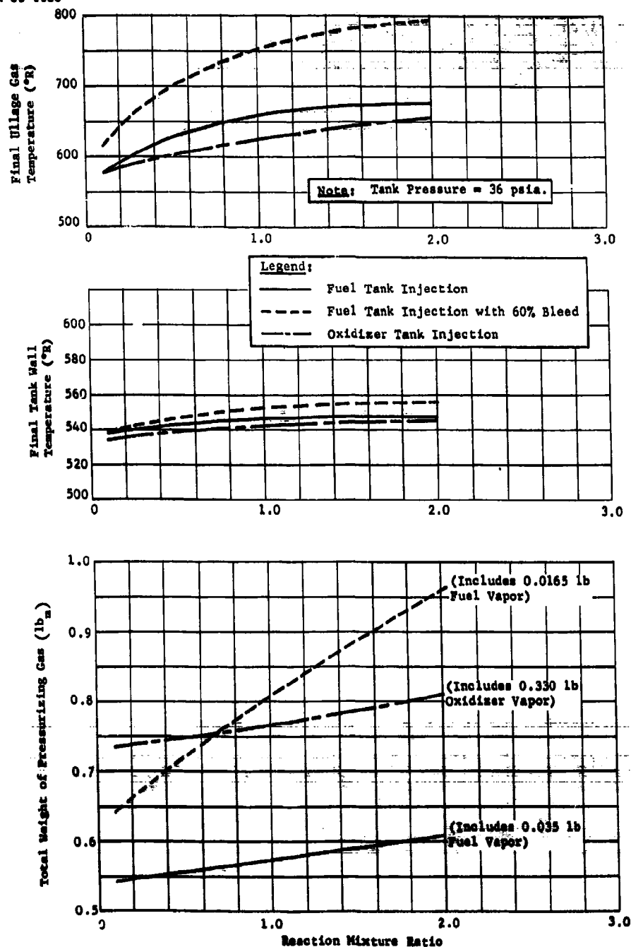
Fig. II-26 Theoretical Phase I System Performance for the Fuel or Oxidizer Tank
