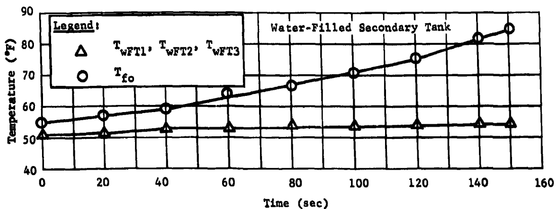
Fig. II-74 Primary Tank External Temperatures for Solid-Stream Subsurface Reagent Injection
