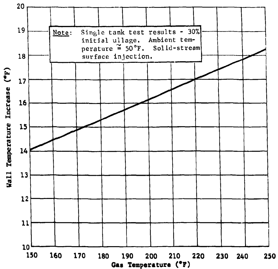
Fig. II-62 Fuel Tank Wall Temperature vs Ullage Gas Temperature
