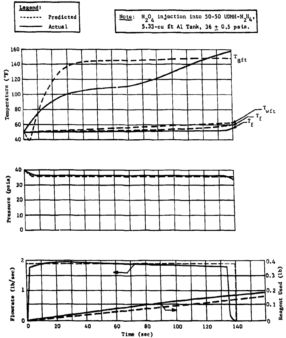
Fig. III-10 MTI Phase 1 Fuel Tank Performance
