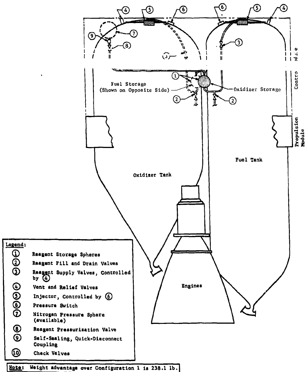
Fig. V-33 MTI Dual-Injection, Titan III Transtage, Nitrogen-Pressurized Reagent Supply (Configuration 3)
