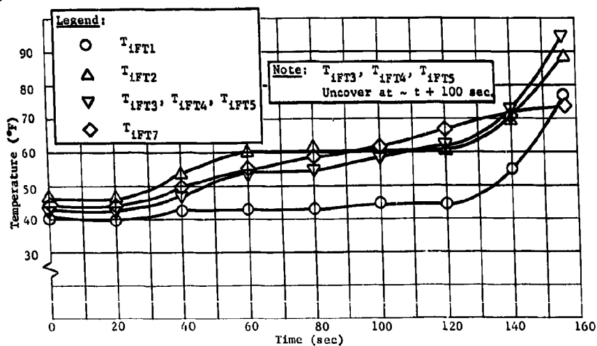
Fig. II-76 Primary Tank Internal Temperature Profiles with 15-deg Fan Spray Subsurface Reagent Injection
