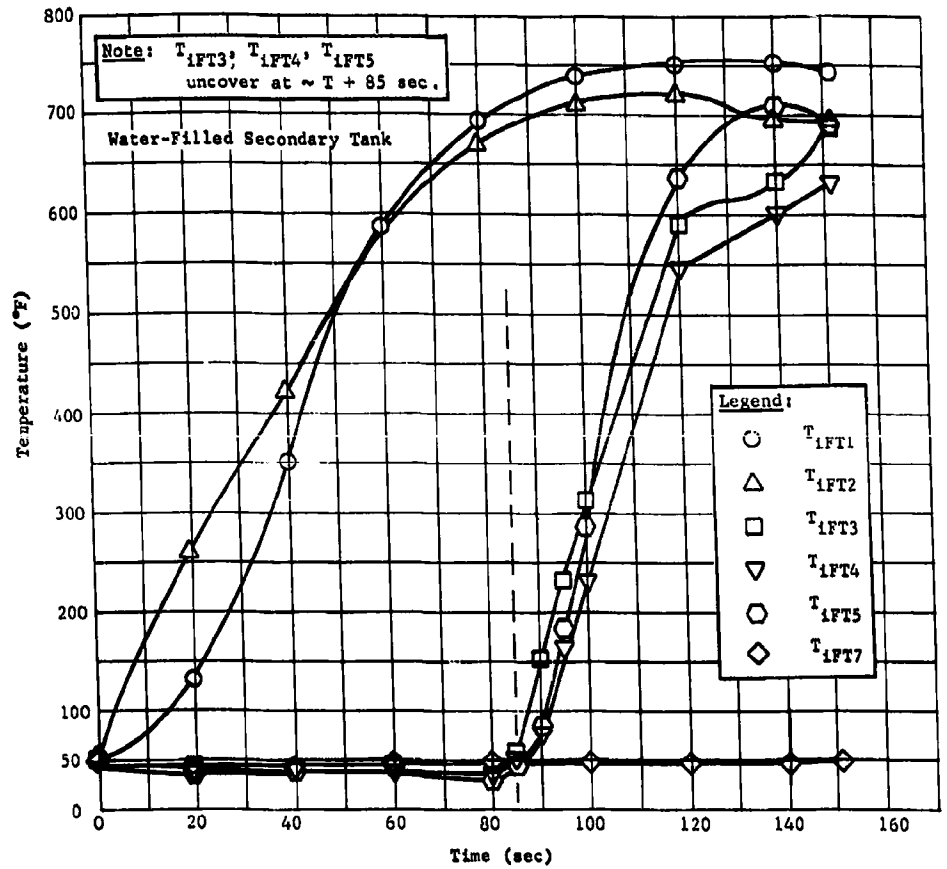
Fig. II-70 Primary Tank Internal Temperature Profiles with 15-deg Fan Spray Surface Reagent Injection
