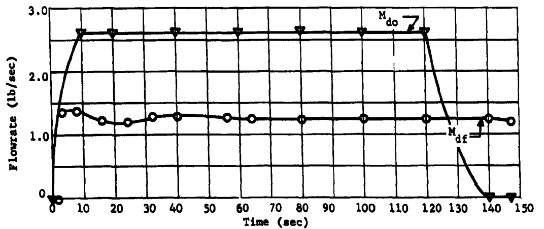
Fig. II-66 Pressurization System Performance Curves with Solid-Stream Surface Injection in Primary Tank
