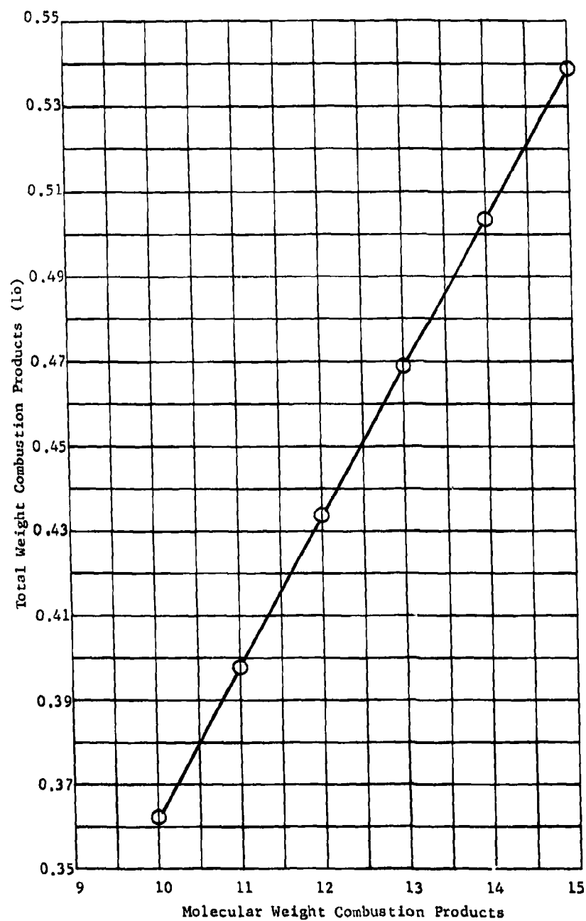
Fig. II-117 Phase I Pressurizing Gas Requirements vs Molecular Weight
