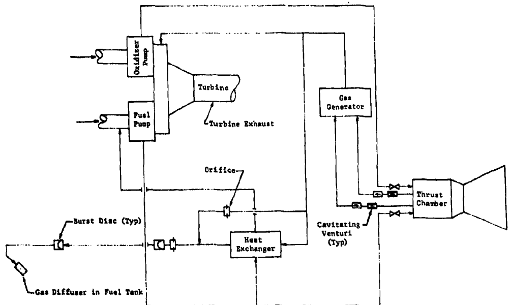
Fig. V-18 Existing Titan II Pressurization System, Stage II
