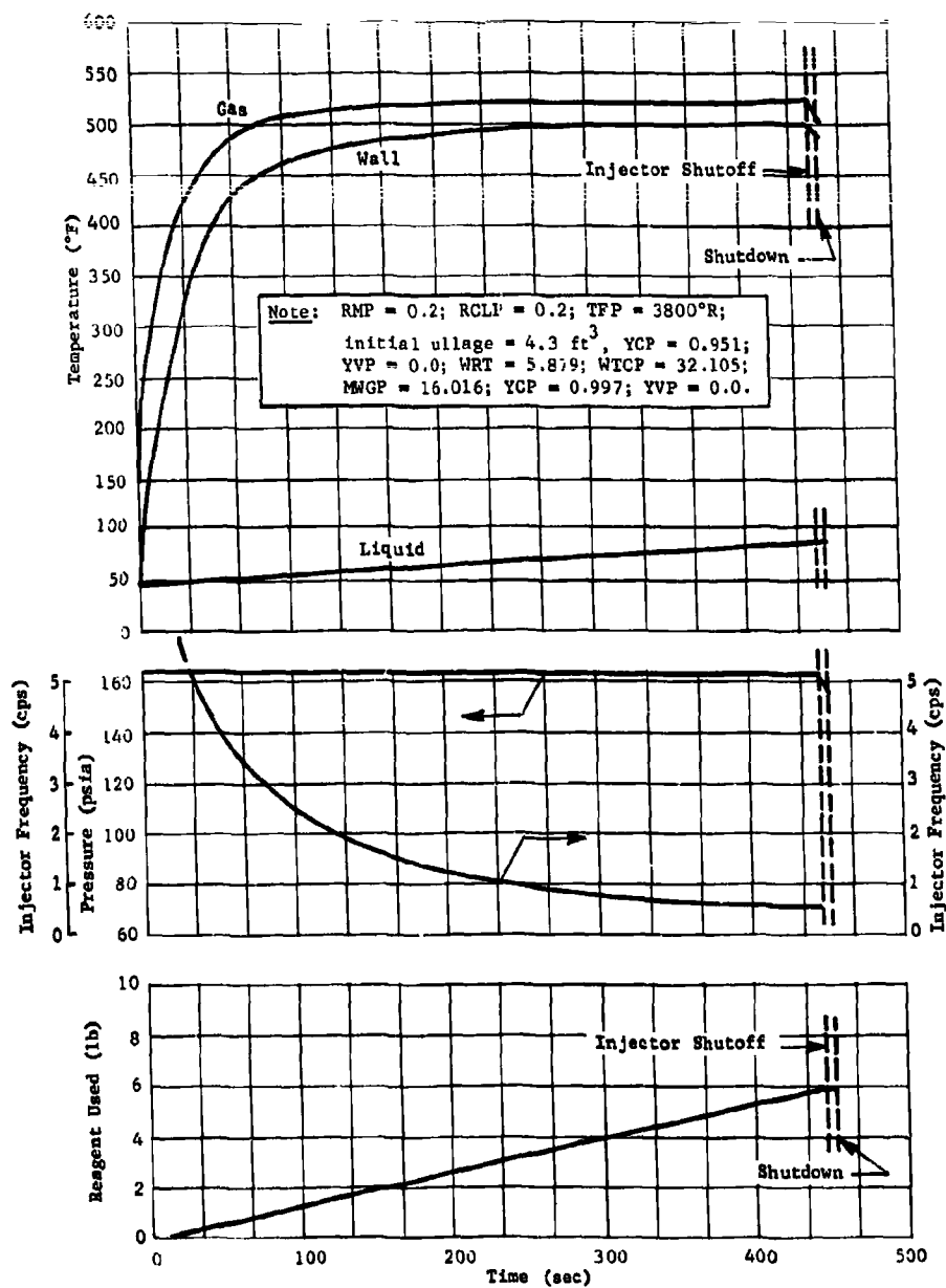
Fig. V-39 Titan III Transtage MTI Predicted Performance, Fuel Tank
