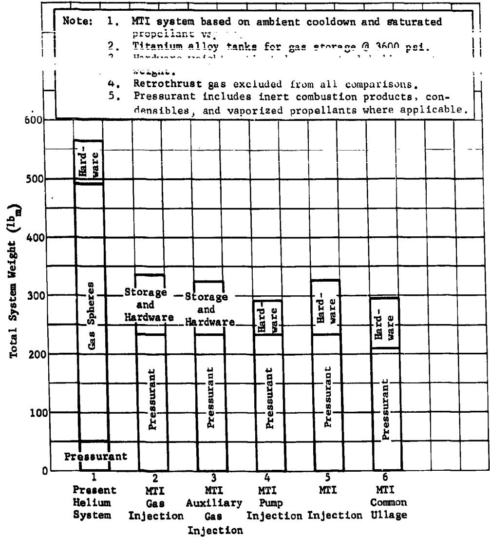
Fig. V-37 Comparative Pressurization System Weight, Titan III Transtage
