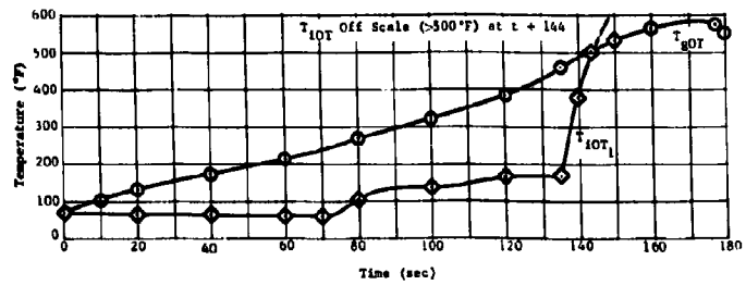
Fig. II-112 Parametric Test Oxidizer Tank System Performance at 200 psia
