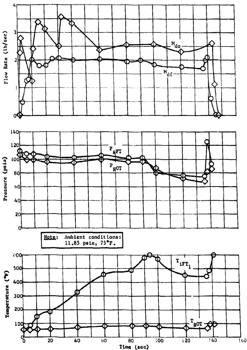
Fig. II-103 Parametric Test Common Ullage System Performance at 100 psia
