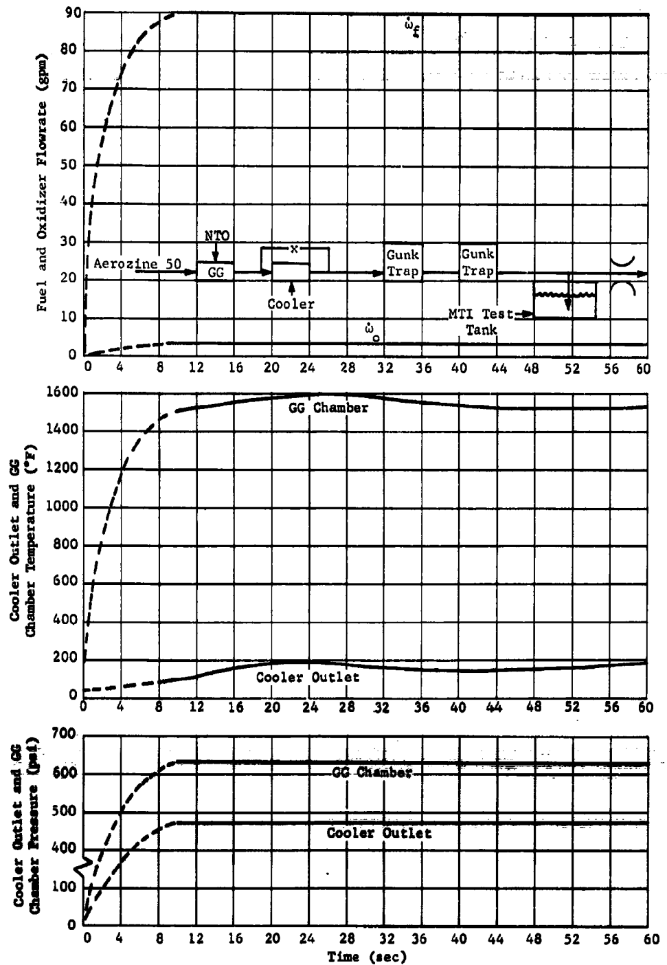
Fig. II-12 MTI Common Ullage Feasibility "Open Container" Test, Submerged Impingement
