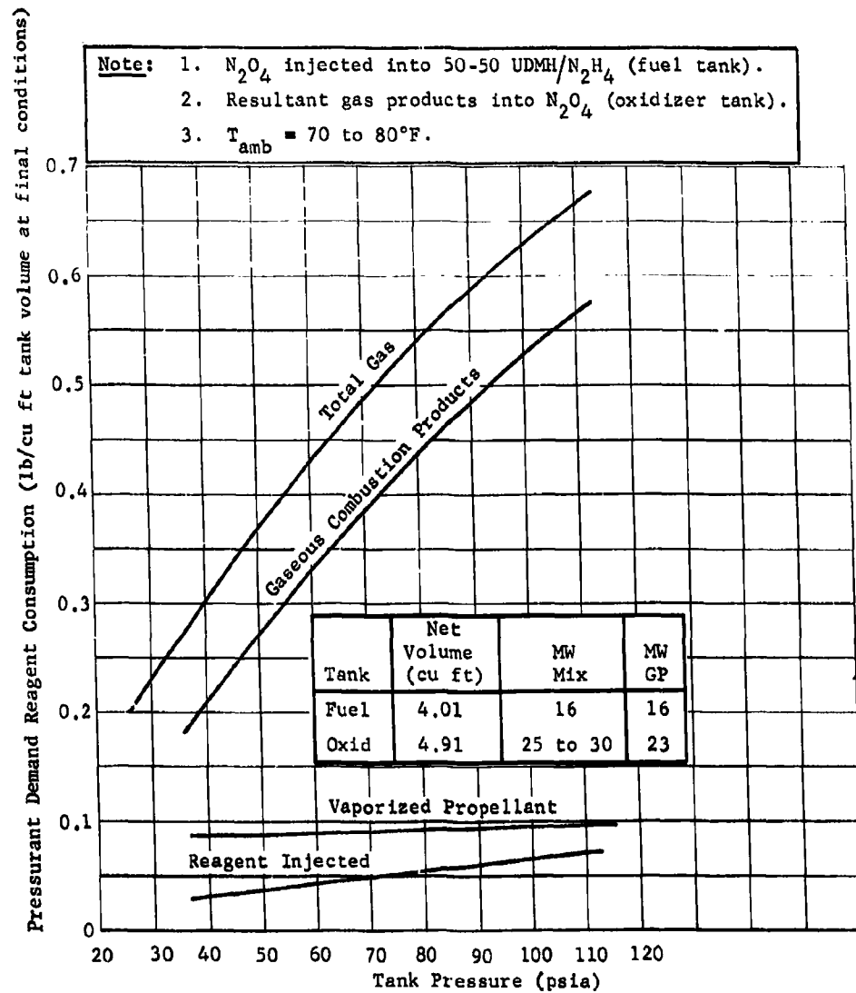
Fig. V-8 MTI Common Ullage Pressurant Weight
