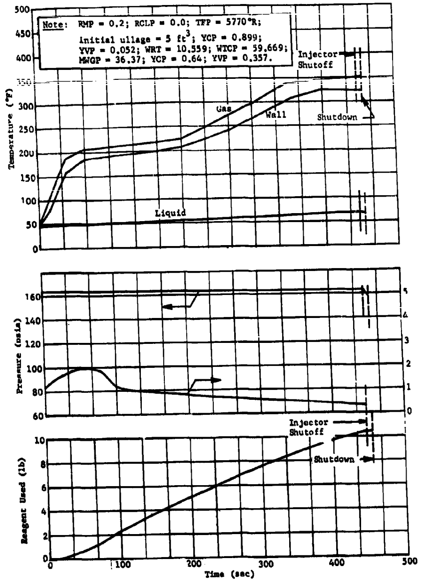
Fig. V-38 Titan III Transtage MTI Predicted Performance, Oxidiser Tank
