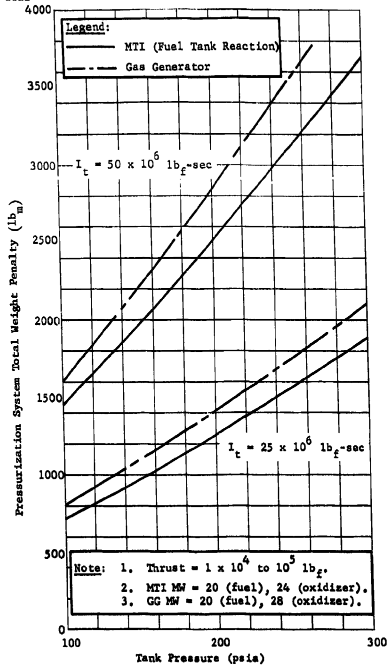
Fig. II-36 MTI vs Gas Generator Pressurization Systems, Case V, Limited Space Vehicle, 1 Month Storage
