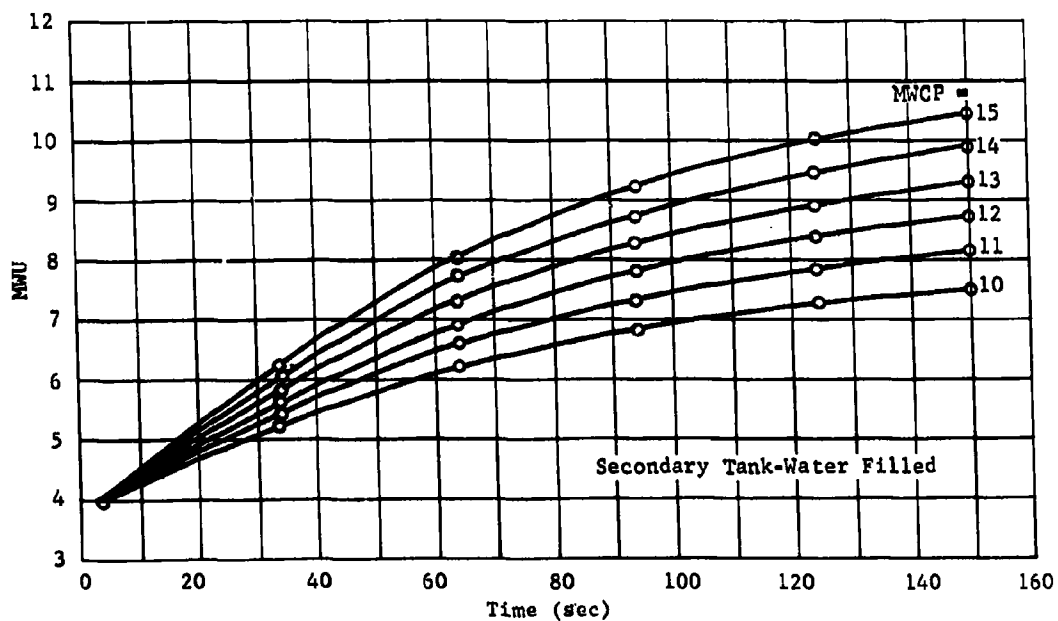
Fig. II-116 Phase I Predicted Pressurizing Gas Dilution
