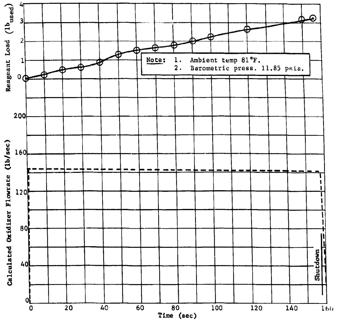
Fig. IV-20 Run 6 Phase III Oxidizer Tank Pressurization and Propellant Flowrates
