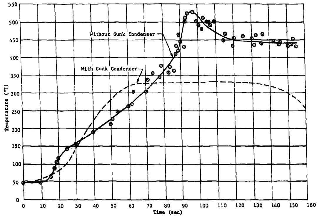
Fig. II-80 Secondary Tank Gas Temperature Profile with Surface Gas Impingement on Oxidizer
