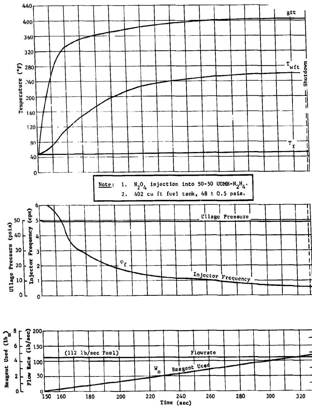
Fig. V-28 MTI Titan II Stage II Predicted Performance
