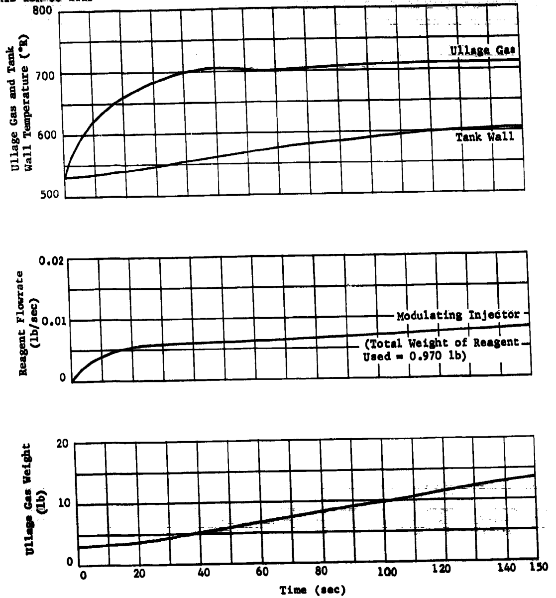
Fig. II-29 Phase III Fuel Tank Predicted Performance for Mixture Ratio of 0.1 and Pressure of 36 psia
