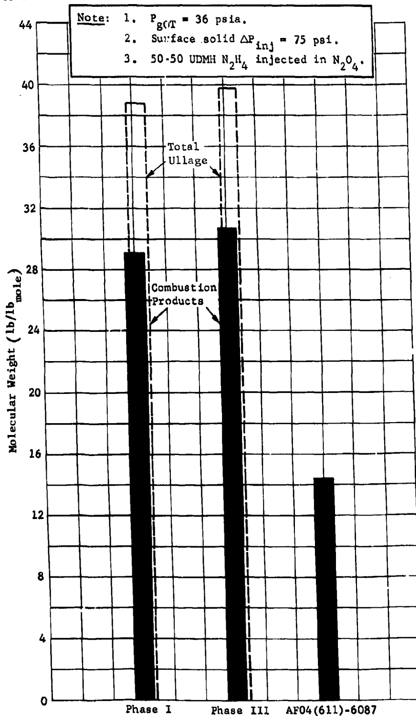
Fig. V-1 Molecular Weight Correlation, MTI in Oxidizer Tank
