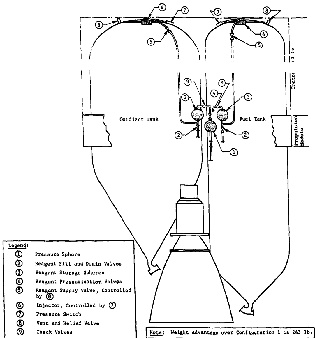
Fig. V-32 MTI Dual-Injection, Titan III Transtage, Gas-Pressurized Reagent Supply (Configuration 2)
