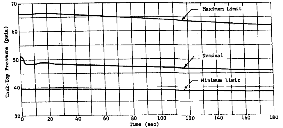
Fig. V-21 Flight Tank Pressure, Stage II Fuel Tank
