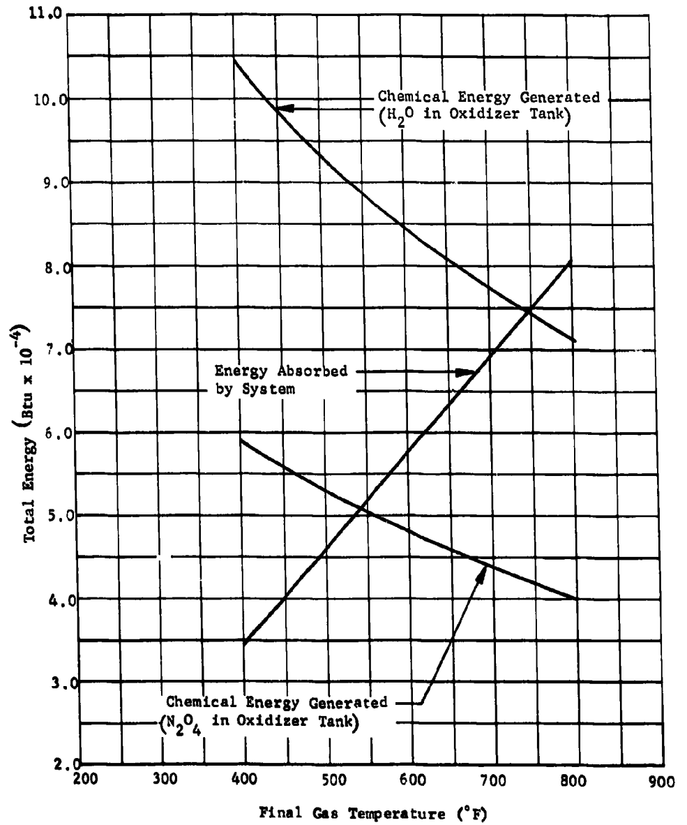
Fig. III-5 Phase III Energy Balance
