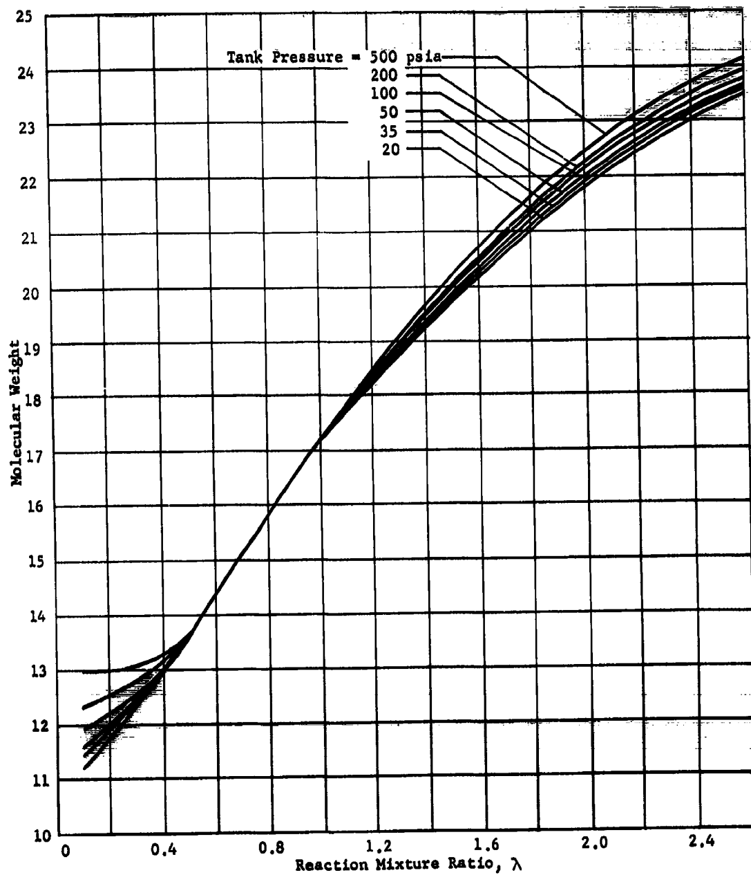
Fig. II-16 Molecular Weight of Combustion Products ( N_2O_4 /Aerozine 50)
