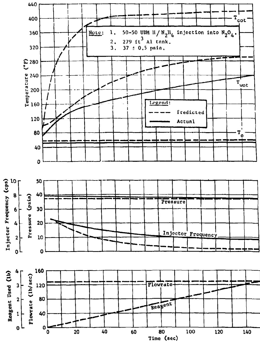
Fig. V-10 Phase III MTI Oxidizer Tank Performance
