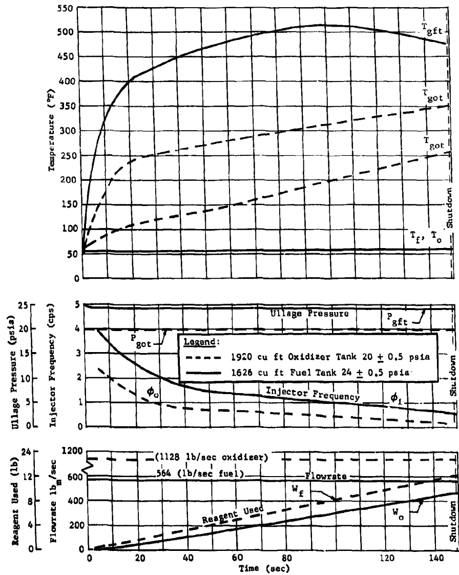
Fig. V-27 MTL Titan II Stage I Predicted Performance
