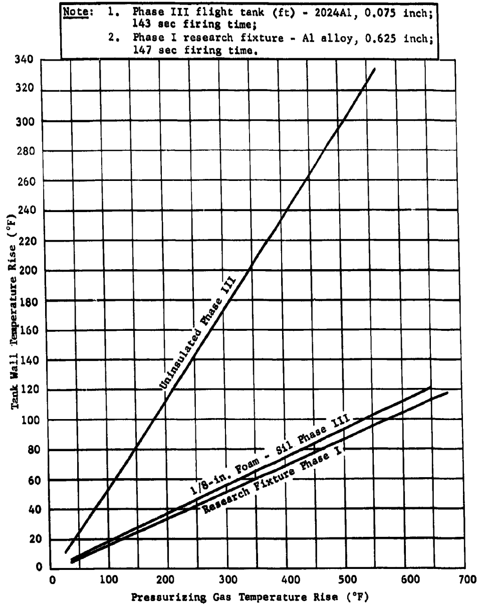
Fig. III-2 Predicted Tank Wall Heating
