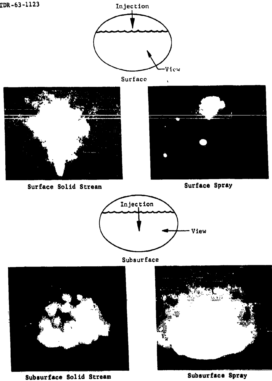
Fig. II-78 Combustion Photographs - MTI of N_2O_4 into a 50-50 Mixture of UDMH and N_2H_4
