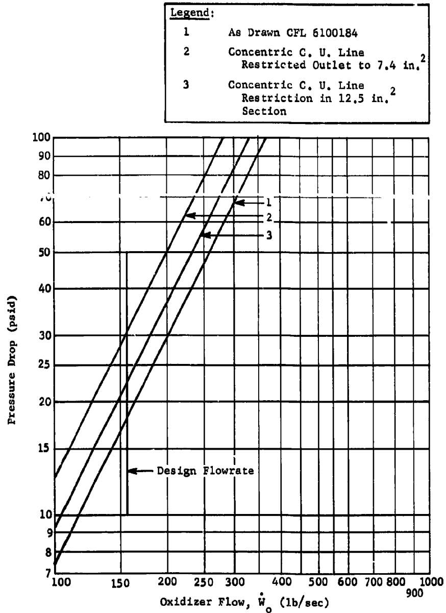
Fig. III-31 Calculated Pressure Drop MTI Phase III Oxidizer System
