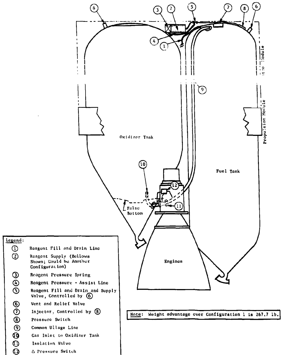
Fig. V-36 MTI Single-Tank Injection, Common Ullage (Configuration 6)
