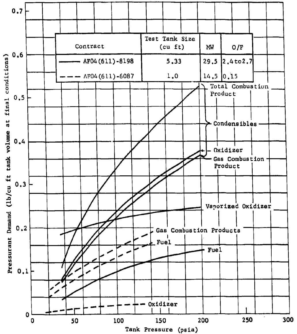
Fig. V-6 MTI Pressurant Weight, Oxidizer Tank, Comparison of Results from AF04(611)-6087 and AF04(611)-8198
