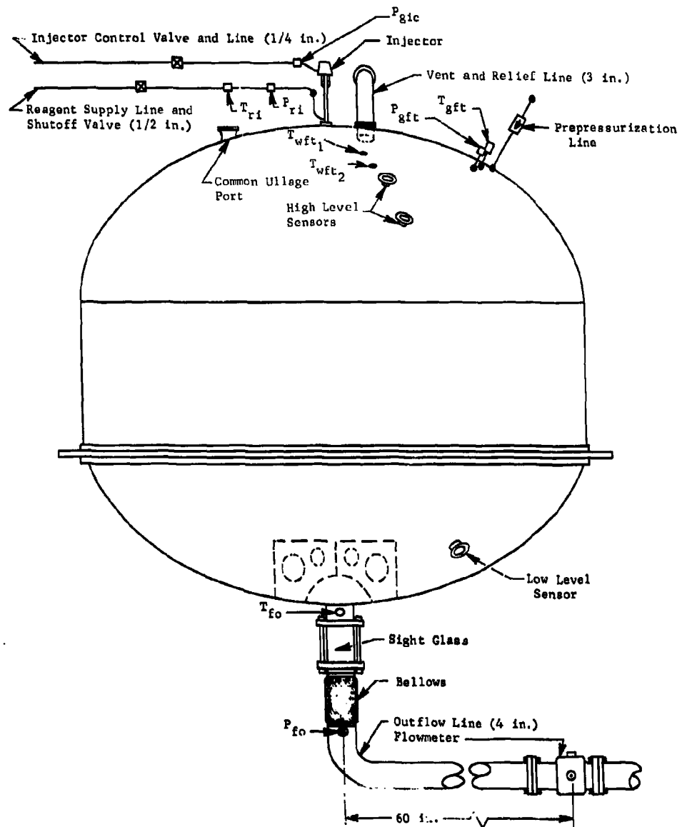
Fig. IV-3 Instrumentation Locations, Phase III Fuel Tank-Side View
