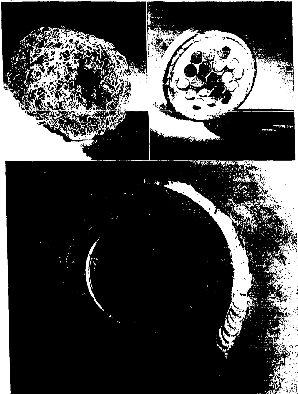
Fig. II-99 Failed Demister Parts Resulting from Faulty Injector
