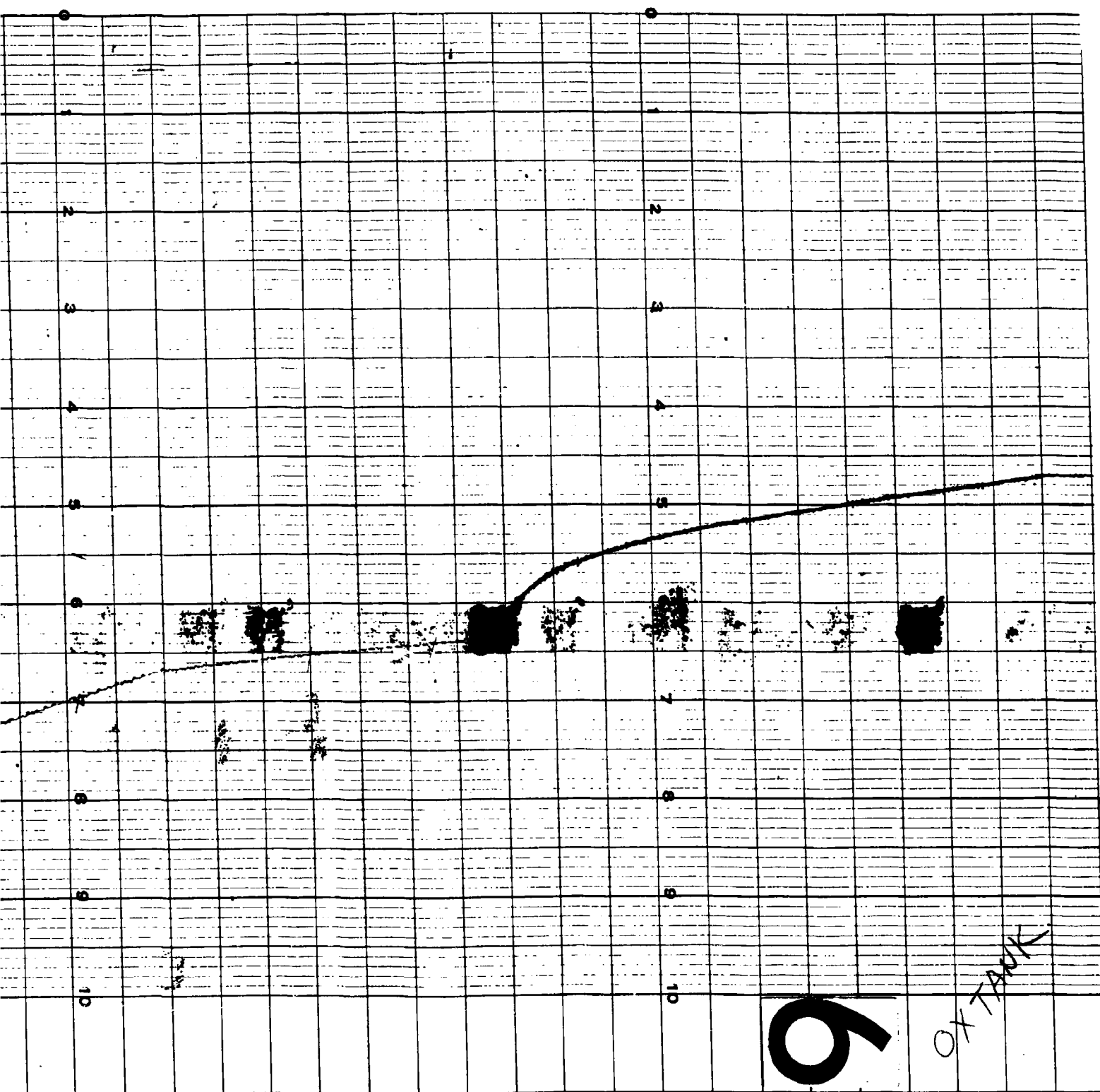
Fig. IV-21 Actual Phase III Pressure Trace with 5% Initial Ullage, Oxidizer Tank IV-39 and IV-40
