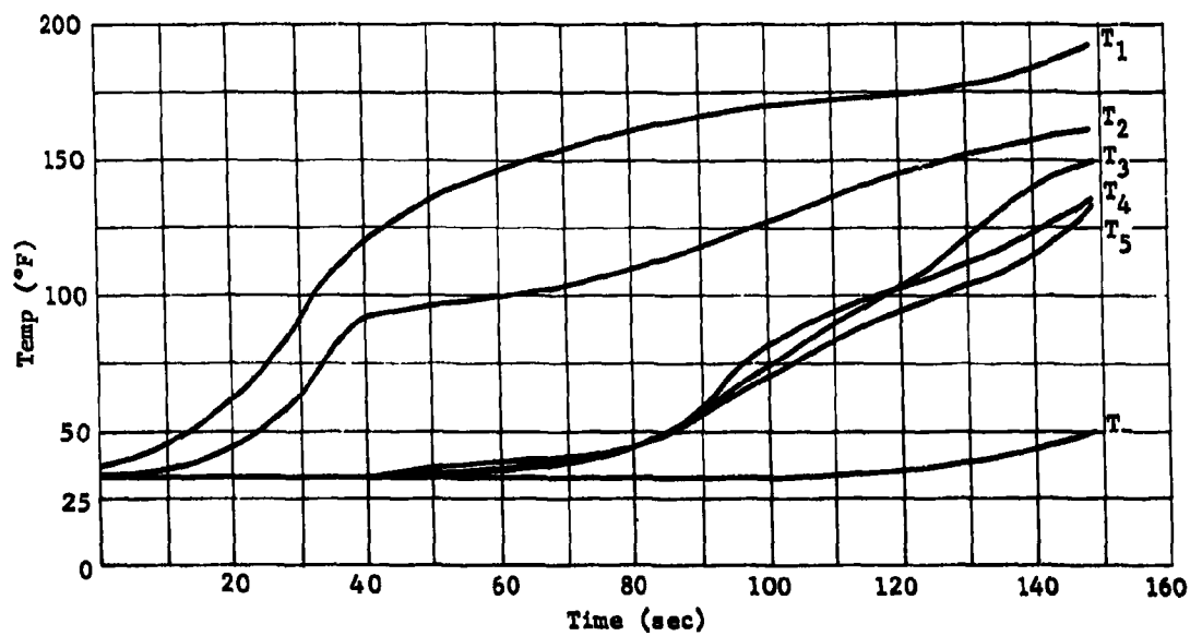
Fig. II-55 Fuel Tank Internal Temperature Profile
