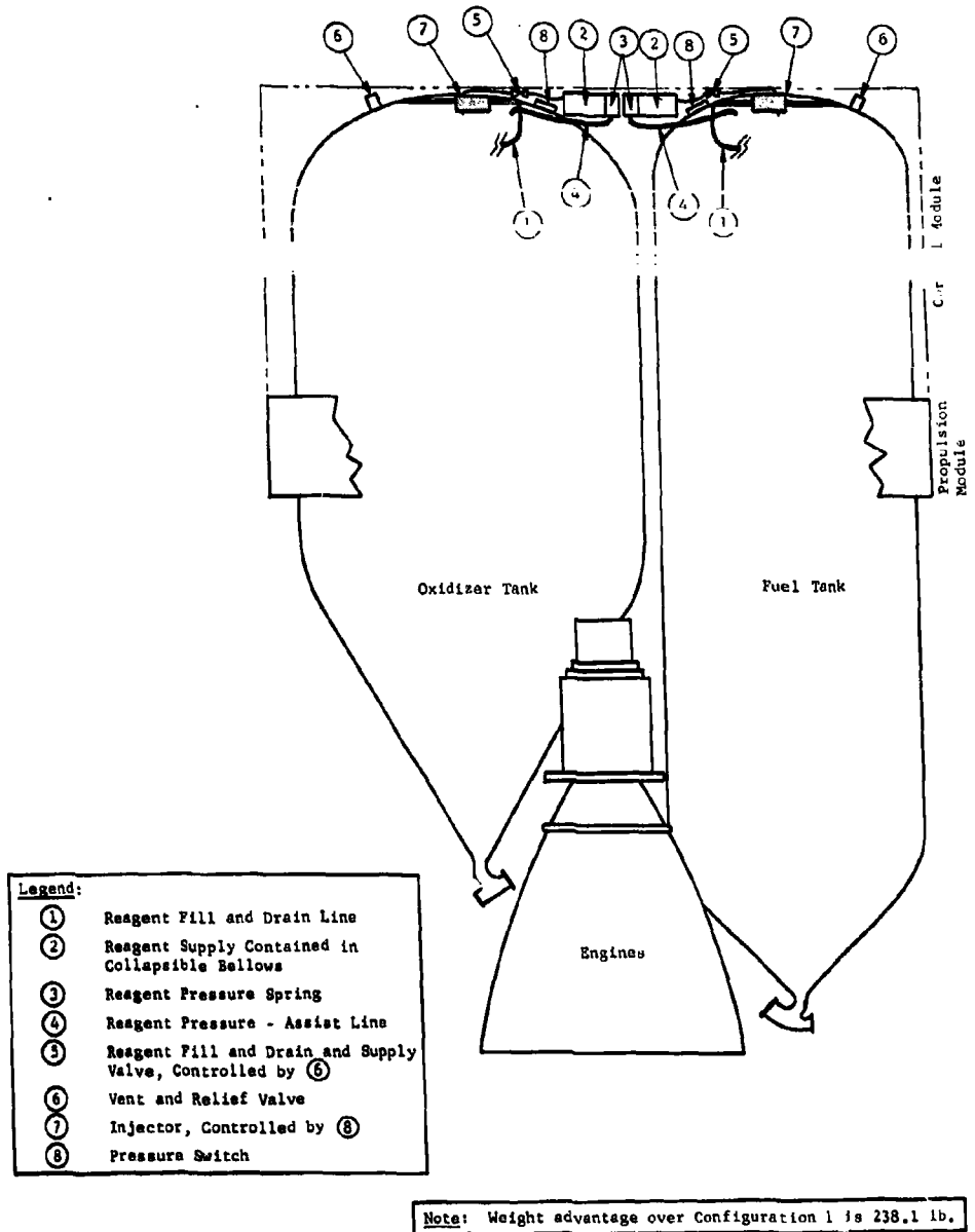
Fig. V-35 MTI Dual-Injection, Titan III Transtage, Mechanically Pressurized Reagent Supply (Configuration 5)
