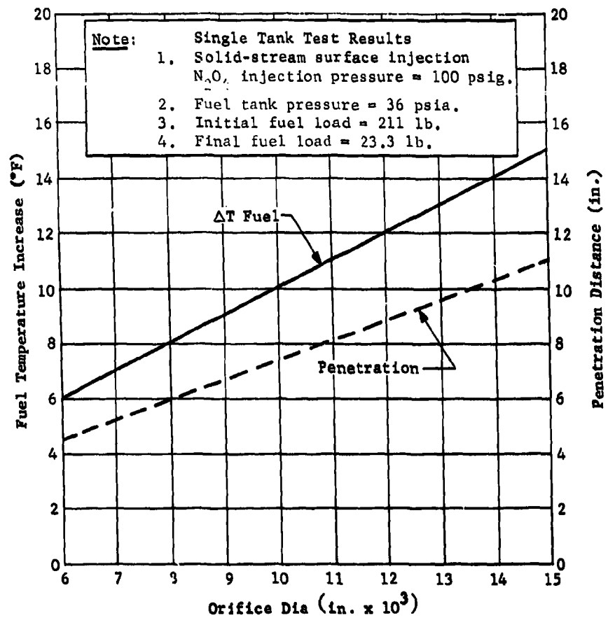
Fig. II-60 Injector Orifice Size Effects on Fuel Combustion
