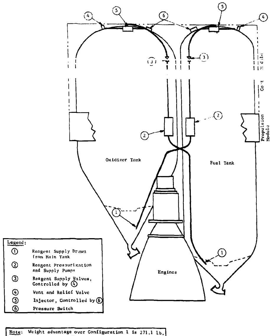
Fig. V-34 MTL Dual-Injection, Titan III Transtage, Pump-Fed, Main Tank Reagent Supply (Configuration 4)
