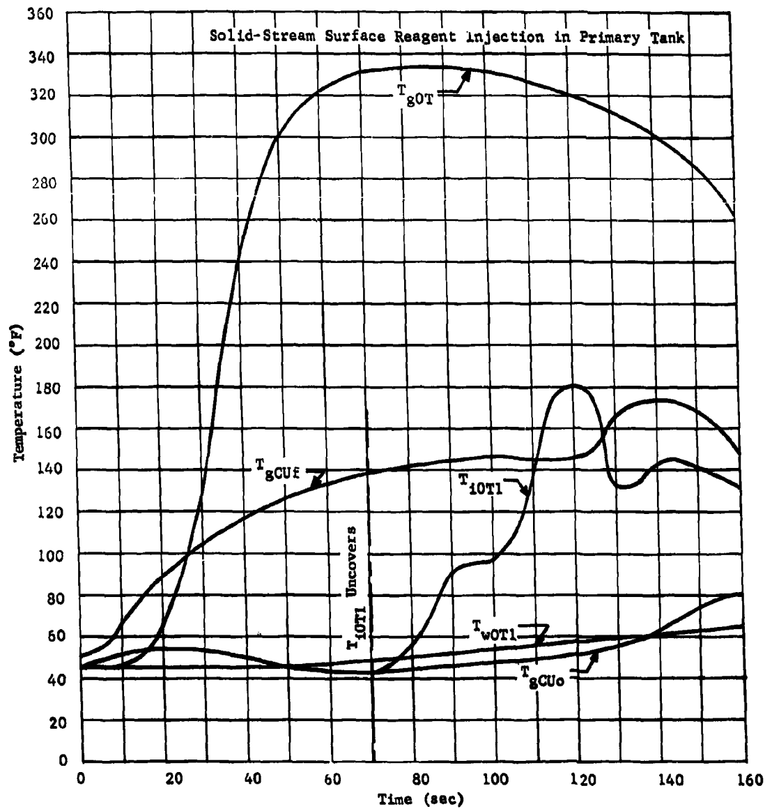
Fig. II-84 Temperatures in Oxidizer Tank with Surface Gas Impingement and Gunk Condenser
