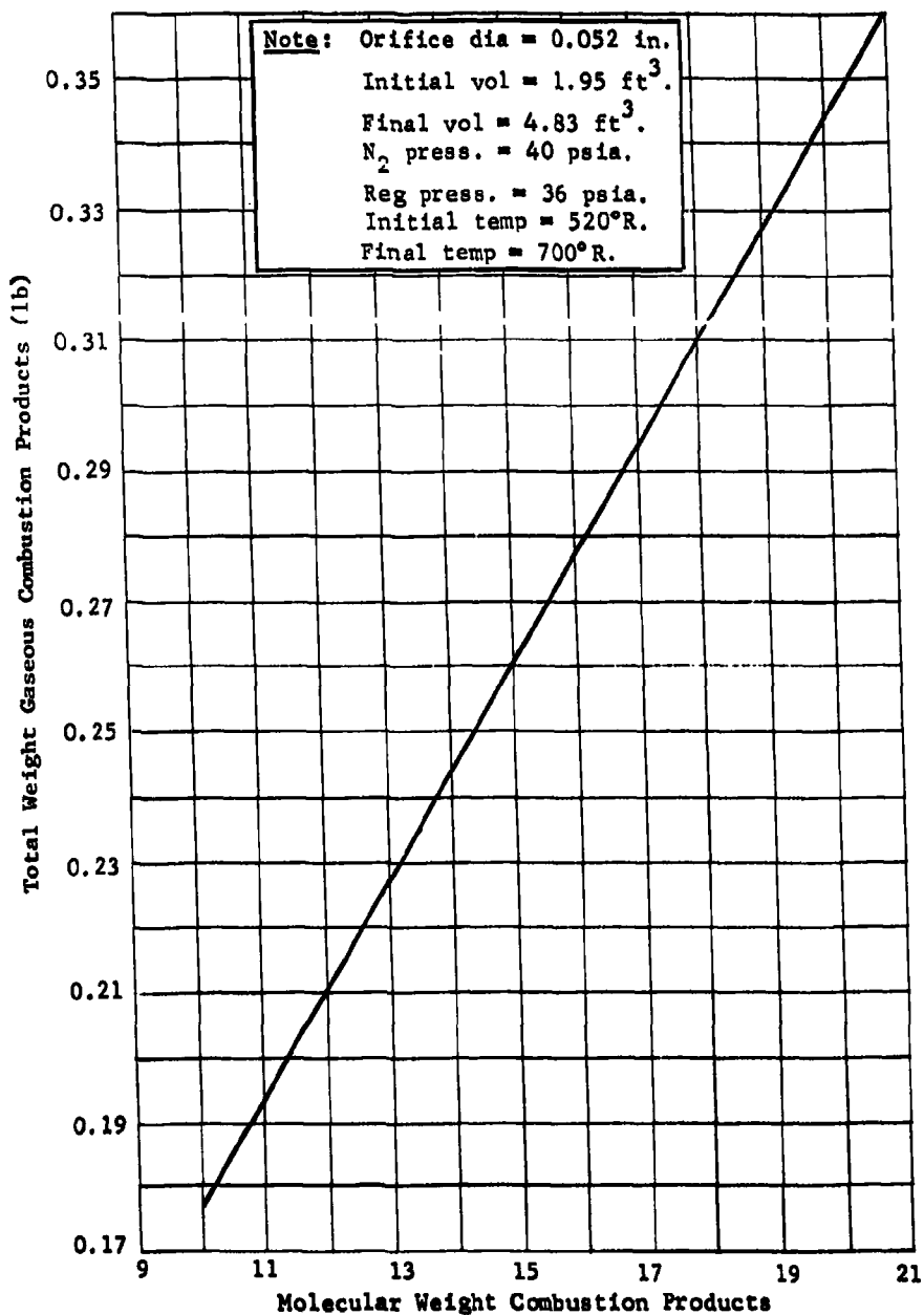
Fig. II-59 MTI Gaseous Combustion Products Total Weight vs Molecular Weight for the Small-Scale Single-Tank System
