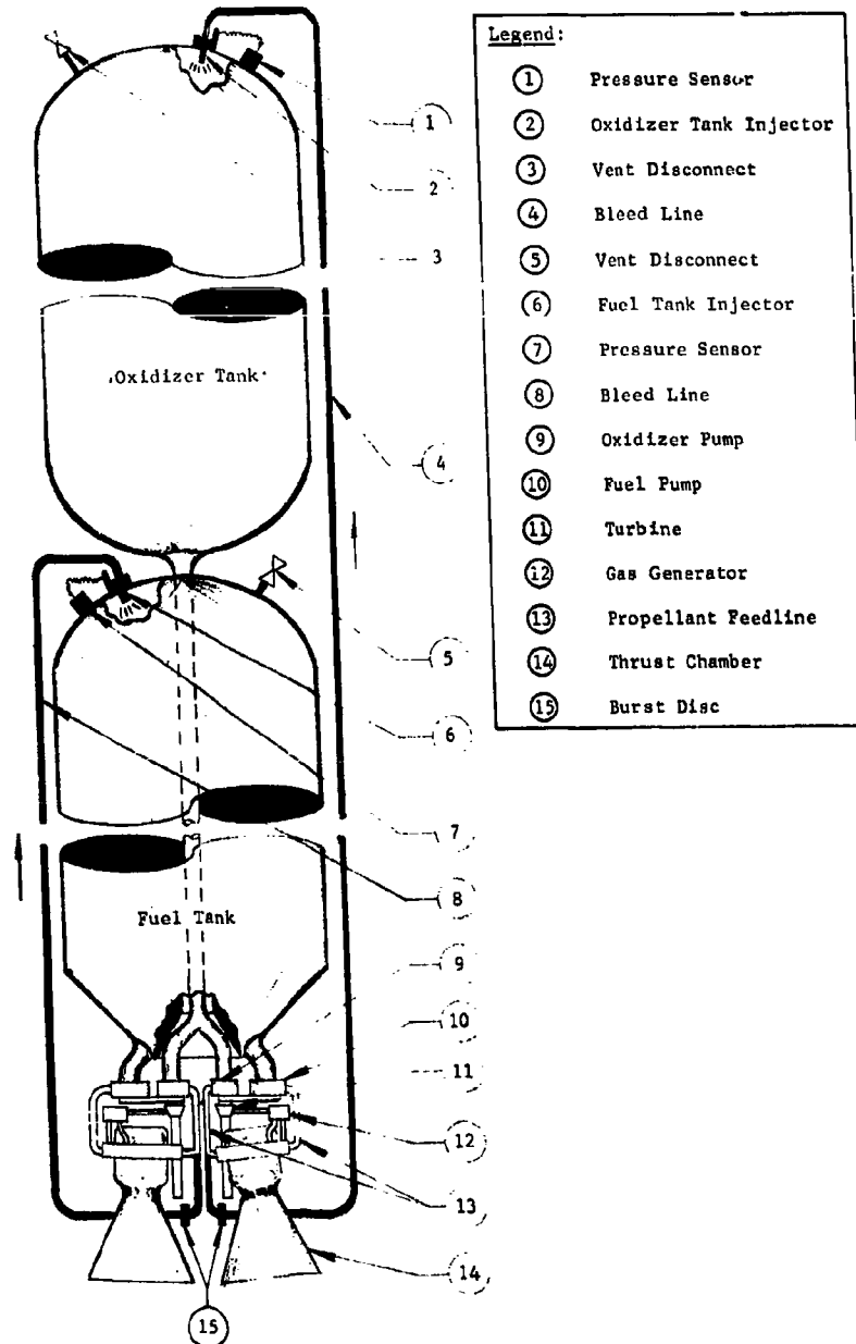
Fig. V-23 Pulse-Type MTI with Turbopump Bleed
