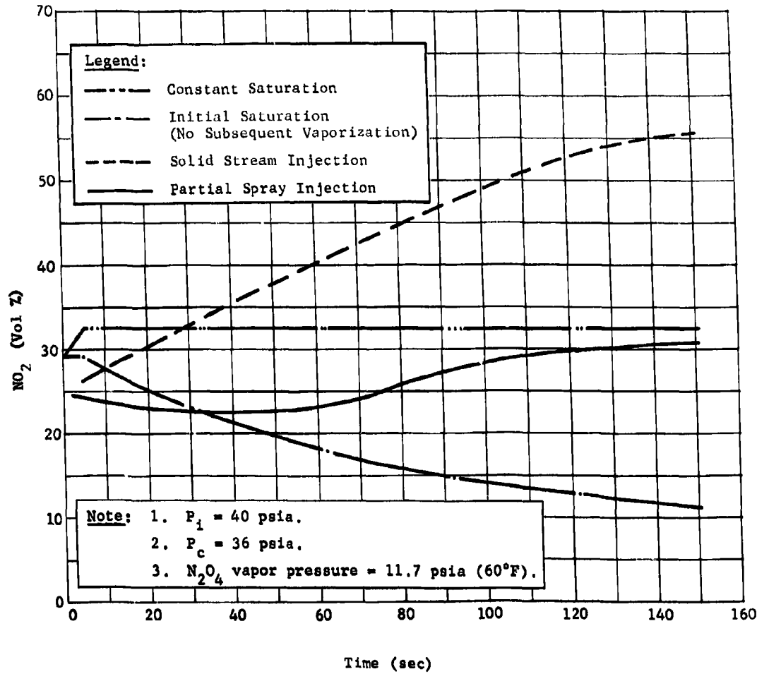
Fig. II-122 Oxidizer Tank Ullage Saturation with NO_2
