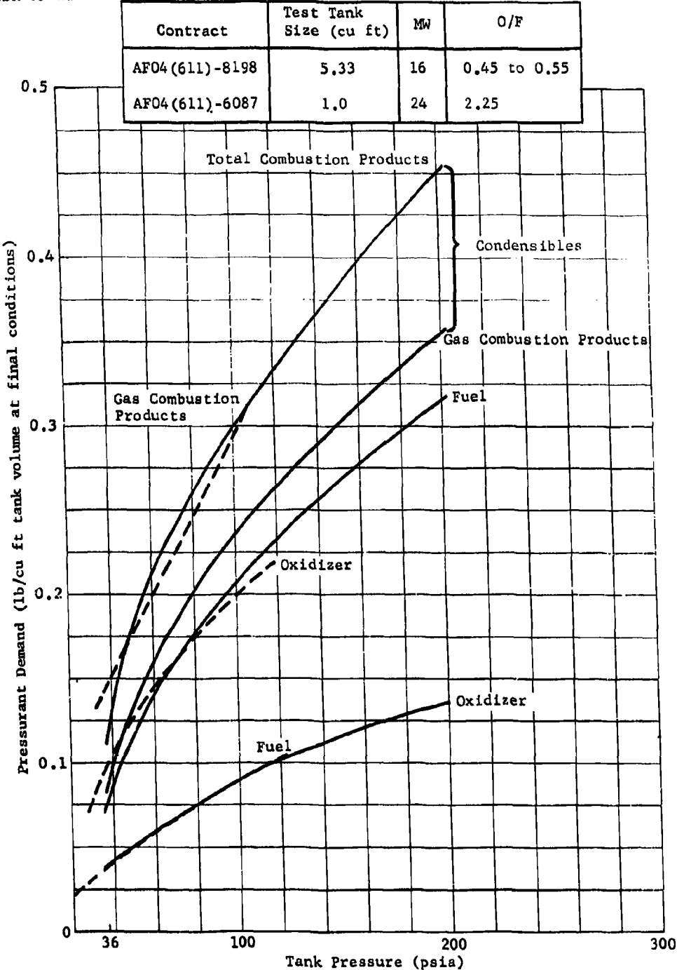
Fig. V-7 MTI Pressurant Weight, Fuel Tank, Comparison of Results from AF04(611)-6087 and AF04(611)-8198
