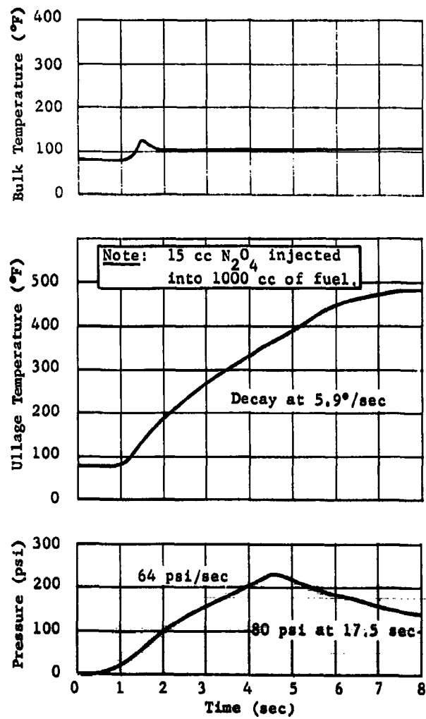
Fig. II-14 MTI "Bomb" Test, Run 1
