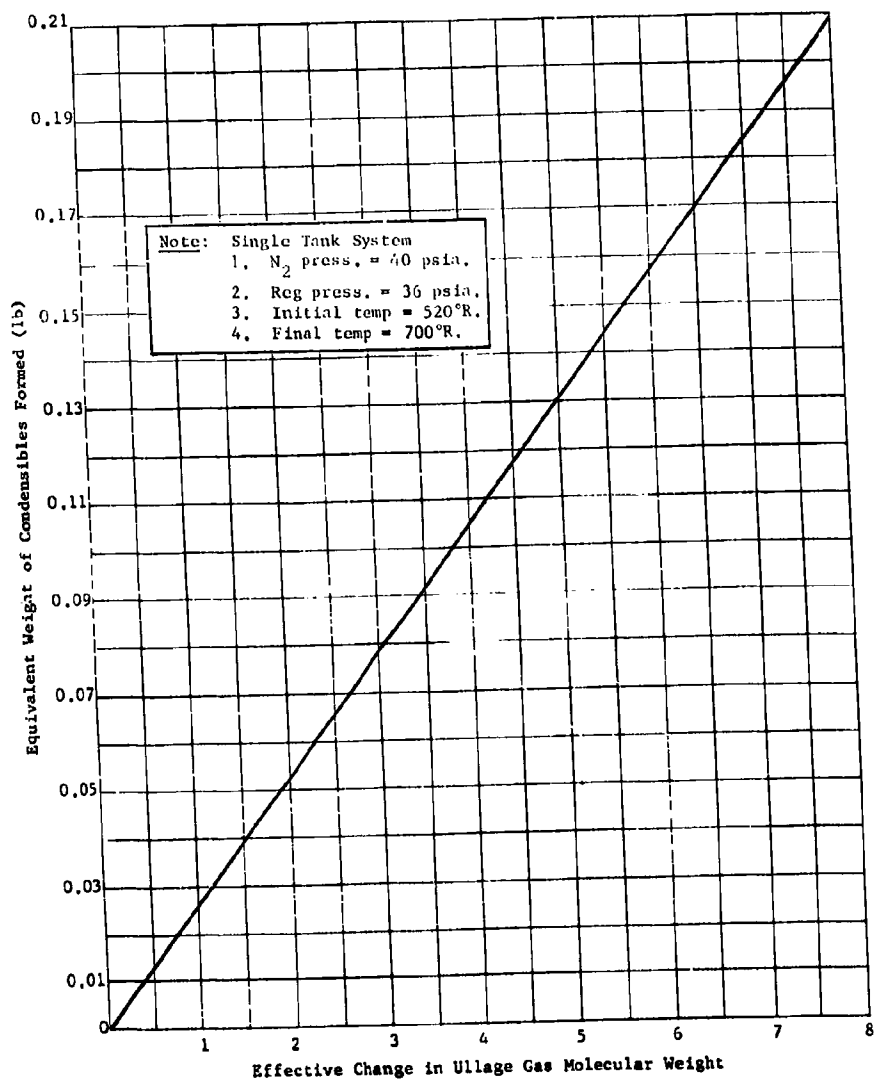
Fig. II-125 Equivalent Ullage Gas Weight as a Function of Changes in Molecular Weight
