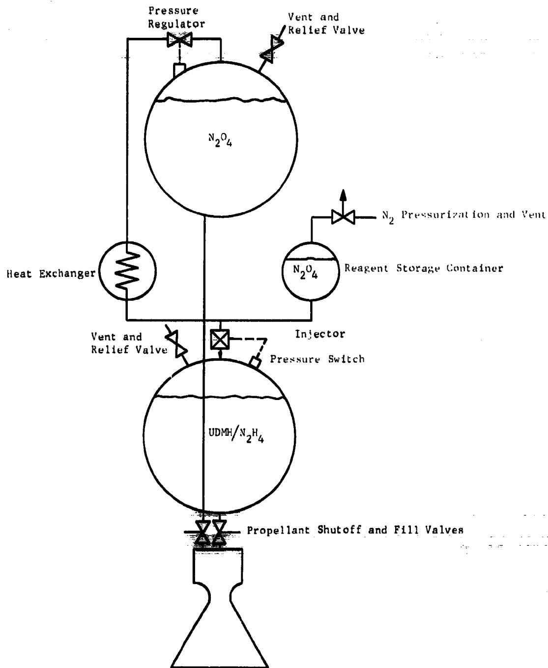
Fig. II-7 Hybrid MTI Pressurization System with Pneumatically Pressurized Remote Reagent Storage and Evaporated Propellant, Pressure-Fed Engine
