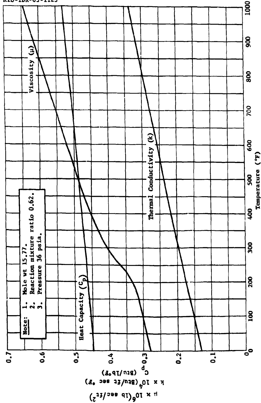
Fig. III-17 Properties of Combustion Gases, Fuel Tank Reaction, N_2O_4 Injection
