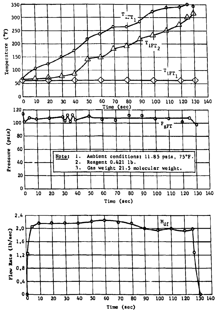
Fig. II-106 Parametric Test Fuel Tank System Performance at 100 psia
