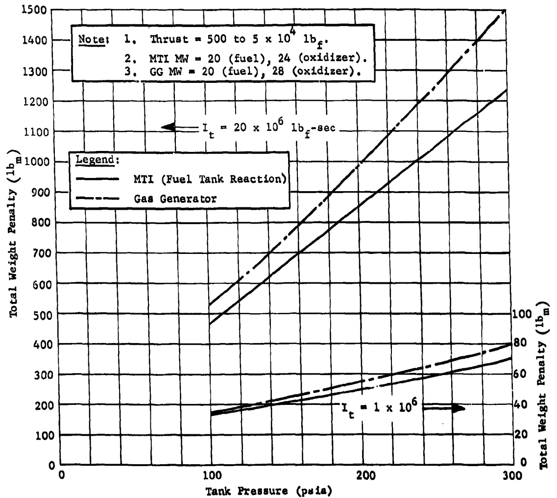
Fig. II-37 MTI vs Gas Generator Pressurization Systems, Case VI, Space Vehicle, Indefinite Storage
