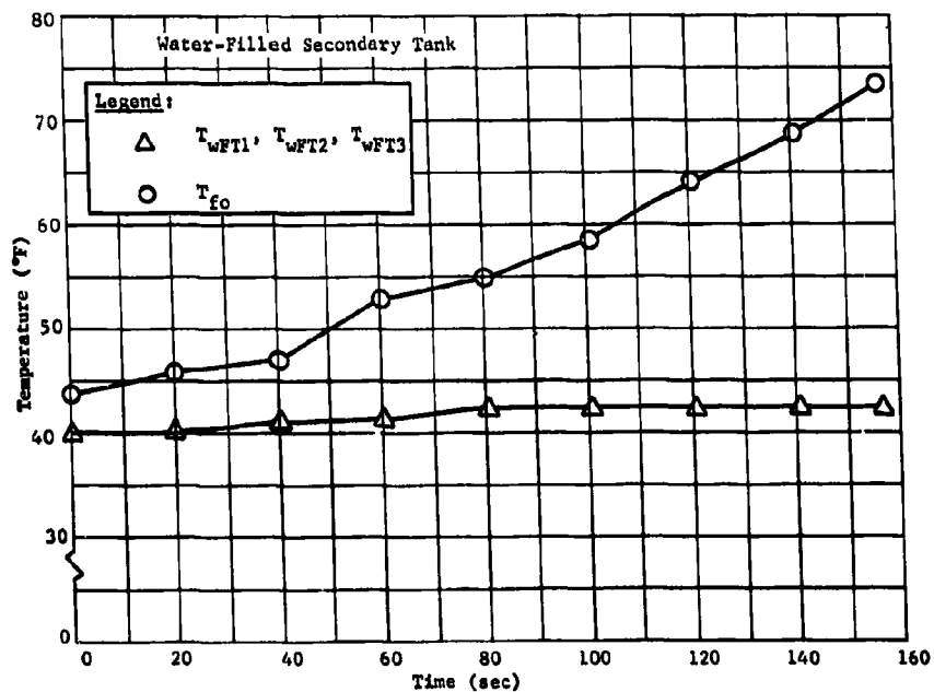
Fig. II-77 Primary Tank External Temperature for 15-deg Fan Spray Subsurface Reagent Injection
