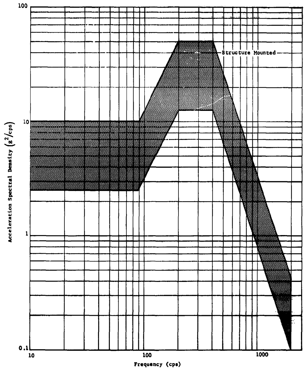
Fig. II-3 Random Vibration Design Criteria for an MTI Pressurisation System, Flight Environment
