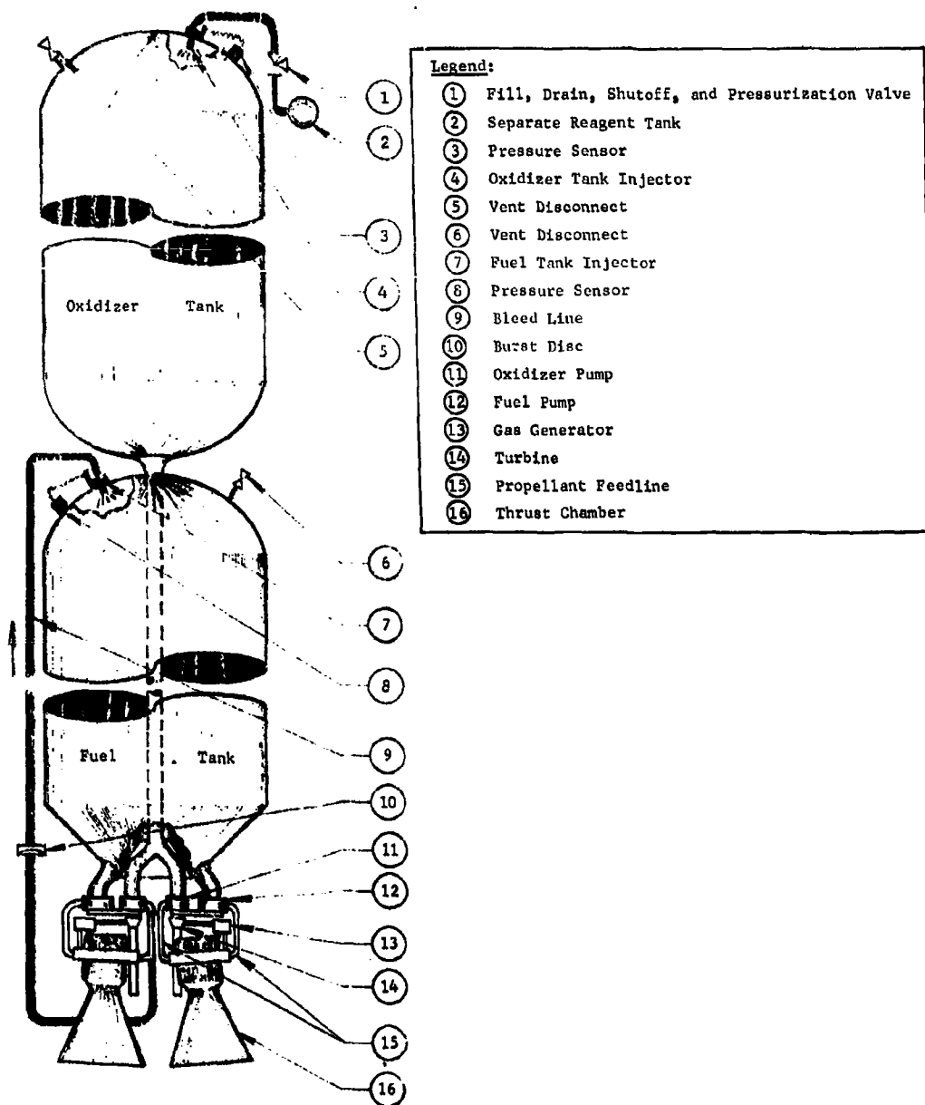
Fig. V-24 Pulse-Type MTL, Turbopump Bleed Fuel Tank and Separate Reagent Supply Oxidizer
