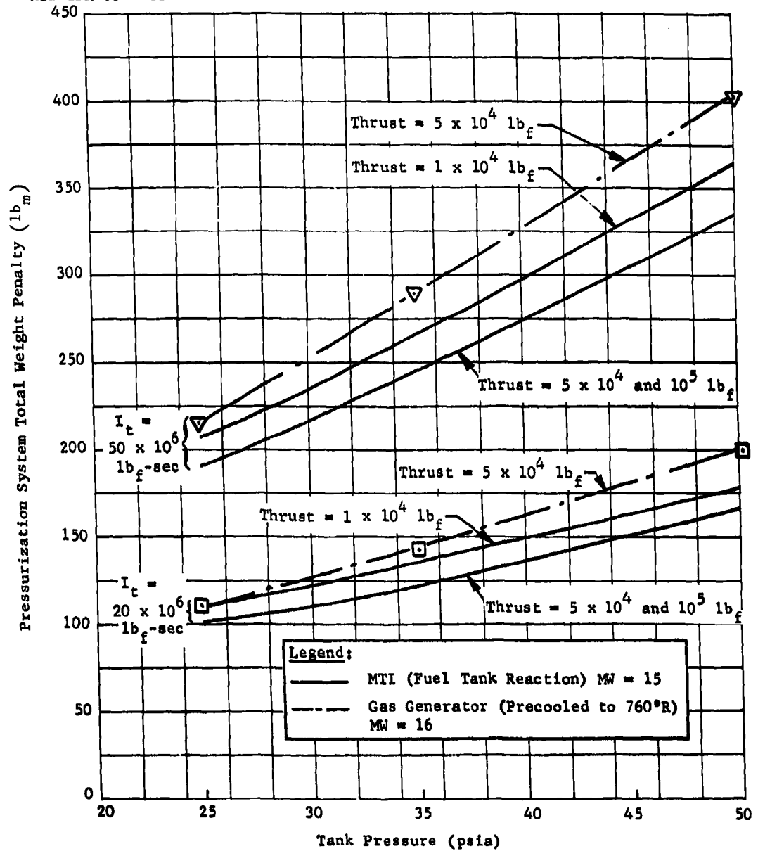
Fig. II-33 MTI vs Gas Generator Pressurization System, Case II, Sustainer Vehicle
