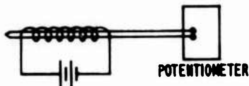
Figure 9. Temperature-Compensated, Contact Thermocouple.
