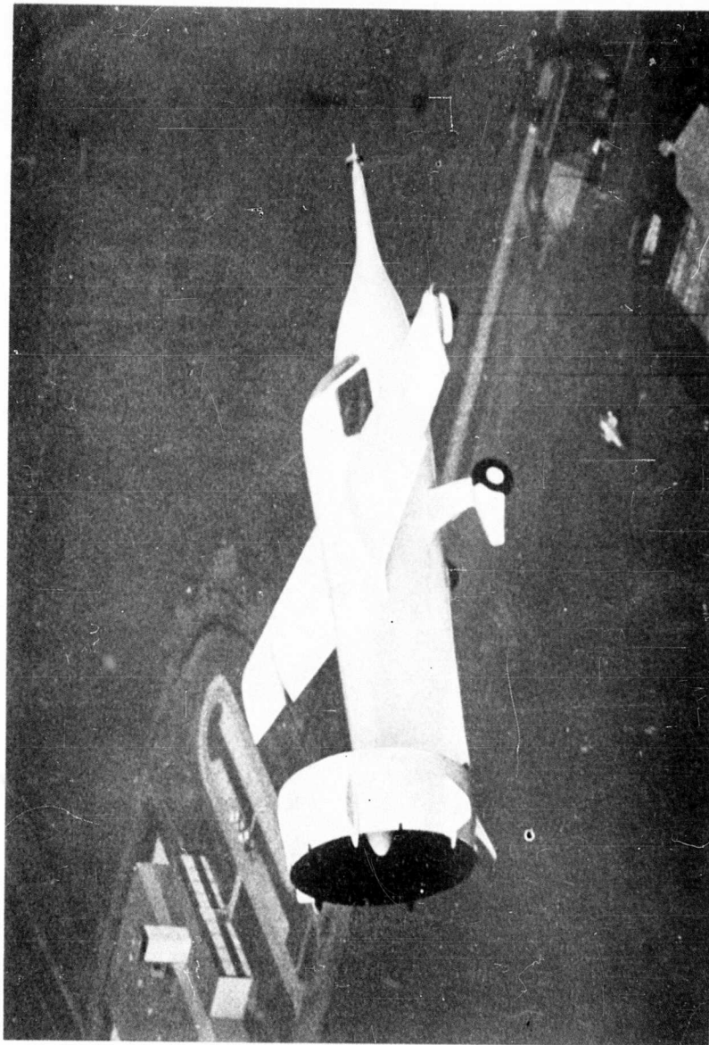
Figure 2. Flight View of MARVELETTE XAZ-1.
