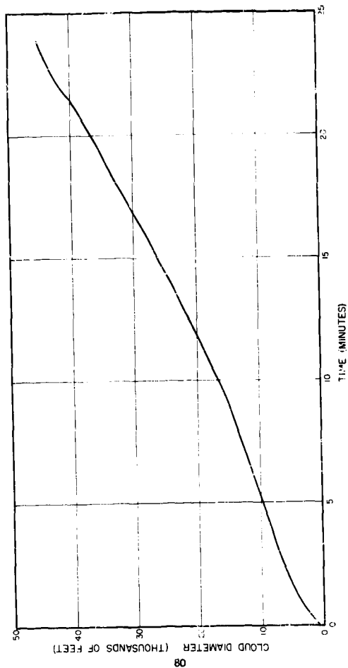
Fig. 3.17a Cloud Diameter vs Time, Shot 6 (1966 Analysis)
