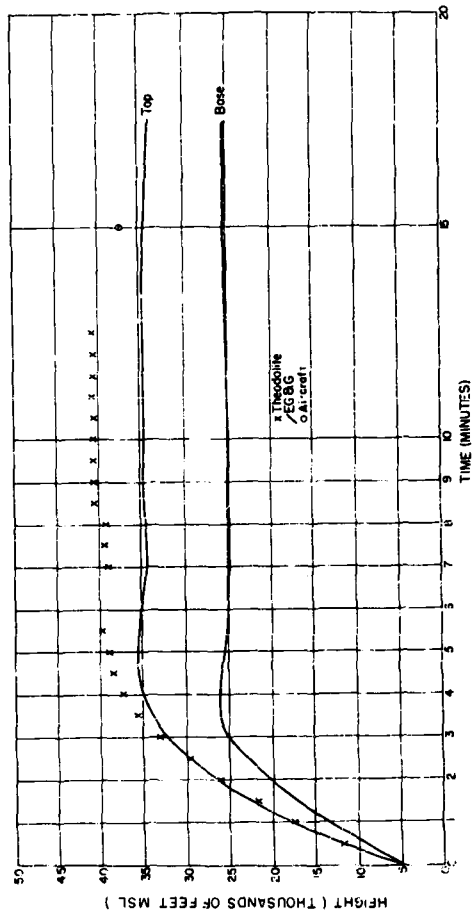
Fig. 3.16 Cloud Base vs Time, Shot 14
