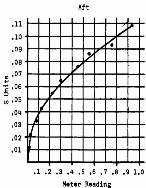
Figure 10. Calibration Curve for 2/rev. Channel, Unit 97V1003.
