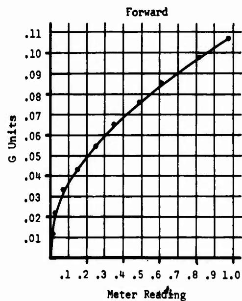
Figure 10. Calibration Curve for 2/rev. Channel, Unit 97V1003.
