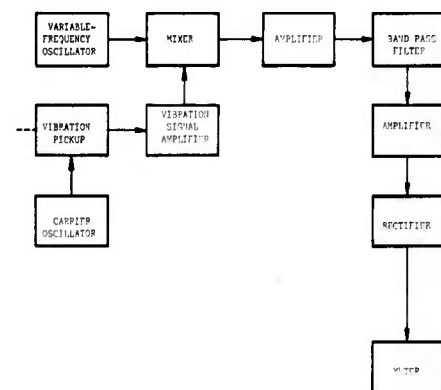
Figure 5. Spectrum Analyzer
