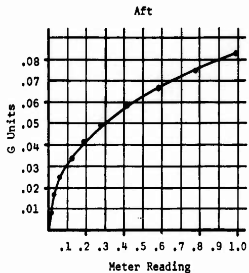
Figure 9. Calibration Curve for 1/rev. Channel, Unit 97V1003.
