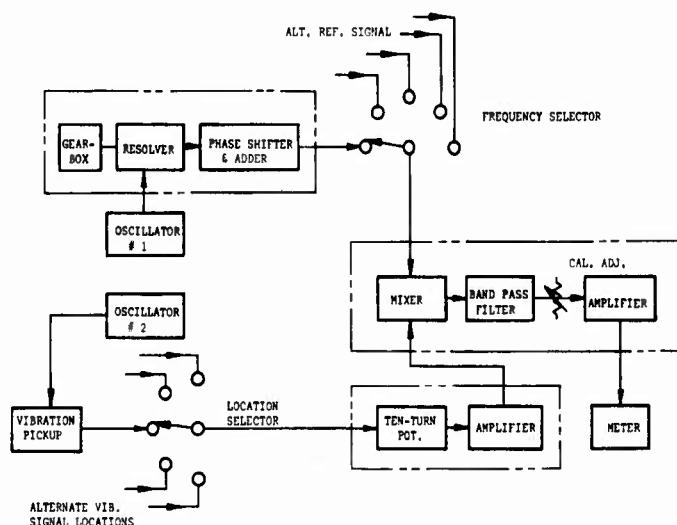
Figure 2. Fixed-Frequency System
