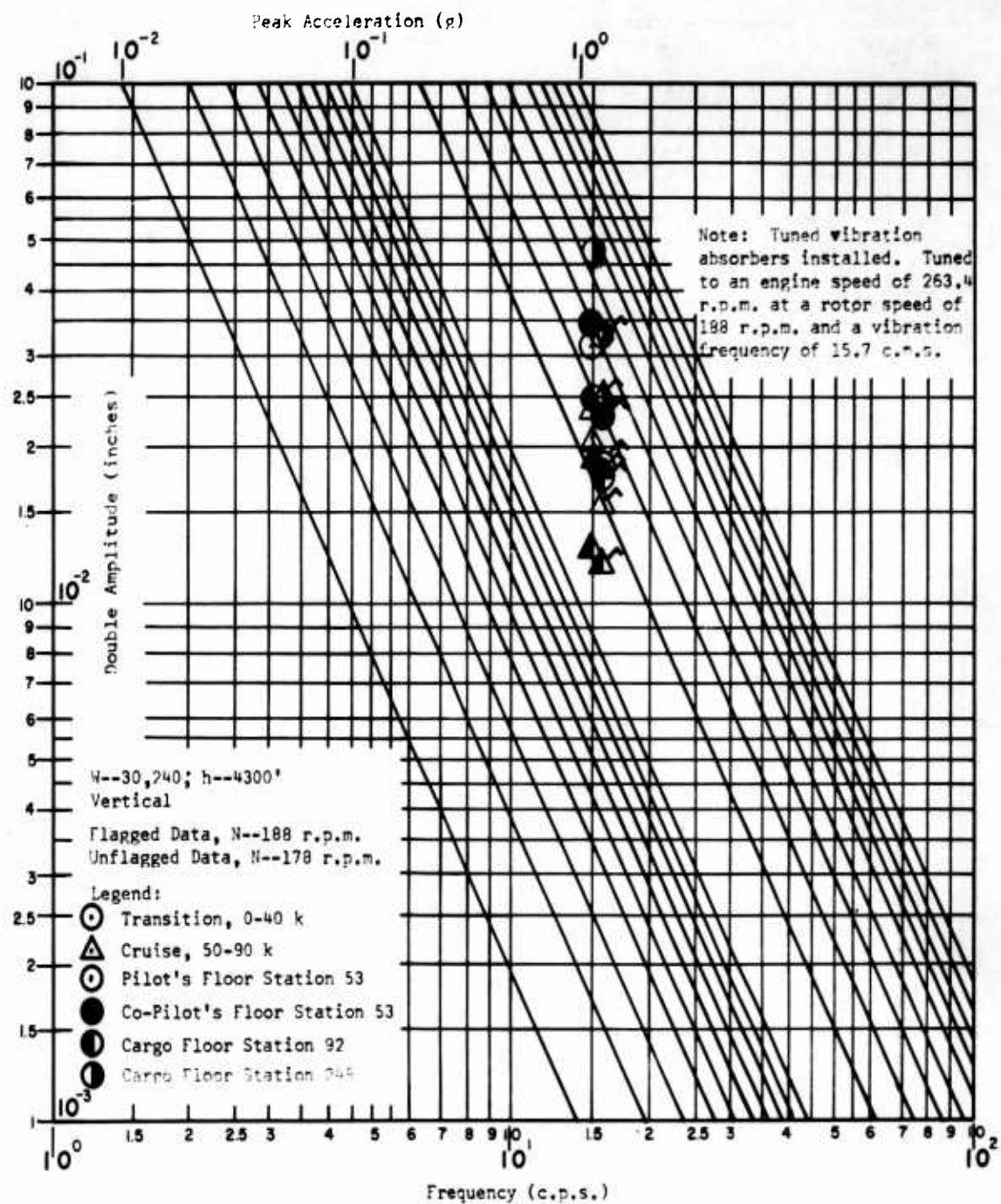
Figure 8a. Vibration Data for the Model H-37A Sikorsky.
