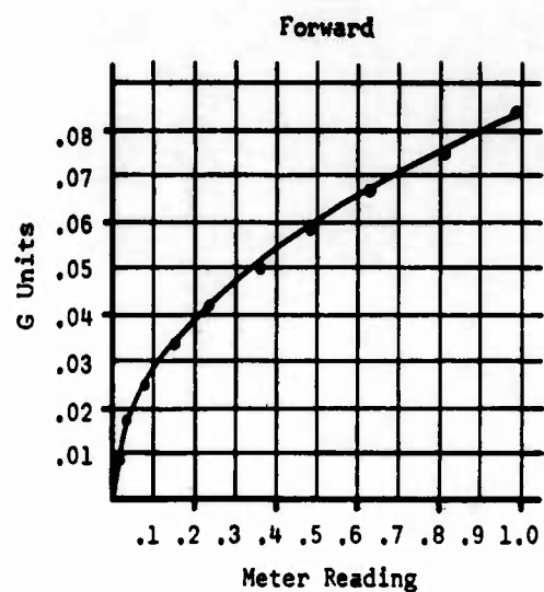
Figure 9. Calibration Curve for 1/rev. Channel, Unit 97V1003.
