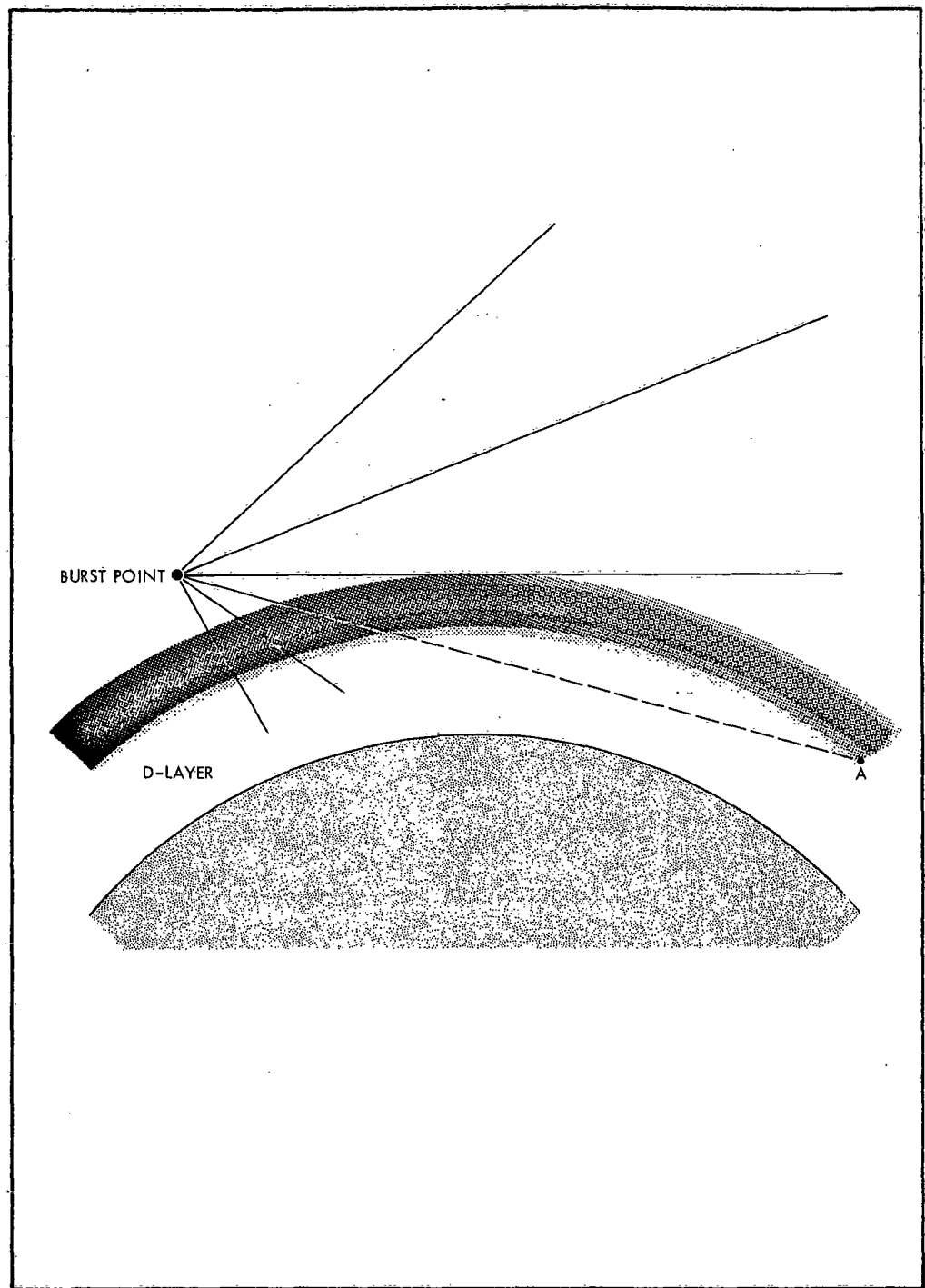
Figure 4-1. Effect of Earth Curvature on Neutron Range
