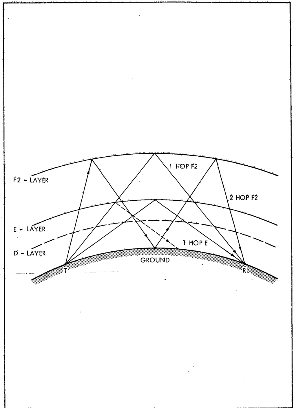
Figure 3-4. Ionospheric Sky-Wave Propagation
