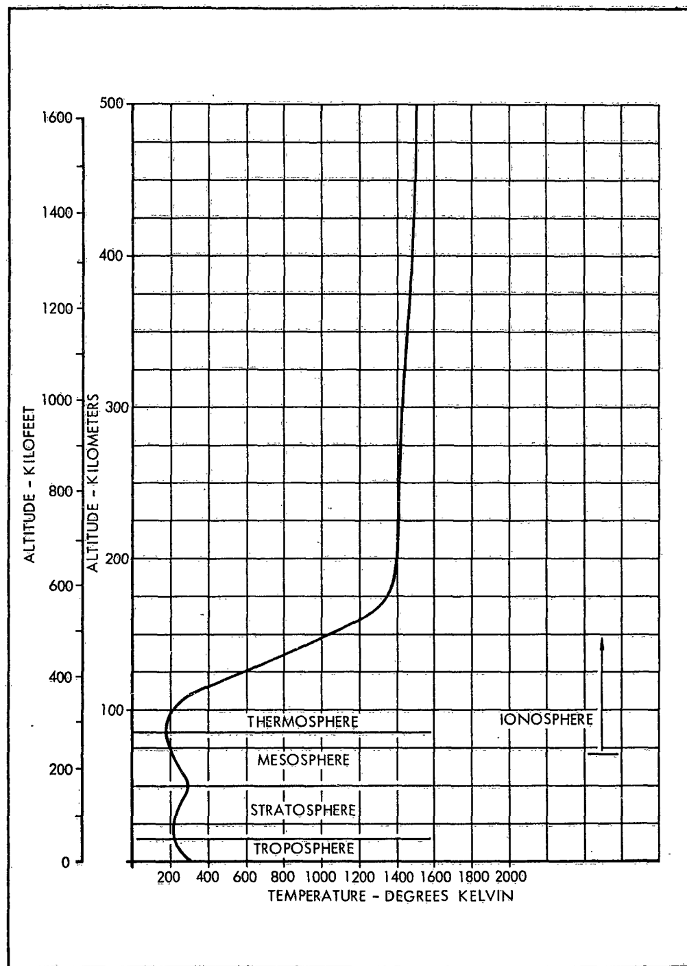
Figure 2-5. Atmosphere Temperature
