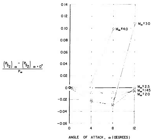
FIGURE 17(B) ANGLE OF ATTACK PERFORMANCE OF S_2 STATIC PORTS ON SURVEY MODEL S-104. EXPERIMENTAL DATA: (AECC E-1 SUPERSONIC WIND TUNNEL)
