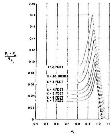
FIGURE 4 STATIC PRESSURE ERROR AHEAD OF XB-70 AS A FUNCTION OF INOKATED MACH NUMBER (NAA ESTIMATE)
