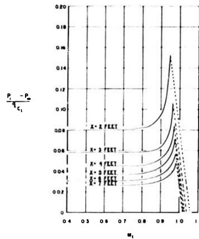
FIGURE 3 STATIC PRESSURE ERROR AHEAD OF XB-70 AS A FUNCTION OF INOKATED MACH NUMBER (REC ESTIMATE)
