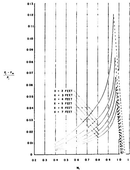
FIGURE 5 STATIC PRESSURE ERROR AHEAD OF XB-70 AS A FUNCTION OF INOKATED MACH NUMBER (REC ESTIMATE)
