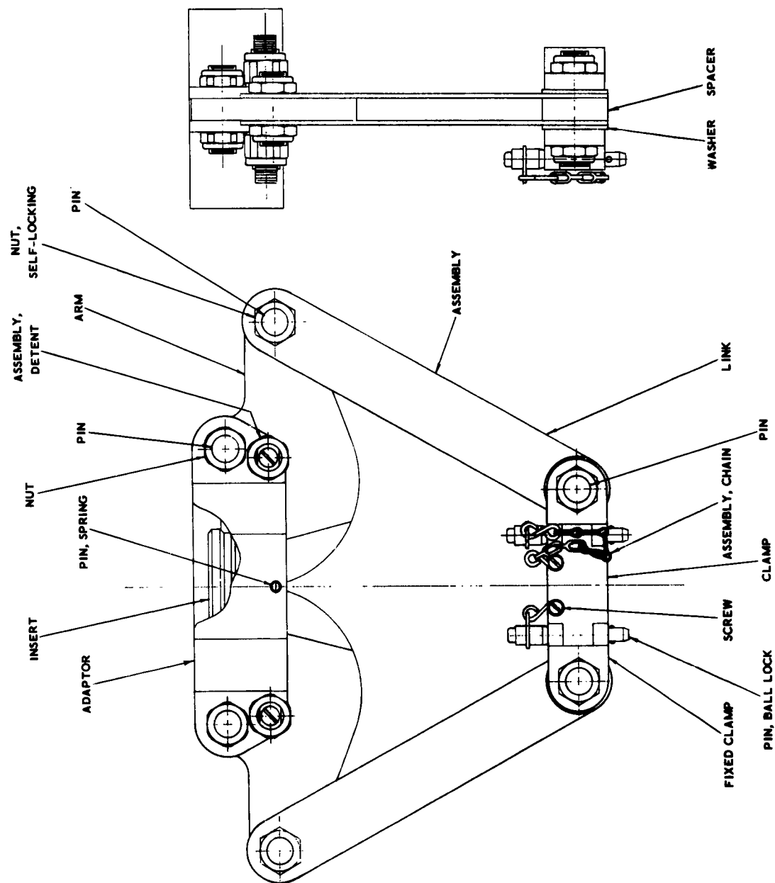
Assembly Drawing of Retrieve Device
