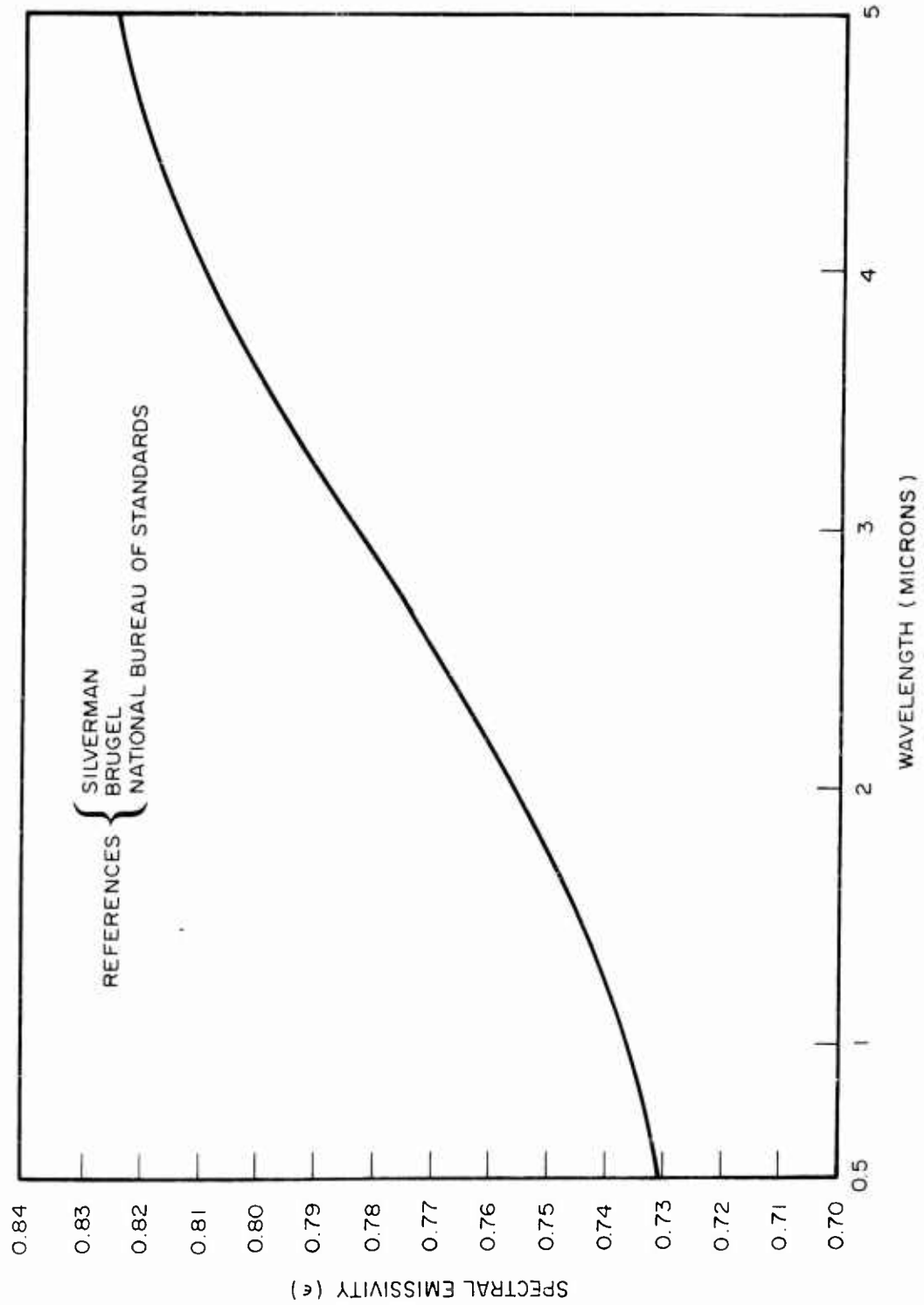
Fig. 2-9 Global Emissivity
