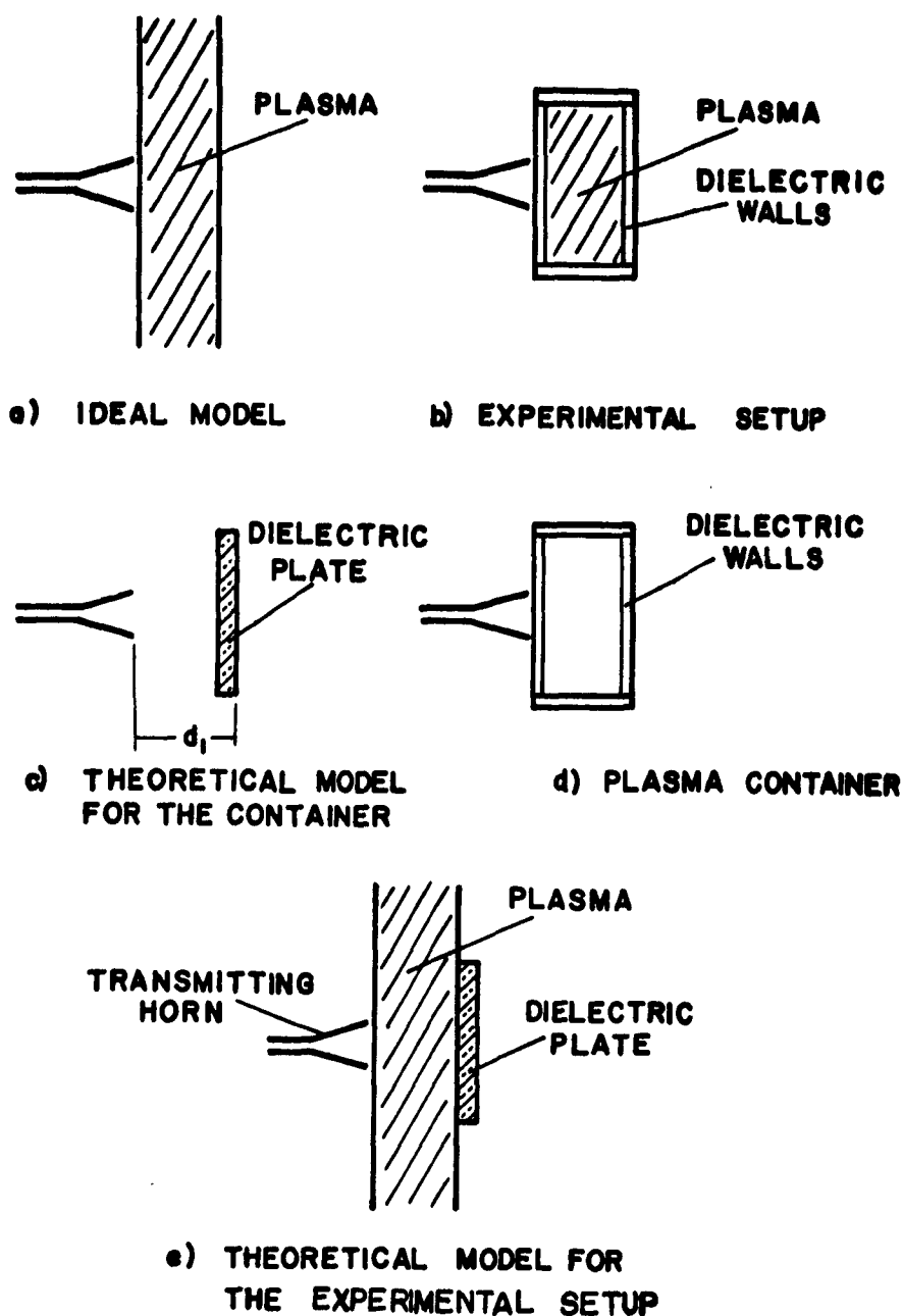
Fig. 8: Schematic diagrams of the various models used in the interpretation of the measurements.
