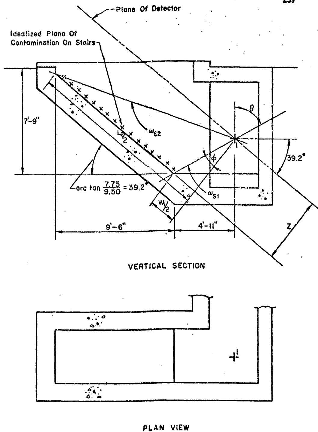
FIG. 9.09 GROUND DIRECT CONTRIBUITON AT POINT 1 FROM STAIRS.
