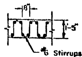
Section B-B (Stirrup Detail Shown)
