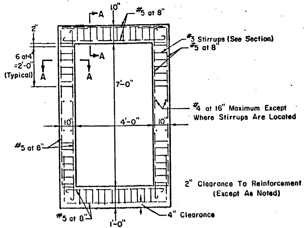
Transverse Section
