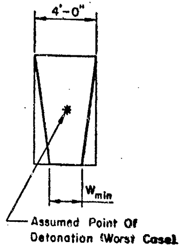
OPENING AS VIEWED FROM POINT 1
