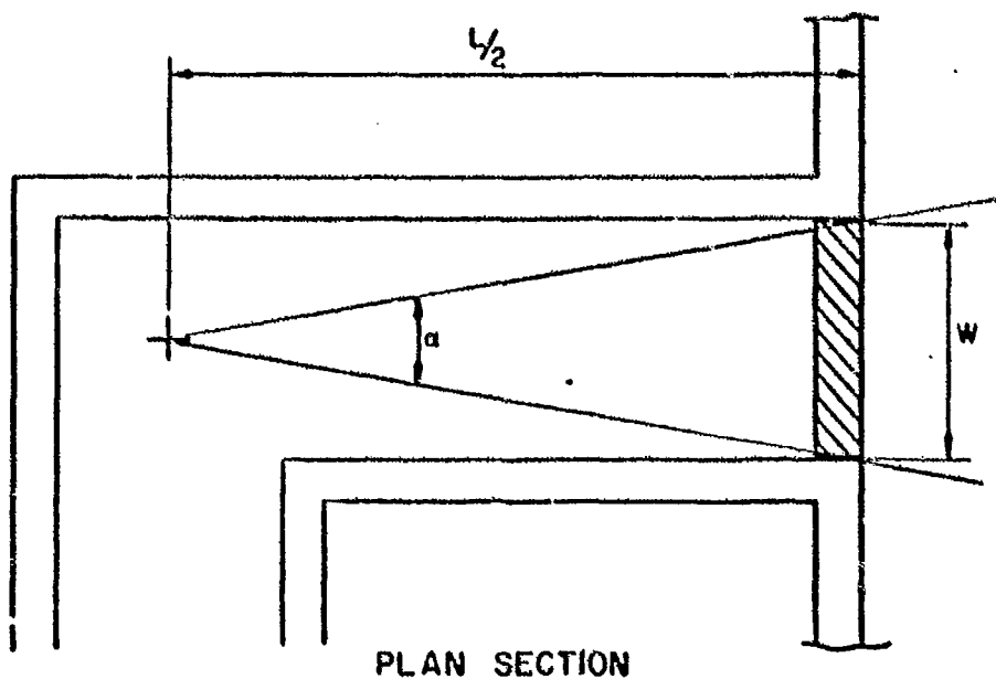
FIG. 6.02 CONTRIBUTION THROUGH VERTICAL EXTERIOR BARRIER (POINT OF INTEREST ABOVE PLANE OF CONTAMINATION OUTSIDE)
