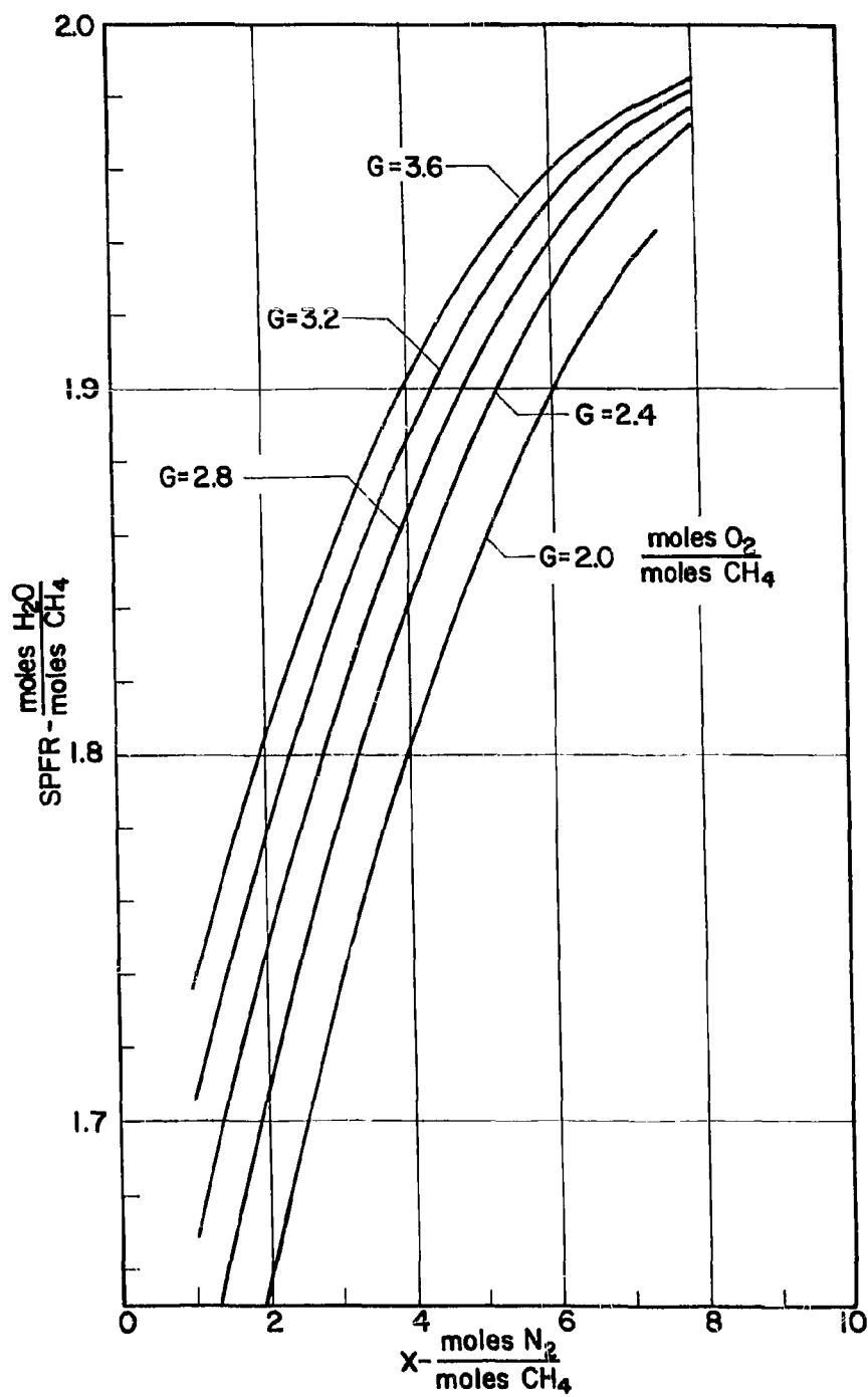
FIGURE 40-SPFR OF H_2O vs. \frac{\text{moles } N_2}{\text{moles } CH_4}
