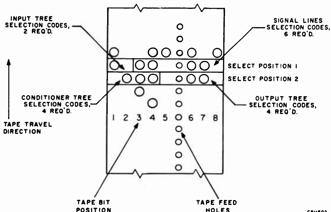
FIGURE 9. PROGRAM TAPE CODING, SIGNAL SELECTION RELAY SECTION
