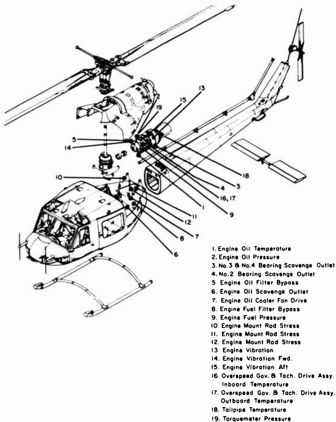
FIGURE 2. PACER SENSOR LOCATION, POWER PLANT
