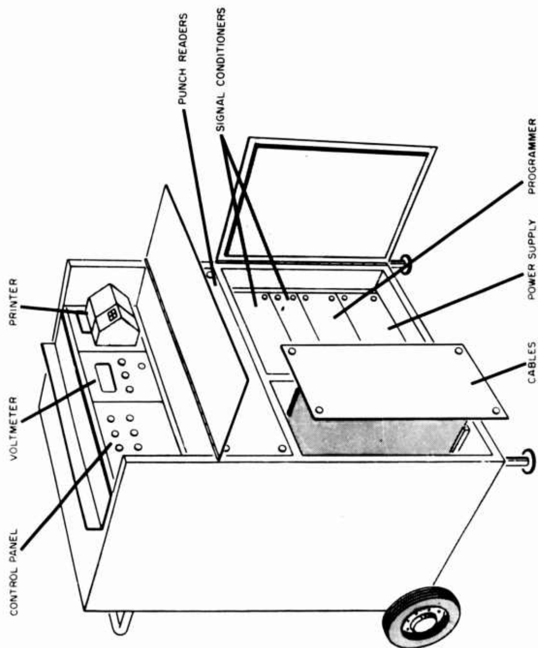
FIGURE 6. PACER CABINET
