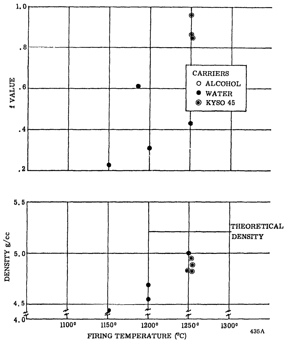
Figure 5. Density and alignment index for \text{Ni}_{1.0}\text{Zn}_{1.0}\text{Y} samples plotted as a function of firing temperature. Data are shown for two different carriers used in the attriting process.
