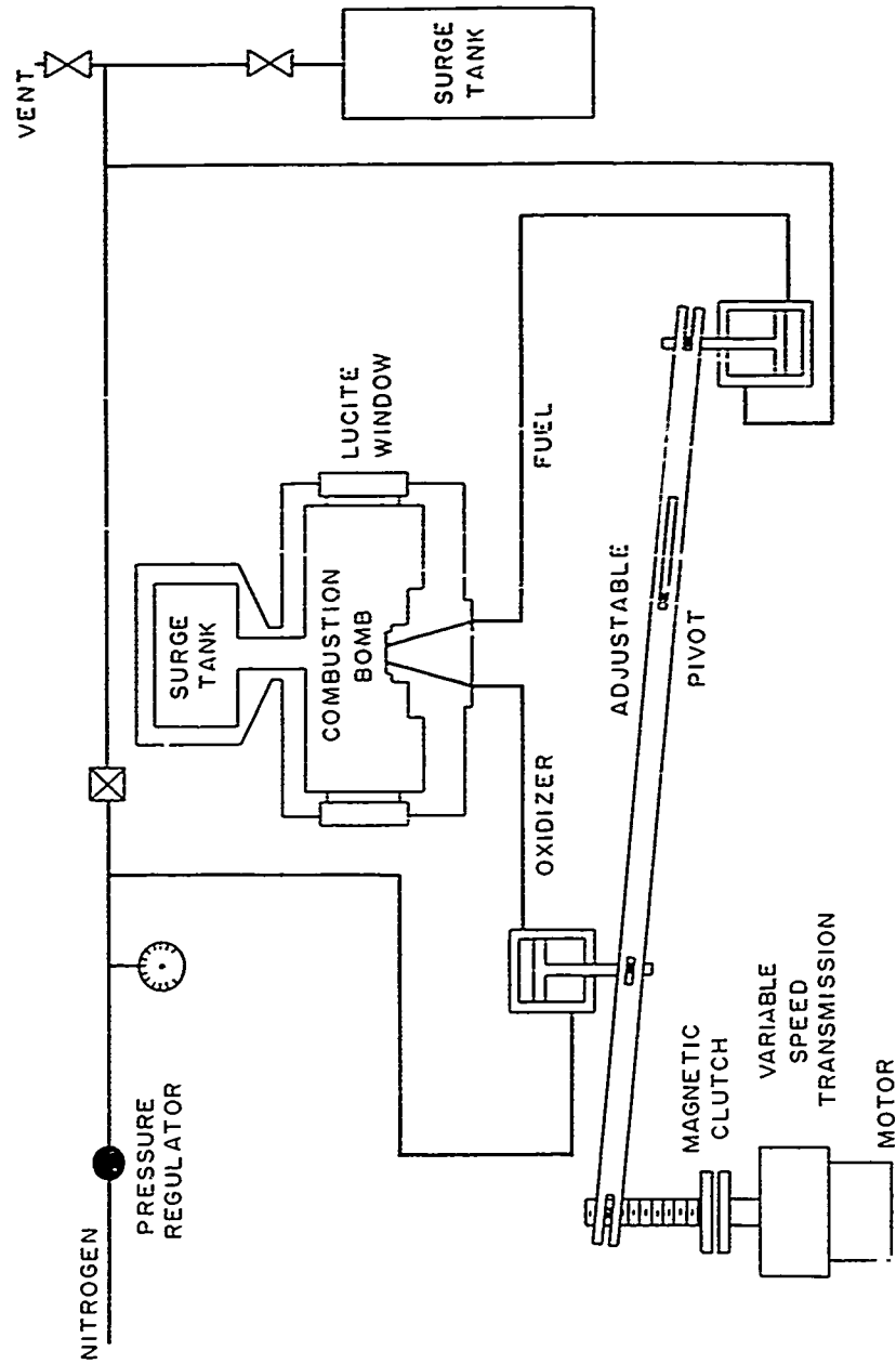
FIG. 18. Micromix Schematic Diagram.
