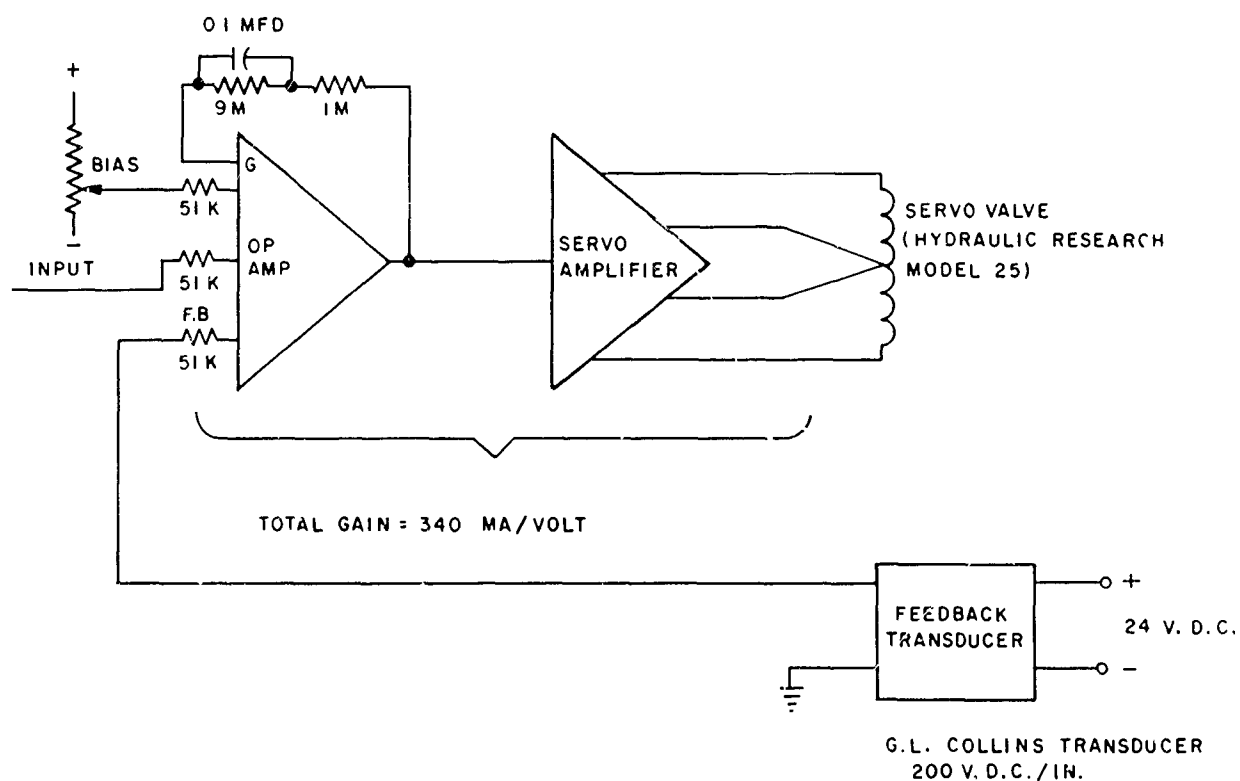
FIG. 43. Preliminary Servo Electronic Schematic Used in Servo Laboratory.
