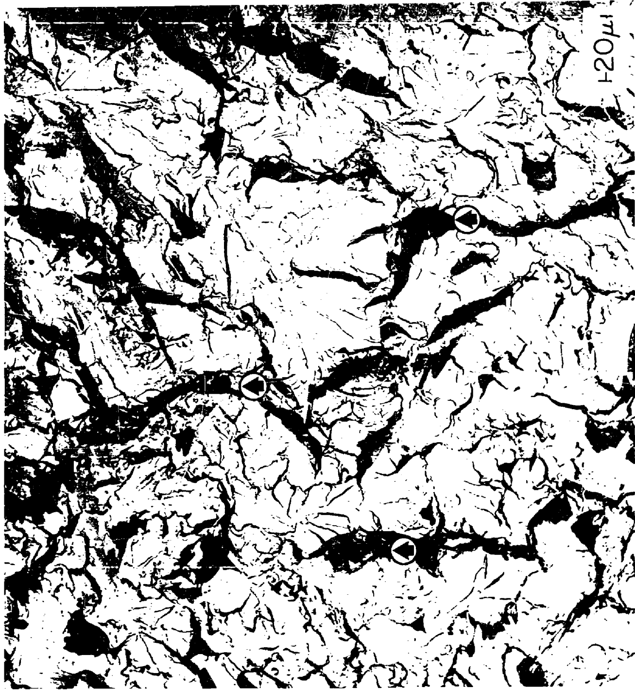
Fig. 11 - Collapsed carbon films (arrows) on replica of cleavage fracture in mild steel
