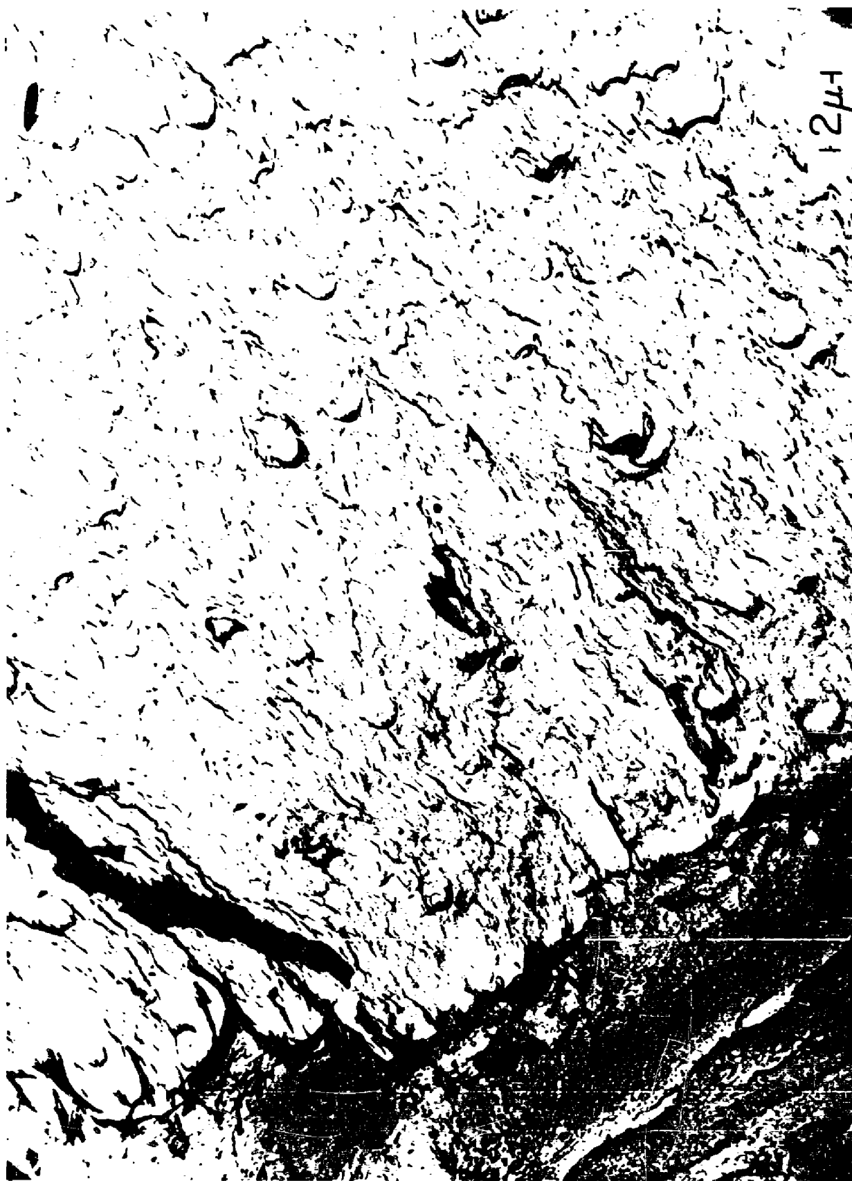
Fig. 6 - Surface structure of a tear in plastic of the first-stage replica
