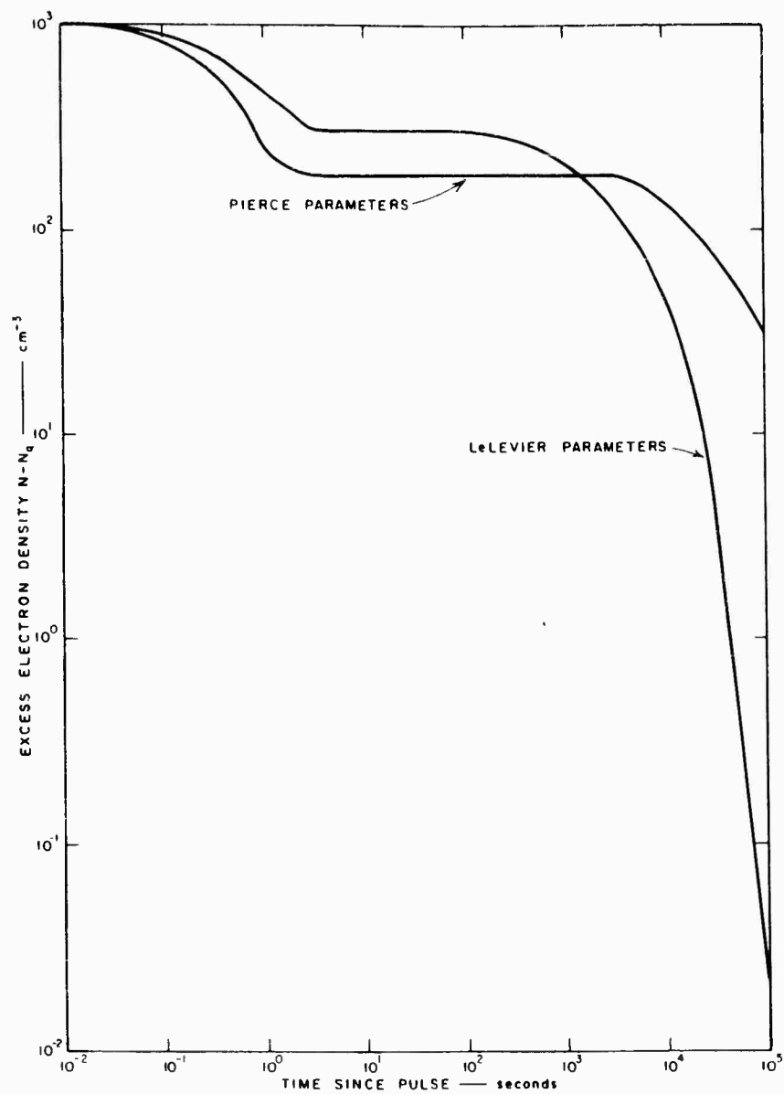
FIG. 1.3 EXCESS ELECTRON DENSITY vs. TIME AFTER DEPOSITION OF 10^3 ELECTRONS/ \text{cm}^3
