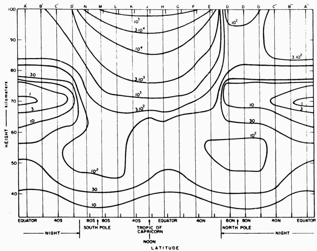
FIG. 4.8 MERIDIONAL PATH AT WINTER SOLSTICE CONSIDERING NONEQUILIBRIUM AT NIGHT — ELECTRON DENSITY CONTOURS ( \text{cm}^{-3} )
