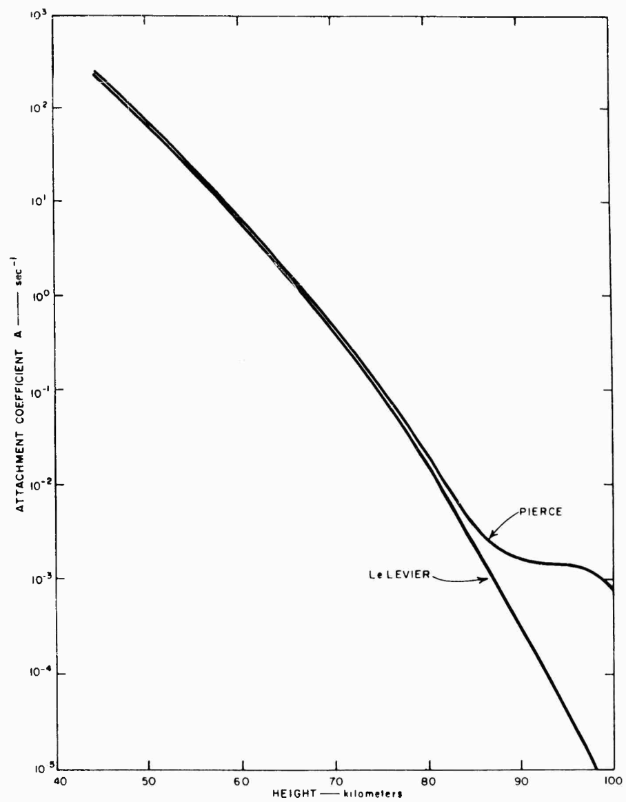
FIG. 1.1 COMPARISON OF VALUES OF PIERCE AND LE VIEUR FOR THE ATTACHMENT COEFFICIENT
