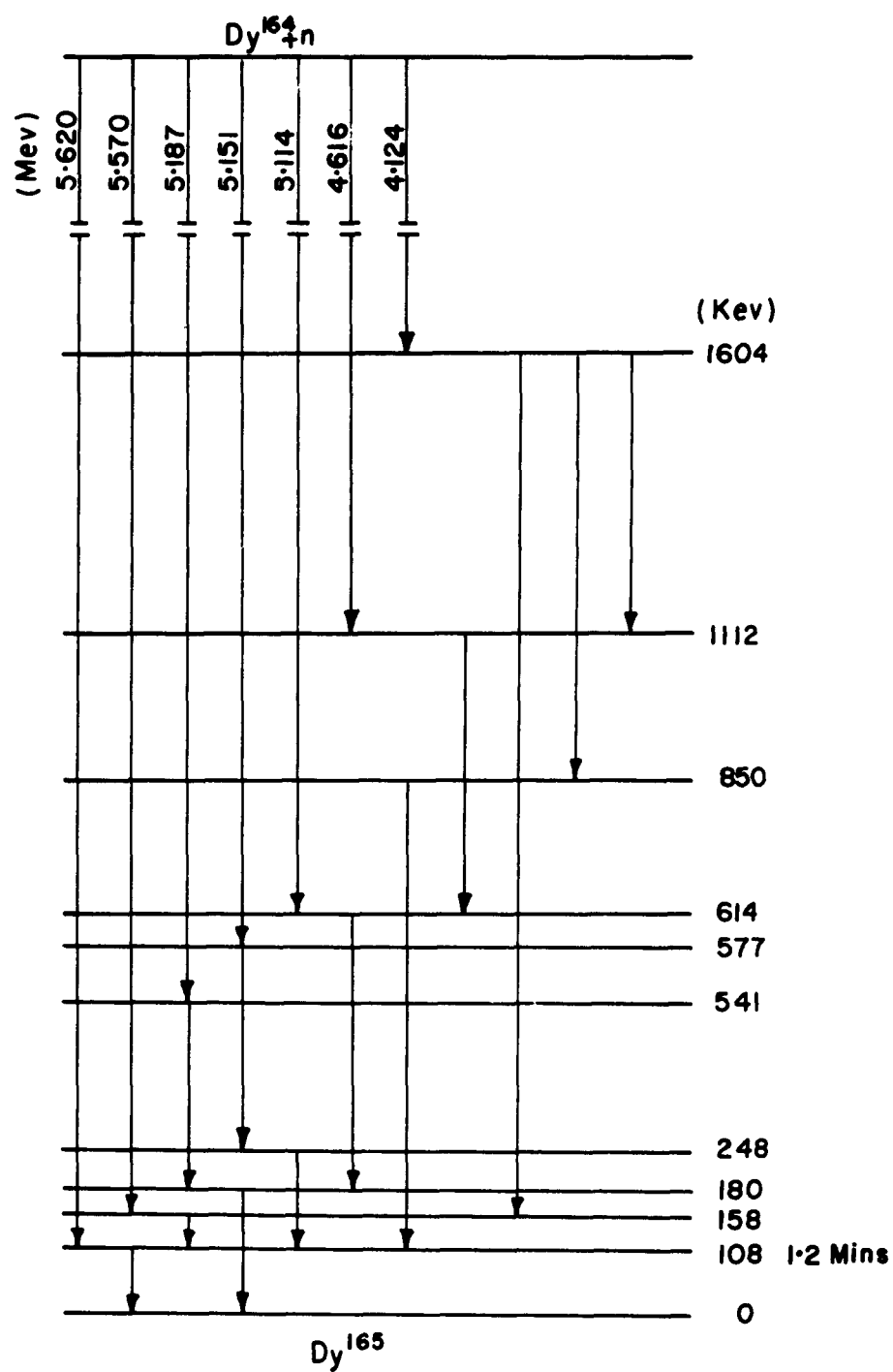
FIG 34. TENTATIVE NUCLEAR ENERGY LEVEL SCHEME OF \text{Dy}^{165} SUGGESTED BY THE COINCIDENCE DATA
