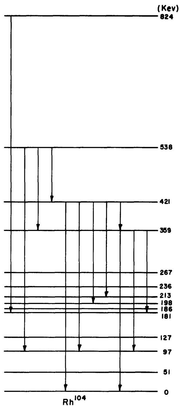
FIG 31. SUGGESTED ADDITIONS TO THE \text{Rh}^{104} NUCLEAR ENERGY LEVEL SCHEME OF BUSCHHORN BI
