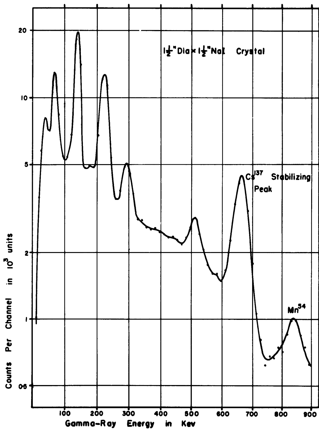
FIG 10. CAPTURE GAMMA-RAY SPECTRUM OF \text{Sc}^{48}
