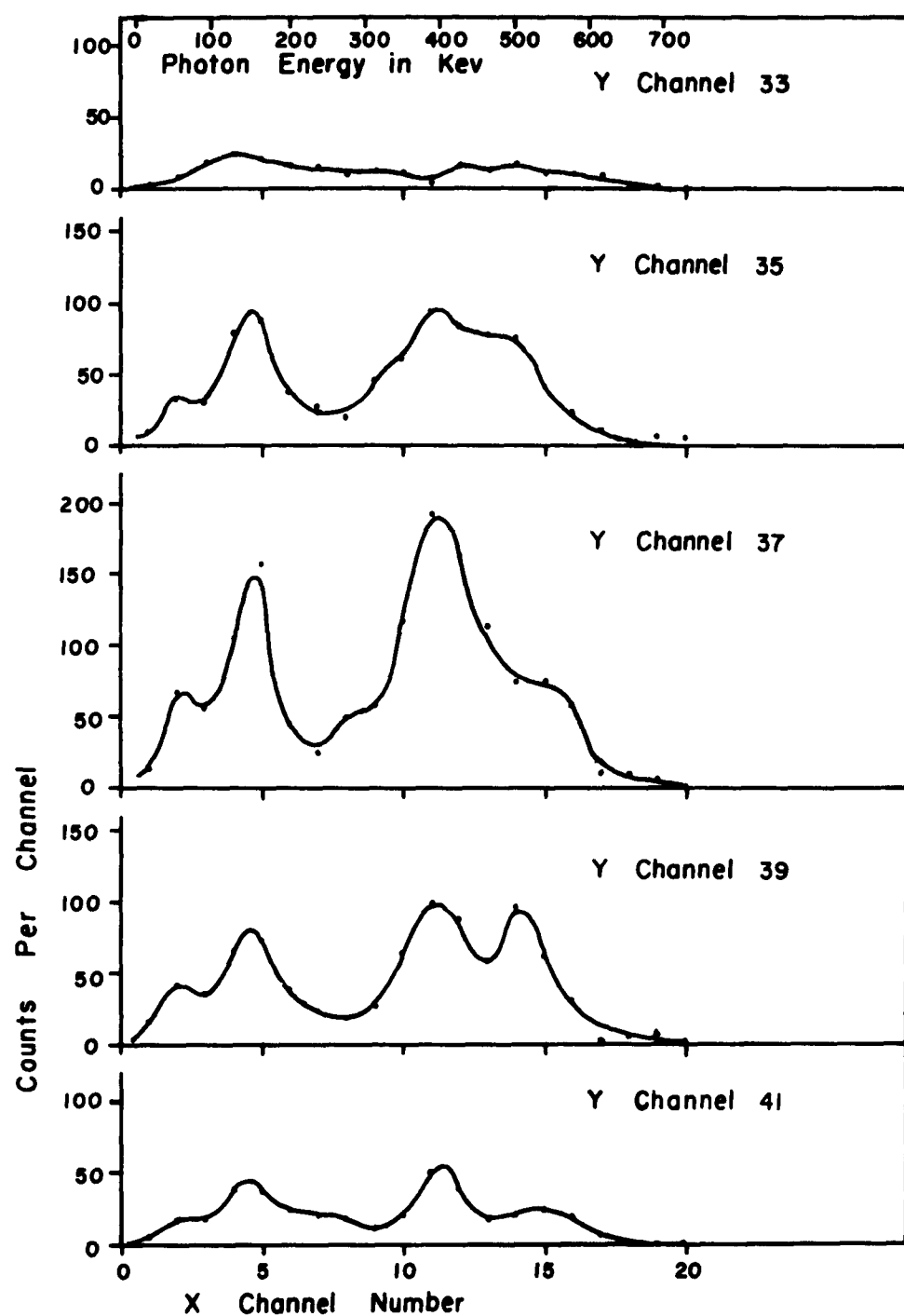
FIG 23. LOW ENERGY GAMMA RAYS IN COINCIDENCE WITH THE 5.15 MEV GAMMA-RAY GROUP FROM IRRADIATED \text{Dy}^{164}
