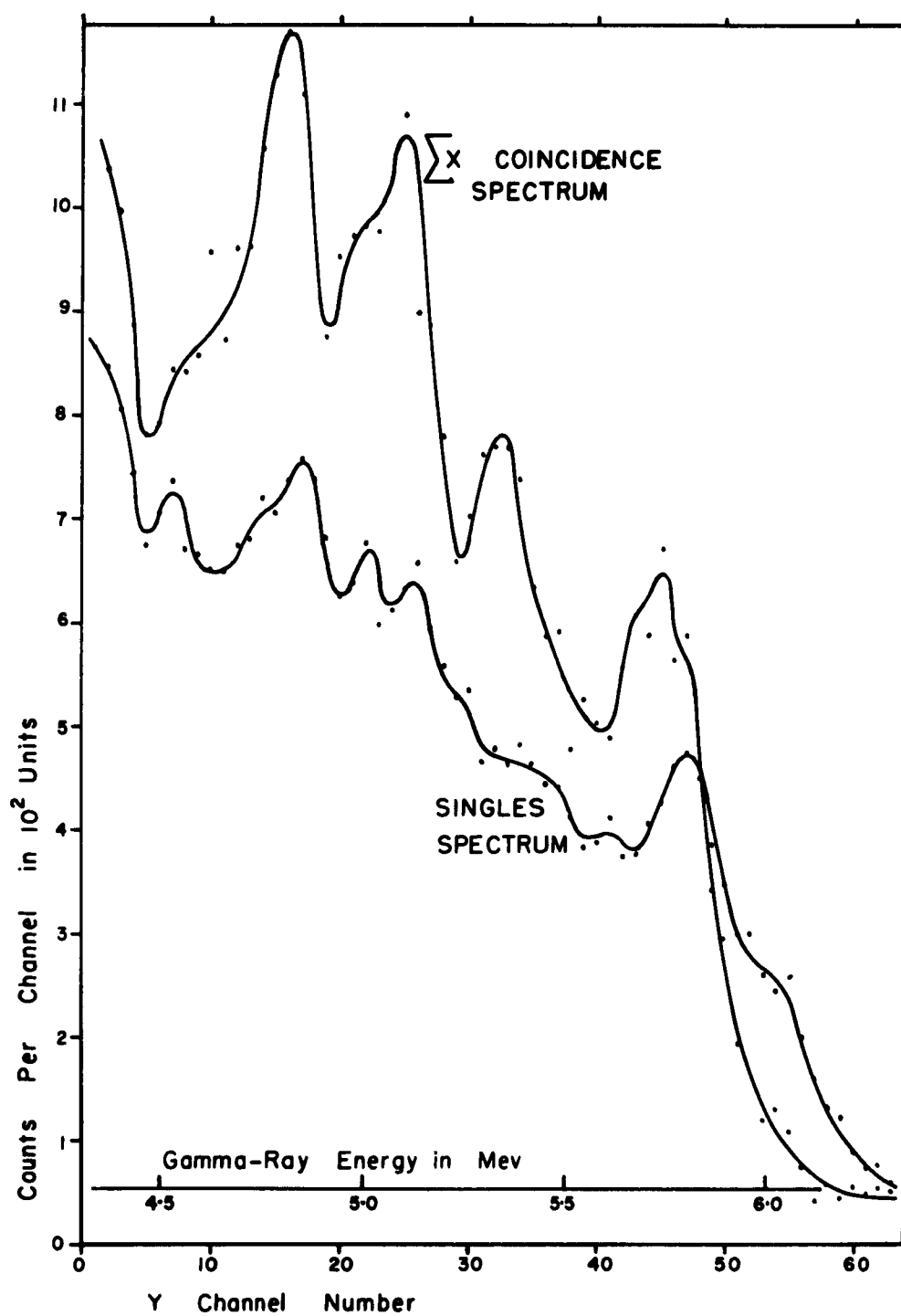
FIG 24. SINGLES AND COINCIDENT PAIR SPECTRA FROM IRRADIATED \text{Ho}^{165}
