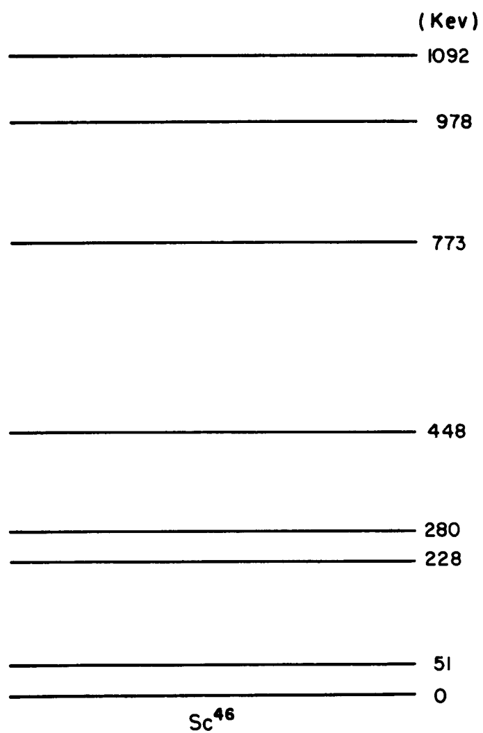
FIG 26. NUCLEAR ENERGY LEVELS OF \text{Sc}^{46} MEASURED BY MAZARI M2
