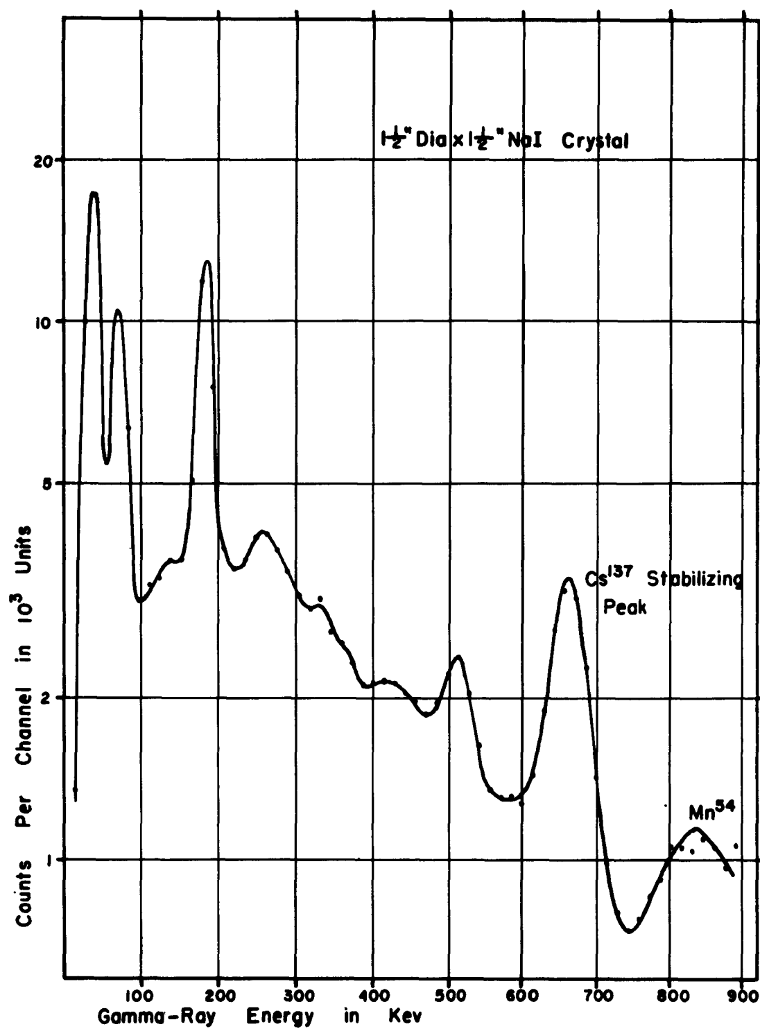
FIG 12. CAPTURE GAMMA-RAY SPECTRUM OF \text{Dy}^{161}
