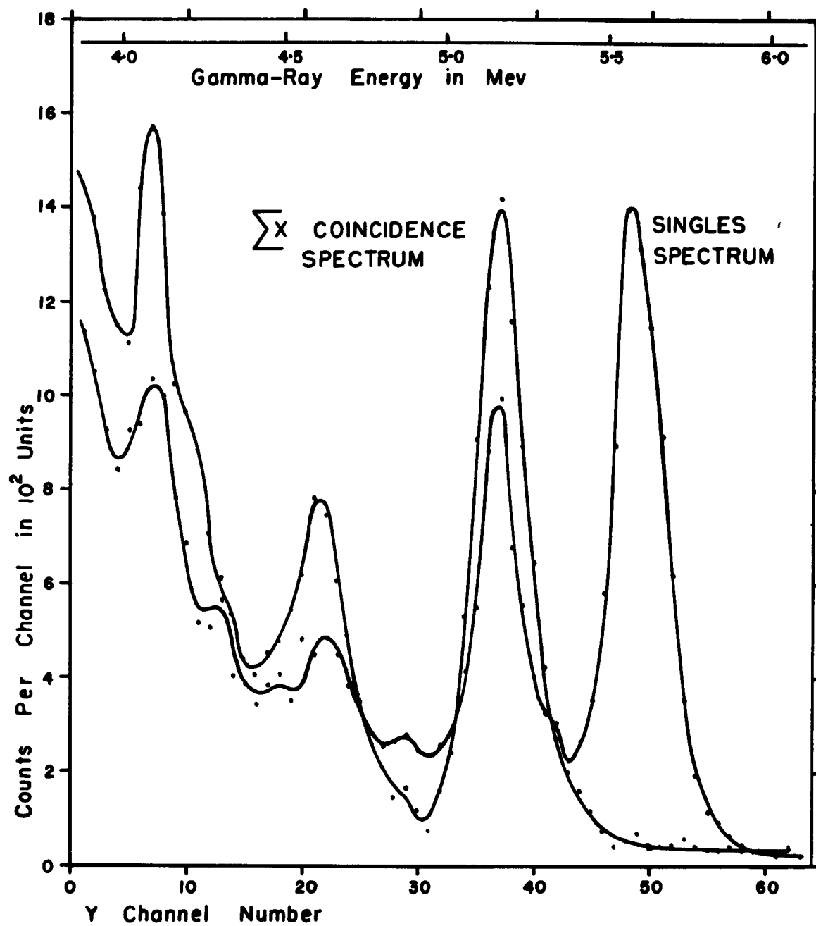
FIG 22. SINGLES AND COINCIDENCE PAIR SPECTRA FROM IRRADIATED Dy 164
