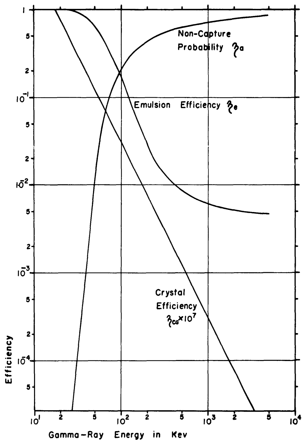
FIG 4. COMPONENT EFFICIENCIES OF THE BENT CRYSTAL SPECTROMETER SYSTEM
