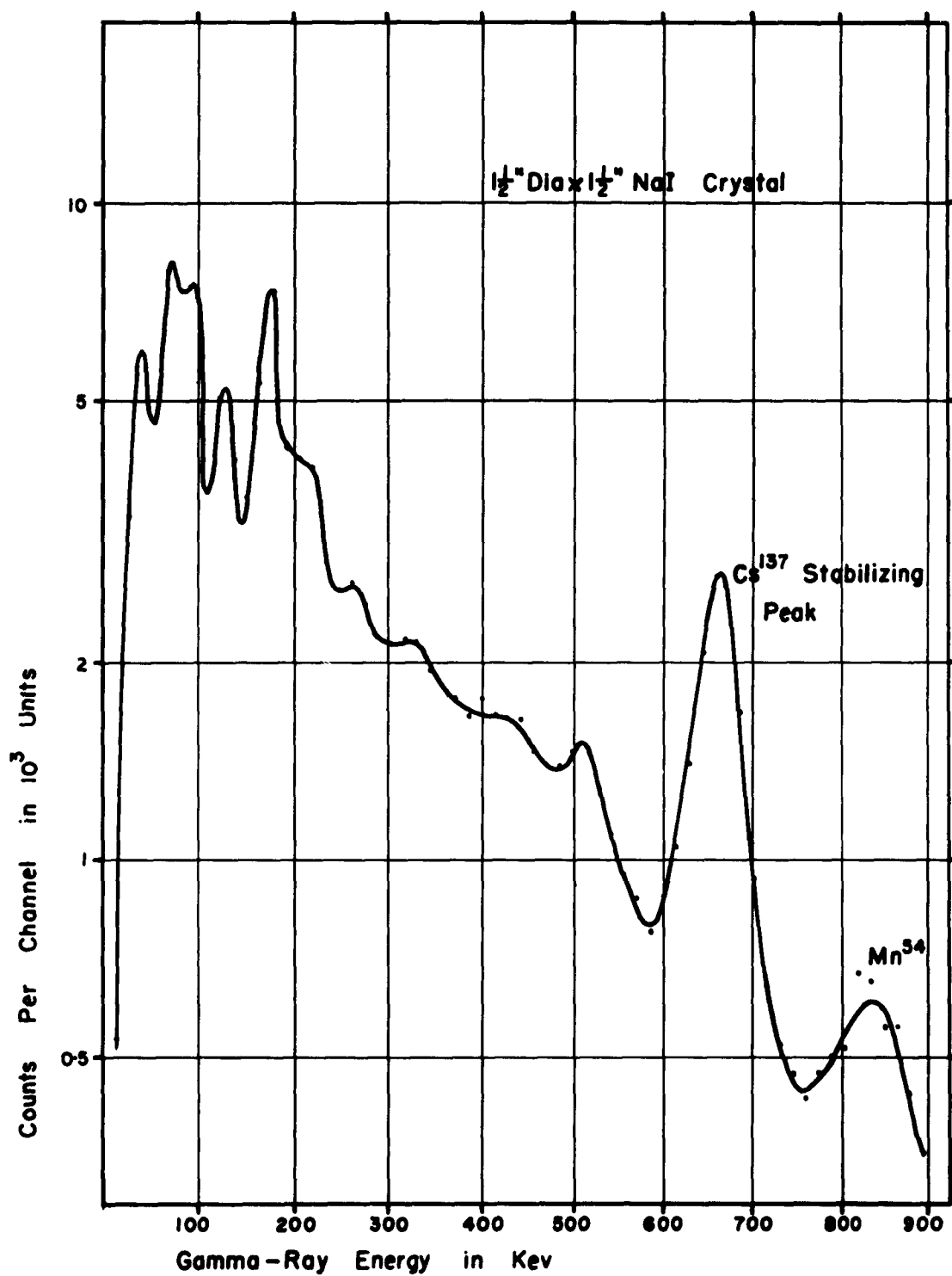
FIG 11. CAPTURE GAMMA-RAY SPECTRUM OF \text{Rh}^{103}
