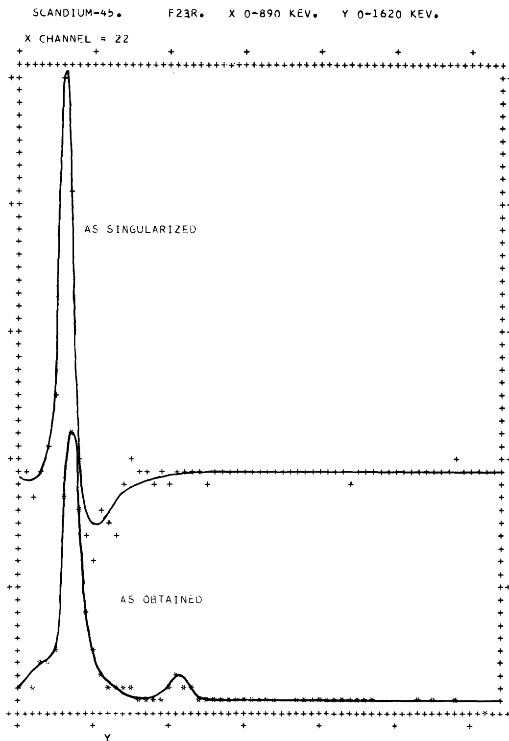
Fig. 43. Twofold coincidence gamma-ray spectra, as obtained and as singularized.
