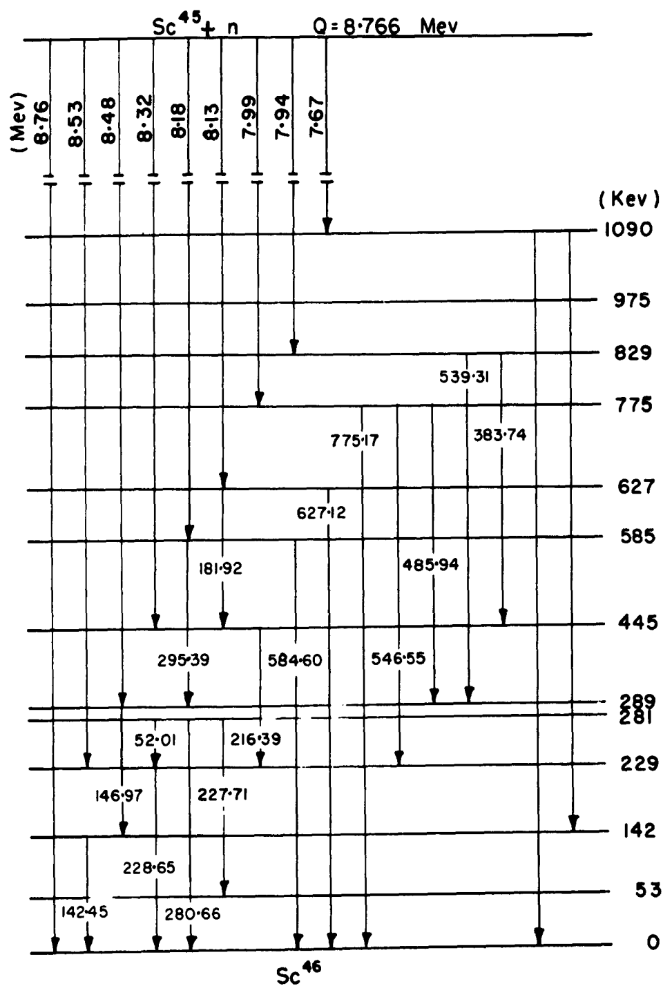
FIG 28. FINAL PROPOSED NUCLEAR ENERGY LEVEL SCHEME OF \text{Sc}^{46}
