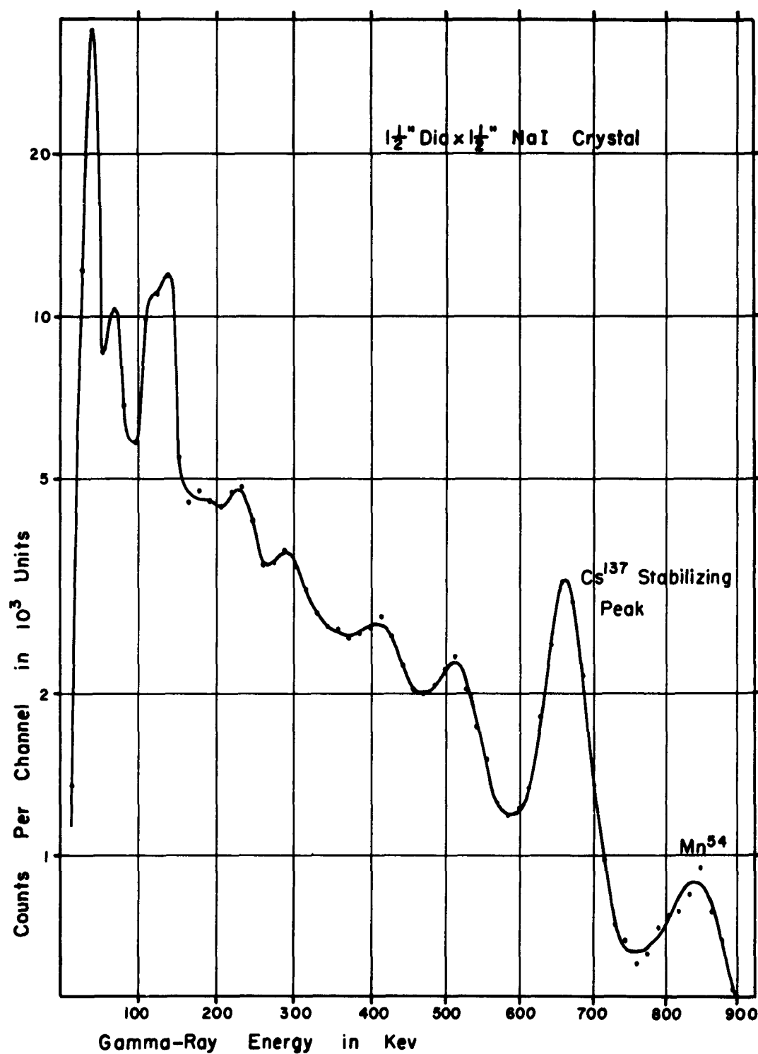
FIG 14. CAPTURE GAMMA - RAY SPECTRUM OF \text{Ho}^{165}
