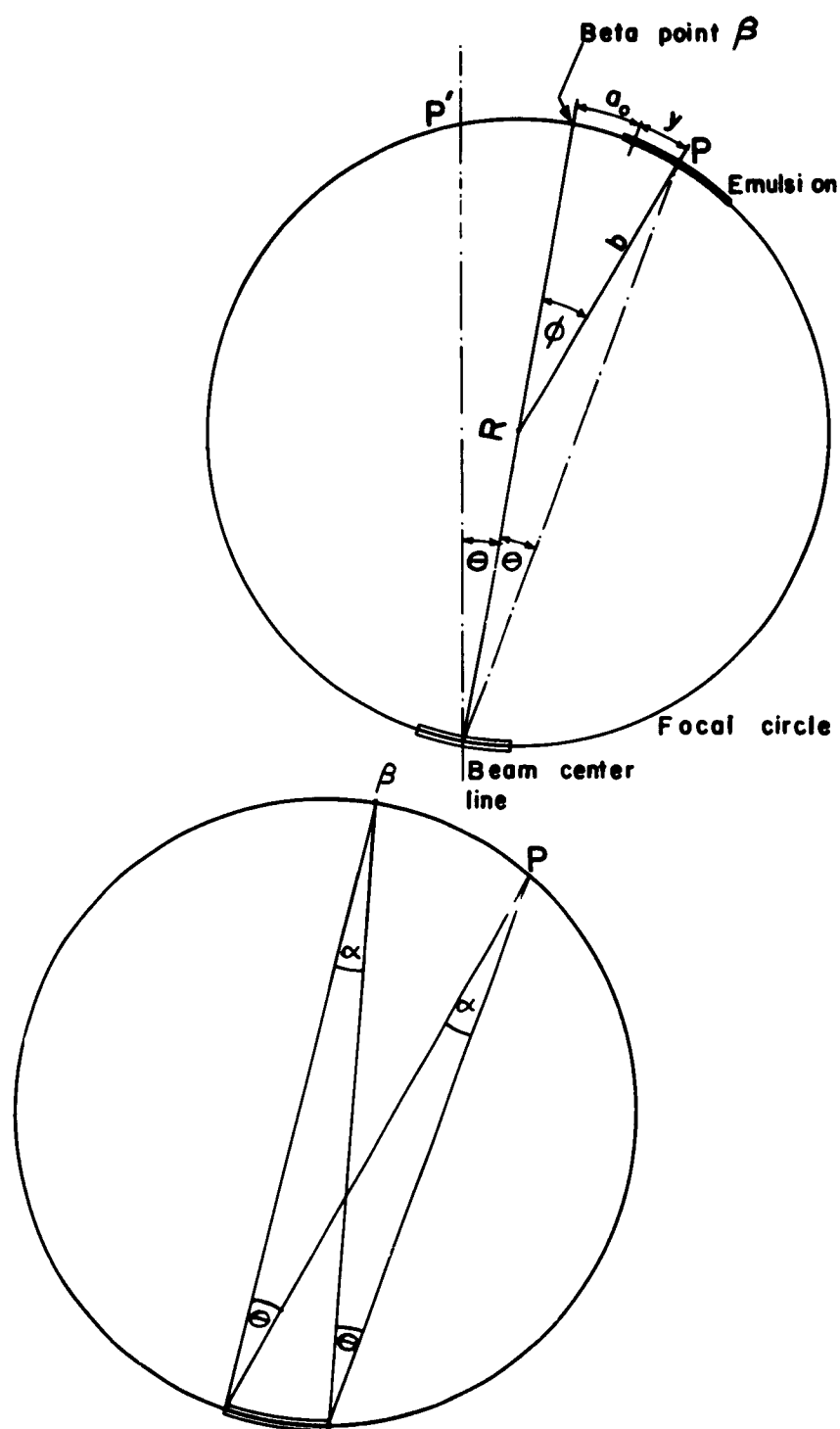
FIG 40. BENT CRYSTAL GEOMETRY
