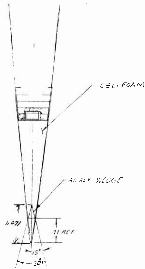
Figure 22 Drawing of 173 Inch 240 Slot Blade Antenna
