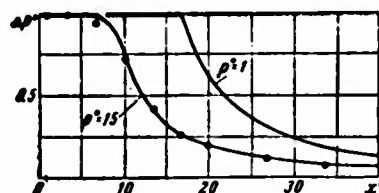
Figure 6. Change in the velocity head \Delta p^0 = \rho_m u_m^2 / \rho_0 u_0^2 along the axis of jets of heated ( \rho^0 = 15 ) and isothermic ( \rho^0 = 1 ) air; curves, by calculation; points, by tests with \rho^0 = 15
