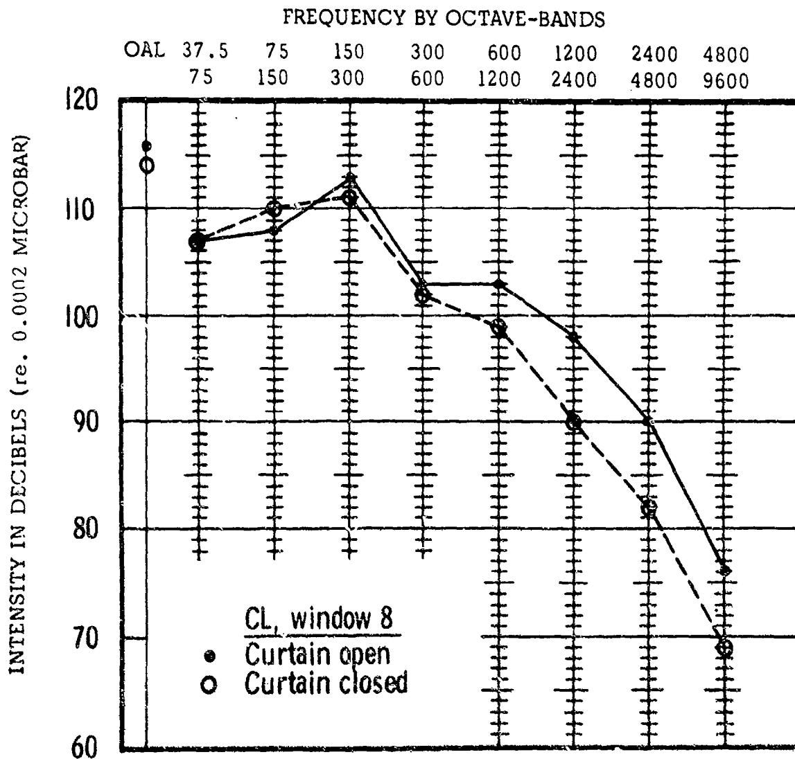
Fig. 92 Internal Noise of CV-2B Aircraft During Normal Cruise at 5500' Altitude, 2000 RPM, 32" MP, 140 Knots IAS
