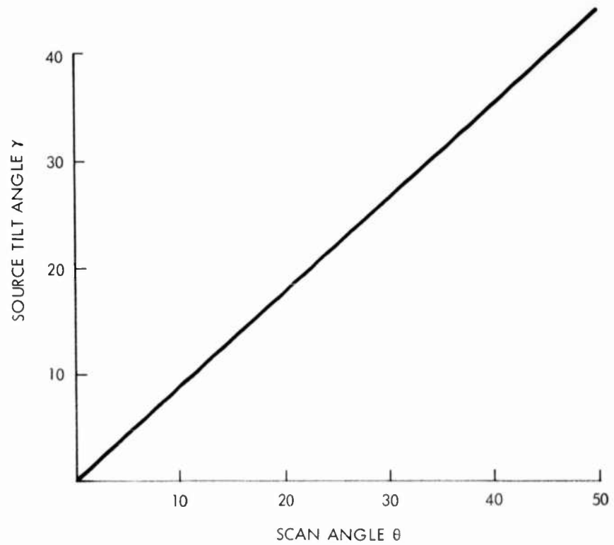
Figure 5-1. Variation of Source Tilt Angle with Scan Angle
