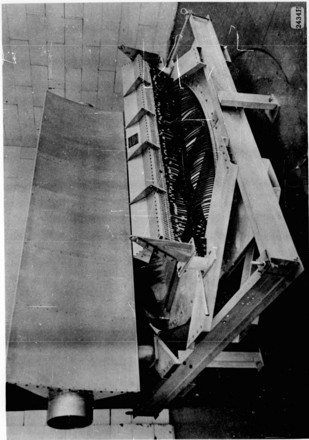
Figure 9-2. Front View of Completed MUBIS Antenna System
