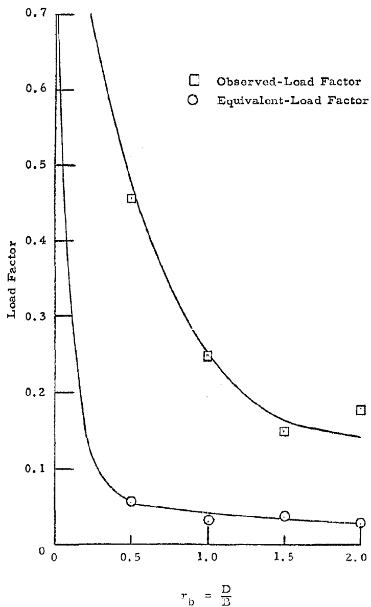
Fig. A-17 LOAD FACTORS AS RELATED TO BURIAL RATIO, TWO-DIMENSIONAL STATIC TESTS, CLAY, f_{\Delta} = 0.050
