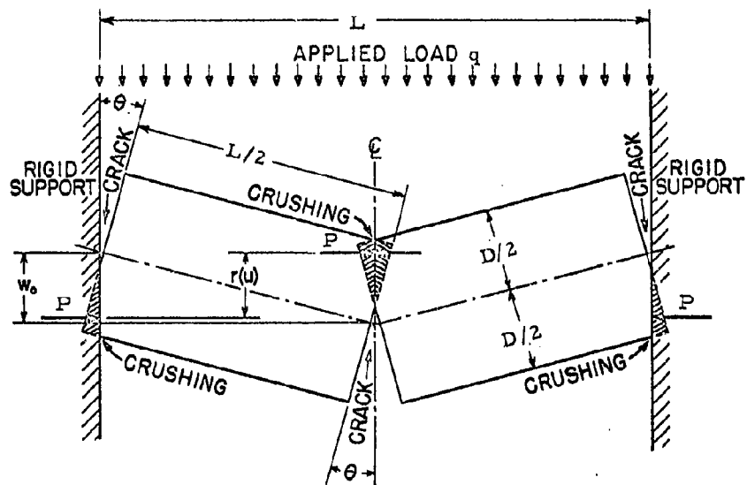
(a) Plan View of Wall in Deflected Position
