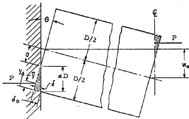
(b) Geometry at Support
