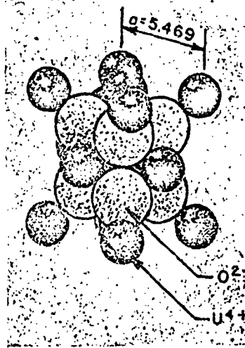
Figure 79. Elementary \text{UO}_2 cell
